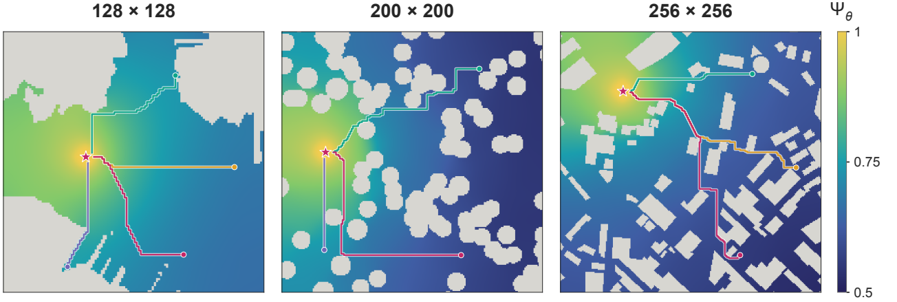
Fig. 4: Zero-shot FNO field predictions and extracted paths at 128 \times 128 , 200 \times 200 , and 256 \times 256 (left to right). Color shows predicted desirability \Psi_\theta , gray denotes obstacles, circles mark starts, and the star marks the shared goal in each map.
