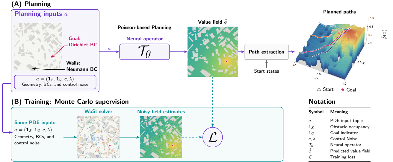
Fig. 2: Planning Under Noise: (A) Planning: a neural operator maps geometry, goal, cost, and noise inputs to a desirability field. Grid-based local search selects feasible routes with high endpoint desirability, executes a short prefix, and replans. (B) Training: Walk-on-Stars (WoSt) estimates provide pointwise supervision; neural caching supplies learned continuation at the walk horizon.
