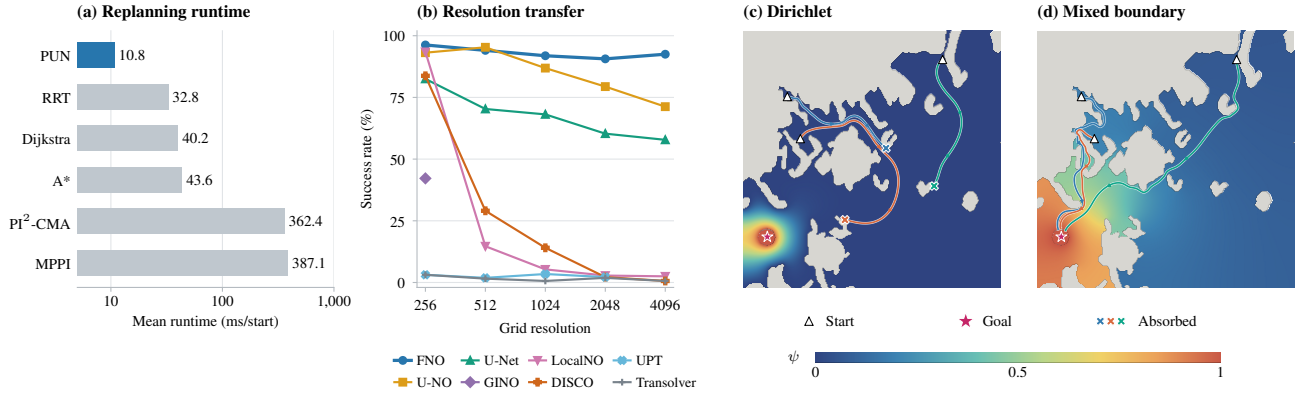
Fig. 1: (a) Fast replanning. PUN has the lowest mean runtime on unseen 4D maps: 10.8 ms/start, compared with 32.8–387.1 ms/start for the baselines. Runtimes are averaged equally over the four execution-noise levels in Table 5 and plotted on a logarithmic axis. (b) Resolution transfer. FNO maintains over 90% local-search success across all five resolutions without retraining, reaching 92.50% at 4096 \times 4096 after training at 256 \times 256 . Missing points indicate out-of-memory failures. (c, d) Continued goal seeking. In the illustrated geometry, the solution induced by the Dirichlet boundary cannot propagate goal information further since most trajectories are absorbed by obstacles. Consequently, it is more difficult for planners to find the target than with the mixed boundary condition.
