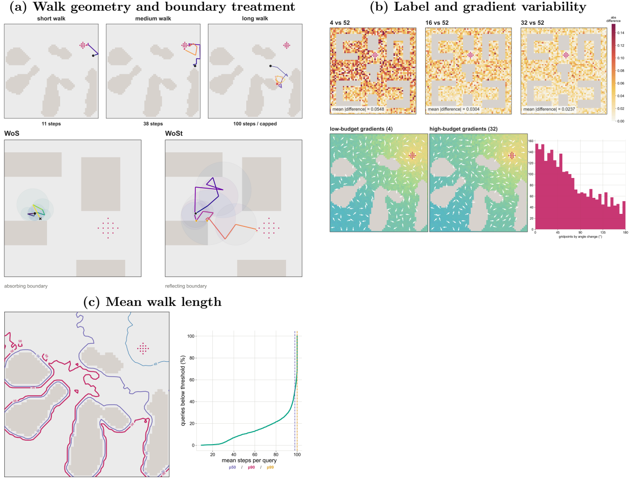
Fig. 6: WoSt walk and label statistics: (a) walk-length variability and boundary treatment; (b) label and gradient variability on a fixed map, with differences measured against a finite Monte Carlo reference; (c) spatial variation in mean walk length.
