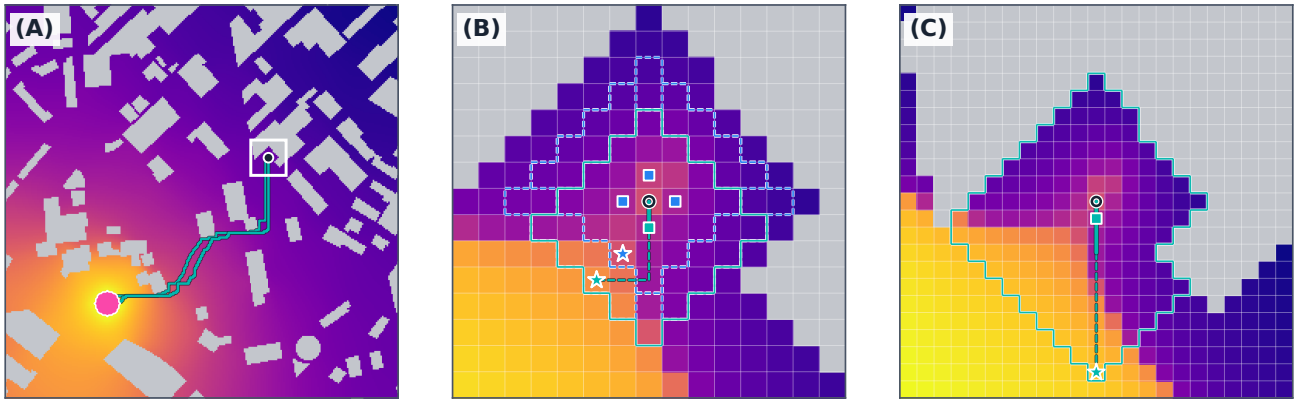
Fig. 7: Local search on one fixed urban-map field: (A) full map and routes; (B,C) enlarged neighborhoods for local search (4) and (10). Greater depth exposes endpoints farther along the passage. Gray cells are obstacles; overlays mark candidate regions and routes. Table 1 reports aggregate controller success.
