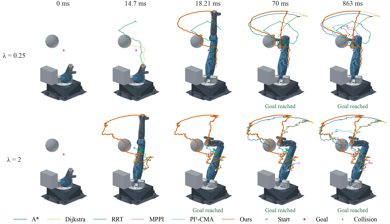
Fig. 3: Replanning trajectories on the same 4D manipulator, start, and goal at \lambda = 0.25 (top) and \lambda = 2 (bottom). Columns show successive execution states; PUN’s trajectory is orange. PUN reaches the goal in both illustrated rollouts. Aggregate success and runtime are reported in Table 5.
