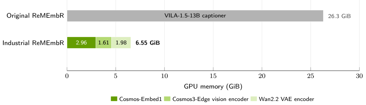
Figure 10: The three iw.encode services fit in 6.55 GiB of resident GPU memory, against a 26.3 GiB sampled process peak for the original server-side captioner. The figure shows GPU-memory profiles for both (Tab. 8); Cosmos3-Edge loads only its vision encoder.
