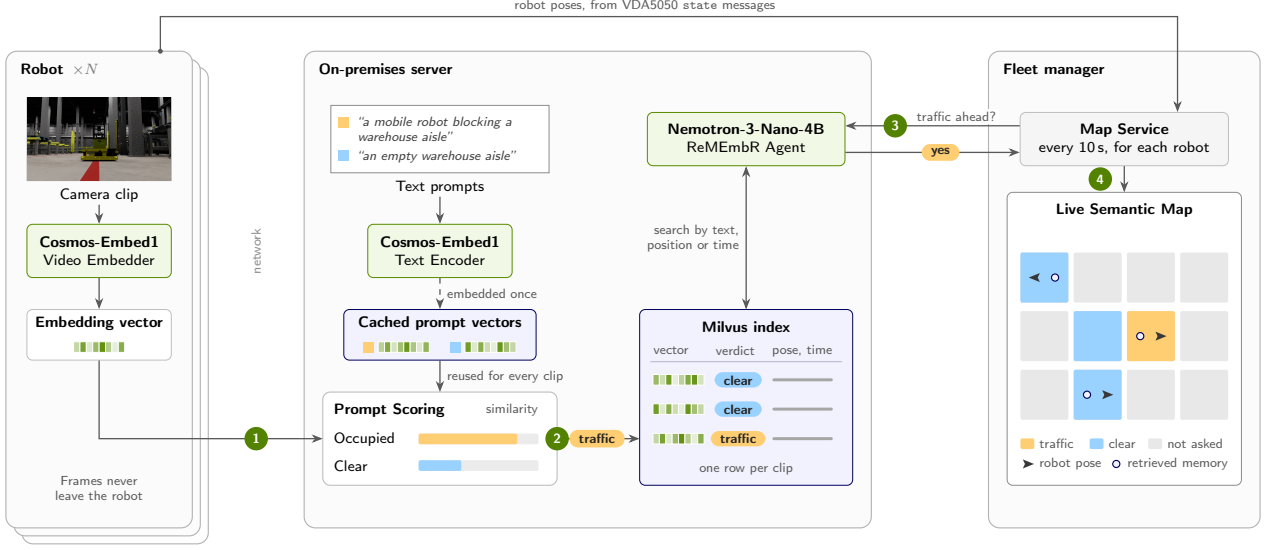
Figure 5: Robots send only a vector, pose and time, and the server turns them into a live traffic map. (1) Each robot embeds its camera clip with Cosmos-Embed1 and sends only the vector, its pose and the time. (2) The vector is compared with cached prompt vectors for an occupied and a clear aisle, and the closer one becomes the verdict stored with the memory. (3) Every 10 s, the map service asks the agent whether there is traffic ahead of each robot. (4) Each answer colors the robot’s zone, and the pose of the memory the agent retrieved is drawn beside the robot. Green boxes are NVIDIA models, blue boxes are storage.
