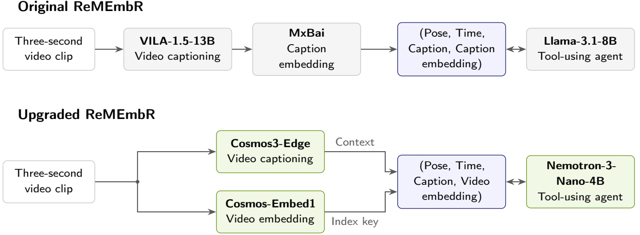
Figure 2: Upgraded ReMEMbR indexes video directly instead of caption text, so retrieval is no longer limited to what the captioner chose to say. Original ReMEMbR is shown on top and Upgraded ReMEMbR at the bottom, with the replaced components in green. In the original, the index is built from caption text, so retrieval can find only what the captioner chose to say. Upgraded ReMEMbR sends each clip down two independent paths: Cosmos-Embed1 produces the video embedding that serves as the index key, and Cosmos3-Edge produces the caption the agent reads once an observation is retrieved. Both workflows still caption every segment in advance. Bidirectional arrows denote agent tool calls and returned evidence.
