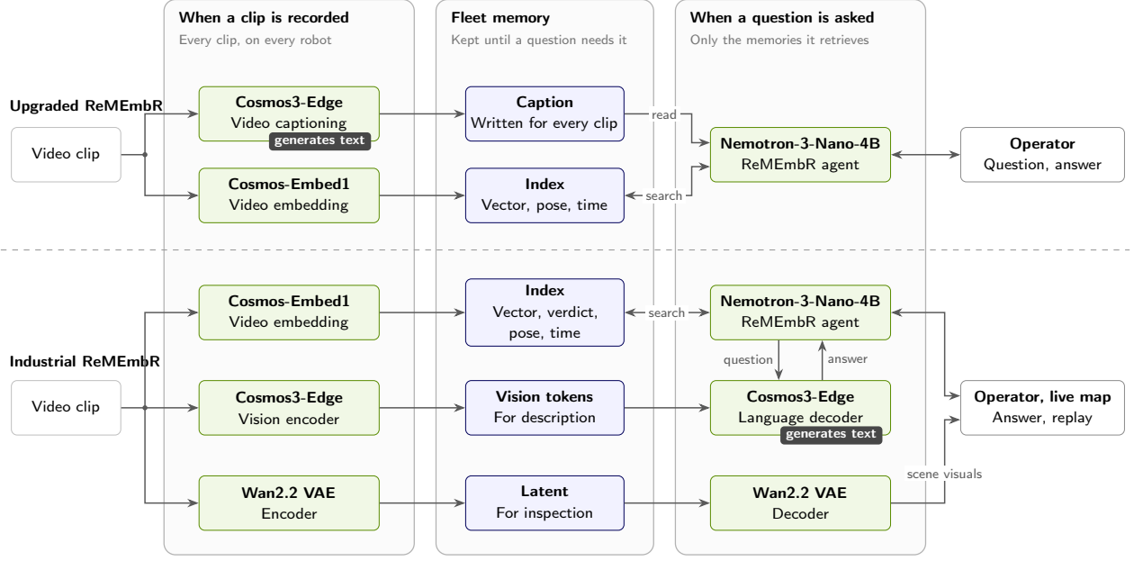
Figure 3: Industrial ReMEMbR defers text generation until a question arrives, whereas Upgraded ReMEMbR (top) fixes the text an answer can draw on when the clip is recorded. Upgraded ReMEMbR runs the full Cosmos3-Edge captioner on every clip; Industrial ReMEMbR (bottom) runs only encoders at that point and keeps their outputs in fleet memory. The language half of Cosmos3-Edge runs once a question has arrived, on the memories the agent retrieves, and the Wan2.2 decoder turns a stored latent back into video when someone wants to see the scene. The dark tag marks the step that generates text. Green boxes are models, blue boxes are storage.
