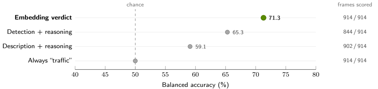
Figure 12: The caption-free embedding verdict (green) has the highest balanced accuracy among the reported representations. Results are on simulated warehouse traffic over 914 frames, by what each frame writes to memory; caption arms use reasoning. Scores exclude frames without usable context; coverage is listed at the right. The dashed line marks chance, where always answering “traffic” sits.
