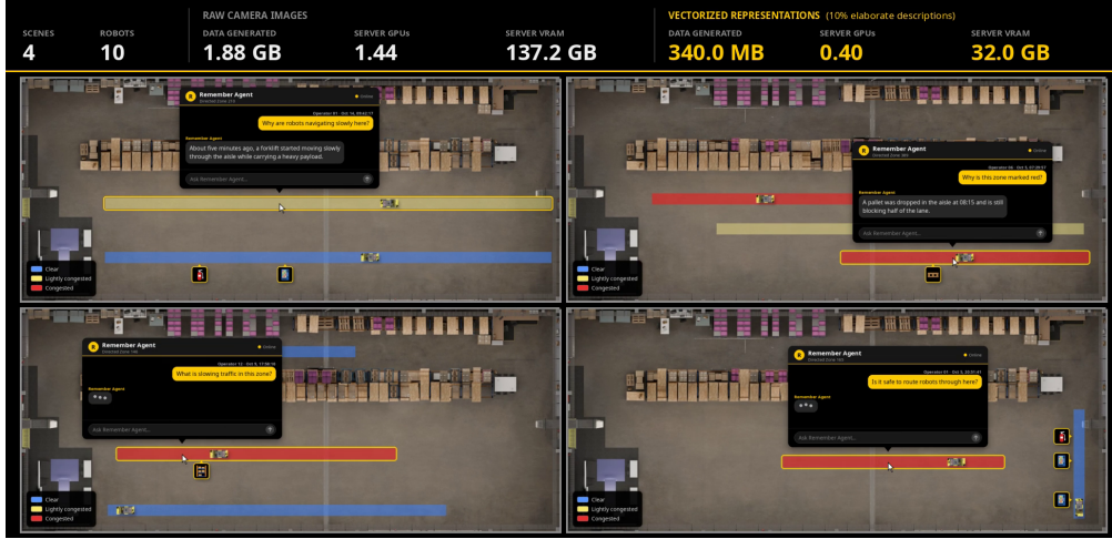
Figure 7: Operators can request an on-demand description from the Industrial ReMEMBR frontend. The popover window allows users to generate on-demand descriptions using vision tokens.
