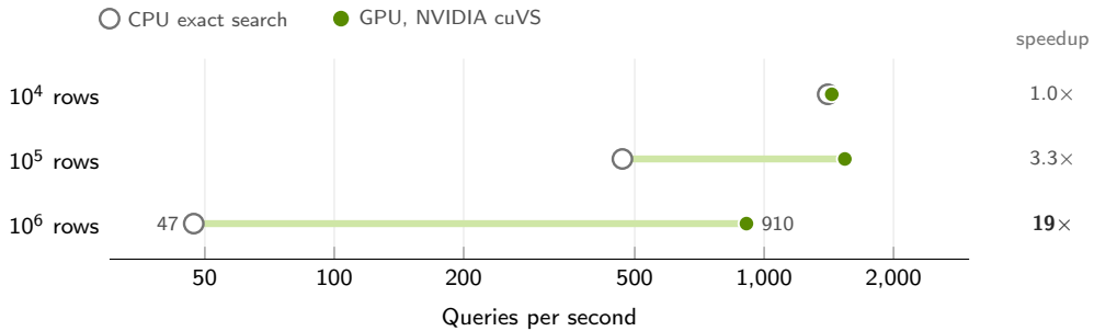
Figure 14: GPU exact search’s throughput advantage over CPU exact search grows across the tested index sizes, from parity at 10^4 rows to 3.3\times at 10^5 and 19\times at 10^6 . Results are for 32 concurrent queries in one Milvus instance over synthetic 768-dimensional vectors; the GPU index uses NVIDIA cuVS (RAPIDS Team, 2024).
