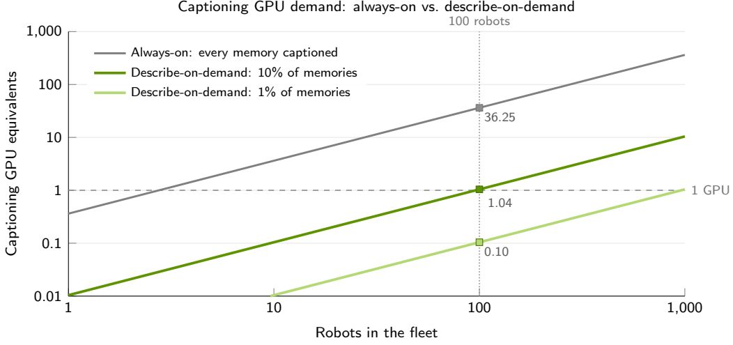
Figure 11: Measured GPU time for captioning, extrapolated at one memory per robot every 12 s. Always-on captions every memory as written (4.35 s). Describe-on-demand captions a memory only when asked (1.25 s), for 10% and 1% of memories. Squares mark 100 robots.
