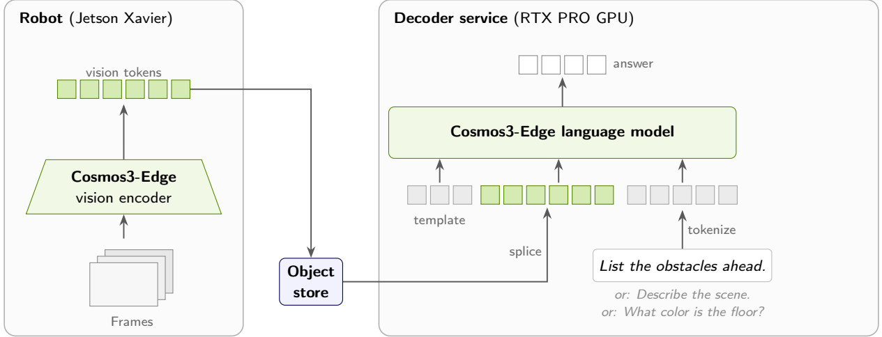
Figure 4: Cached vision tokens let the server describe a scene on demand, without the source frames. The robot runs only the vision half of Cosmos3-Edge and stores its vision tokens (green). When a question arrives, the server’s language model receives the usual chat template and the embedded question (gray), with the cached vision tokens spliced into the slot where encoded video would normally go, after checking that the token counts match. The same cached tokens can answer any number of different questions.
