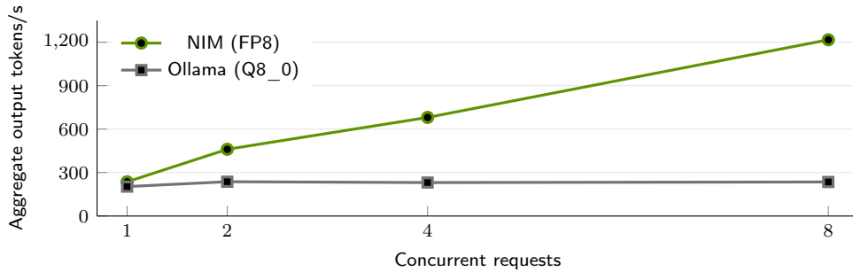
Figure 13: NIM (FP8) scales to 1217 tokens/s at 8 concurrent requests, while Ollama (Q8_0) stays near 235. Throughput is aggregate output for Nemotron-3-Nano-4B at 8k context on one RTX PRO 6000 Blackwell Server Edition.
