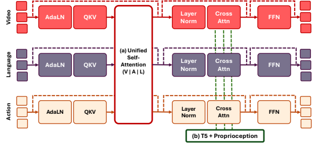
Figure 4: Mixture of Transformers Layer. Each modality is processed by its own transformer that performs adaptive layer norm followed by Q, K, V projection. The (a) unified self-attention enables feature sharing between different modalities. Each modality transformer then cross attends to the (b) task instruction and proprioception for conditional generation of video, language, and action in a unified architecture.
