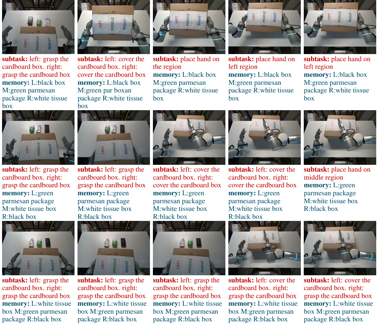
Figure 9: Real-world Find the Item rollouts. Row 1: black box ; Row 2: white tissue box ; Row 3: green parmesan package (ends at the cover-complete moment). Items are hidden mid-episode under cardboard covers; the subtask and textual memory under each frame are generated by the language DiT in tandem with the action , and the memory string is re-consumed as the next-step prompt to preserve the item-region (L/M/R) mapping across the occlusion.
