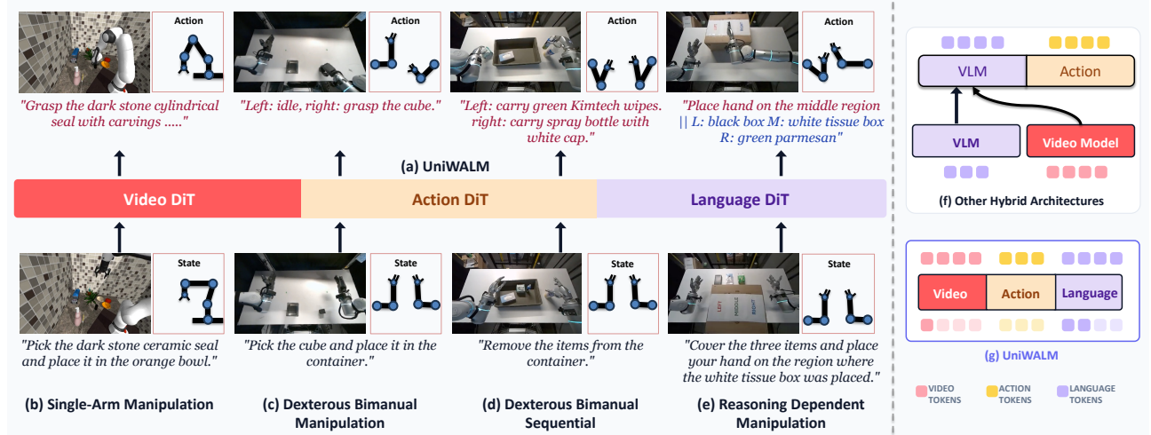
Figure 1: (a) UniWALM is a unified World Action Language Model that extends a single video-model backbone to act and reason by co-generating video, action, and language through one shared diffusion process — no separate language model fused onto a world-action model. This supports (b) single and (c) bimanual dexterous manipulation with (d) multi-stage manipulation and (e) memory-dependent reasoning . Prior work (f) composes a VLM with a VLA and a video model in pipeline or parallel; UniWALM (g) tunes a single unified representation end-to-end. Each manipulation example displays the input task instruction at the bottom and the generated video, action, and subtask at the top. In (e) the predicted subtask and textual memory (shown as ‘ subtask || memory ’) are re-consumed as the next-step prompt.
