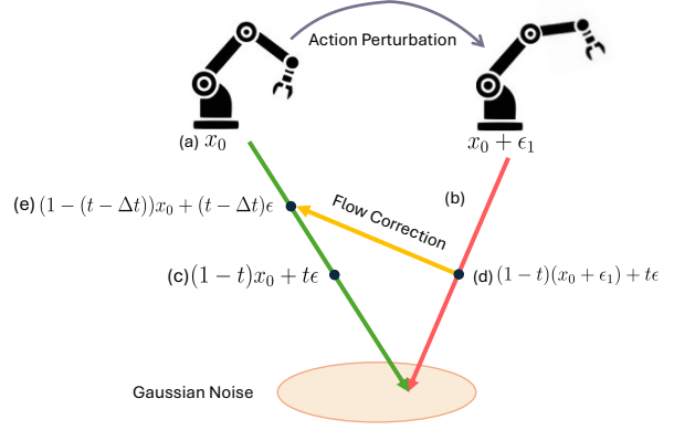
Figure 3: Flow Matching with Correction (FMC) . A clean action x_0 (green path) and its perturbed counterpart x_0 + \epsilon_1 (red path) are noised to the same time t . The model is trained to transport the perturbed sample back onto the clean trajectory within \Delta t (yellow arrow), while the clean branch follows standard flow matching. This requires no extra conditioning or model capacity and leaves inference unchanged.
