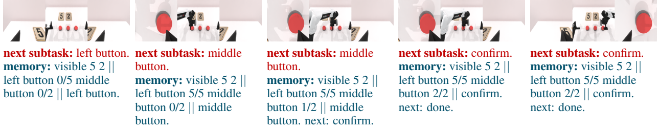
Figure 12: Timing-lag failure on Press Button. Target counts are (left = 5, middle = 2, confirm = 1). The memory readout tracks the intended count correctly (left 5/5, middle 2/2, confirm, next: done), but the action executor over-shoots by one press on middle, yielding 3 physical middle presses instead of 2. The language-memory loop is correct; the task-completion channel fires one step late, so the action expert continues the current subtask for one extra press.
