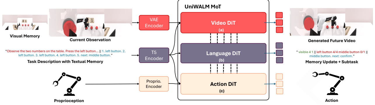
Figure 2: Overview of UniWALM. UniWALM is a unified mixture-of-transformers (MoT) world-action-language model that co-denoises video, language, and action in a single shared representation. Given the current observation, task instruction, proprioception, an optional visual memory \mathcal{F} (one or more frames; in our experiments a single anchor at episode start), and the previously generated textual memory , UniWALM processes inputs through a (a) video , (b) language , and (c) action DiT that share features via unified self-attention. The language stream emits a subtask together with a textual memory string, which is re-consumed as the prompt on the next control step, closing a language-as-memory loop across time. Video generation is disabled at inference, so the language and action DiTs run without producing future frames.
