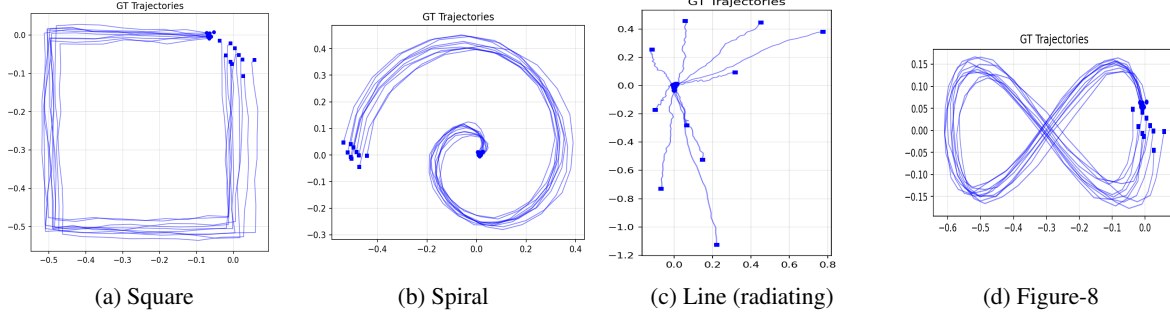
Figure 10: 2D robot-trajectory benchmark used for FMC ablation. Each shape class contains multiple noisy demonstrations sharing a canonical motion pattern (blue curves show ground-truth trajectories). Shapes span repeating closed motion (Square, Figure-8), unbounded expansion (Spiral), and multi-modal starts (Line’s radial variants). The policy is trained to generate trajectories matching the full distribution of each class.
