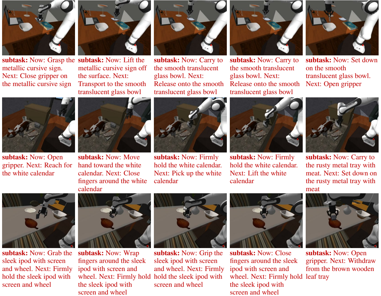
Figure 13: MolmoSpaces Pick & Place rollouts (sim). Each row is a successful UniWALM rollout across diverse scenes. The subtask under each frame is generated by the language DiT in tandem with the action (co-denosed in the same forward pass), not produced autoregressively before action.
