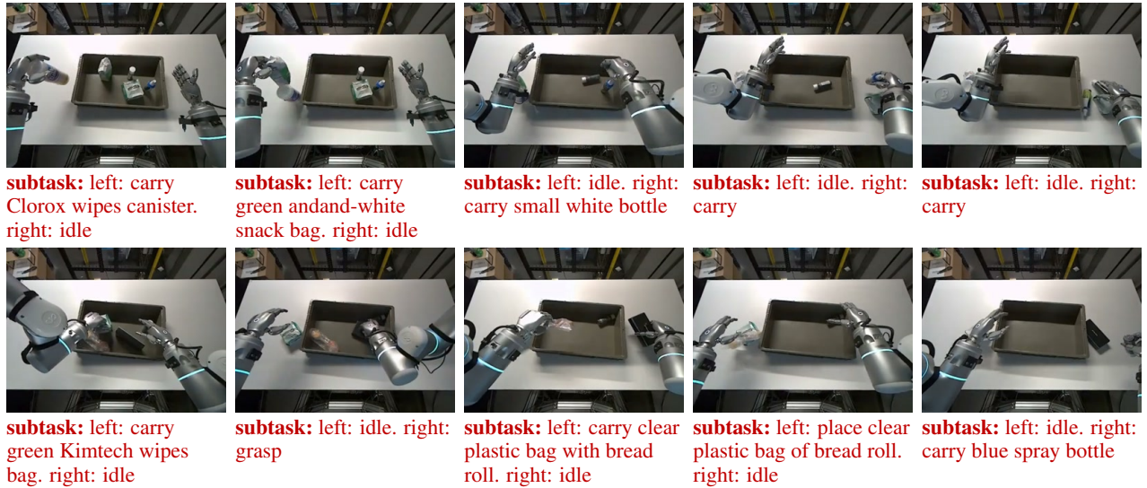
Figure 8: Empty Container (real, bi-manual) rollouts. Each row is a successful UniWALM rollout. The subtask under each frame is generated by the language DiT in tandem with the action (co-denoised in the same forward pass).
