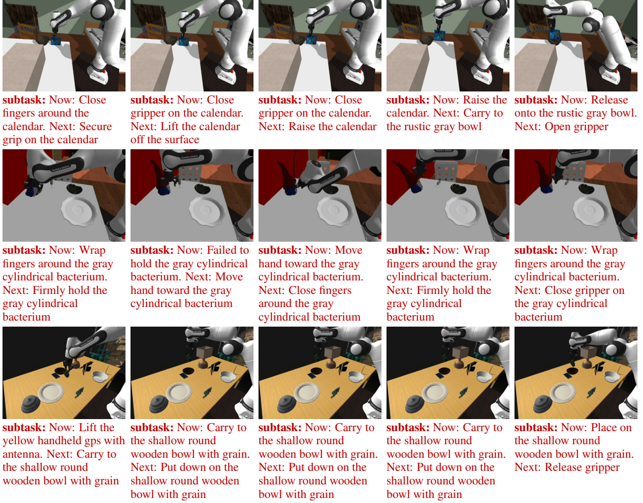
Figure 14: MolmoSpaces Pick & Place rollouts (sim). Each row is a successful UniWALM rollout across diverse scenes. The subtask under each frame is generated by the language DiT in tandem with the action (co-denoised in the same forward pass), not produced autoregressively before action.
