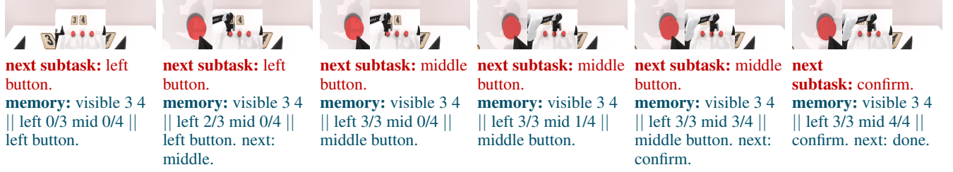
Figure 7: Language-as-memory loop on Press Button. At each step UniWALM emits a next subtask and textual memory that is re-consumed as the next-step prompt; press counters transition cleanly (left 0/3 \rightarrow 3/3; middle 1/4 \rightarrow 4/4) until confirm. Intermediate frames skipped for clarity; see Fig. 6 for all four M(n) tasks.
