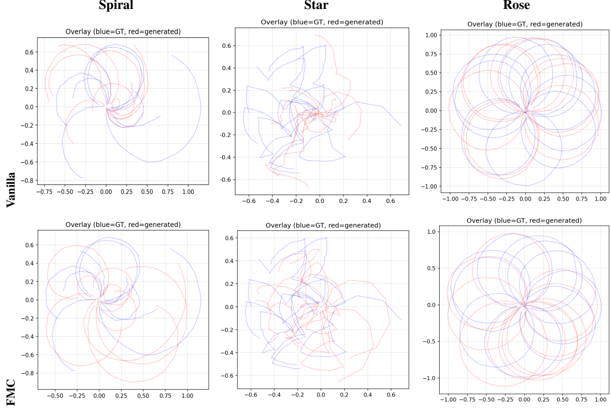
Figure 11: FMC vs vanilla flow matching on 2D robot trajectories (overlay view). Blue curves are ground-truth demonstrations; red are model-generated trajectories, overlaid for direct comparison. Top row: vanilla flow matching frequently drifts off the demonstration manifold, truncates the shape, or collapses mode coverage. Bottom row: FMC tracks the ground-truth distribution more faithfully across all three shape classes, consistent with the quantitative Chamfer improvements in Tab. 6.
