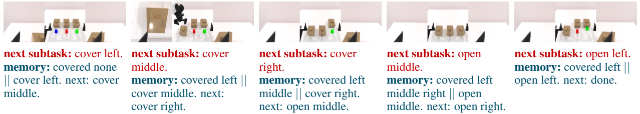
Figure 6: RMBench M(n) qualitative rollouts . Each row is a successful UniWALM rollout on one M(n) task; we display a subsampled sequence of inference steps for clarity. Below each panel we show the predicted next subtask and the generated textual memory that is re-consumed as the prompt on the next control step; within the memory string, “||” separates memory components (task state, progress counters, and the next subtask). Reading left-to-right shows how the language-memory loop accumulates task-relevant state (button counts, battery orientations, tried permutations, cover progress) that memoryless baselines lose across steps.
