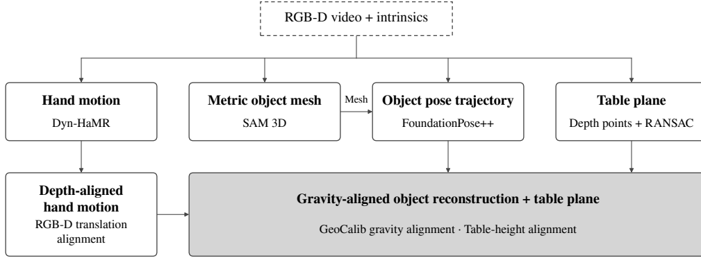
Figure 7: Overview of our RGB-D hand-object reconstruction pipeline. Given an RGB-D video and camera intrinsics, we recover hand motion with Dyn-HaMR, reconstruct a metric object mesh with SAM 3D, and track its pose with FoundationPose++. A table plane is estimated from depth points using RANSAC. We align hand translations to the observed depth, then apply GeoCalib-based gravity alignment and table-height alignment to express the hand, object, and table in a shared world coordinate frame.
