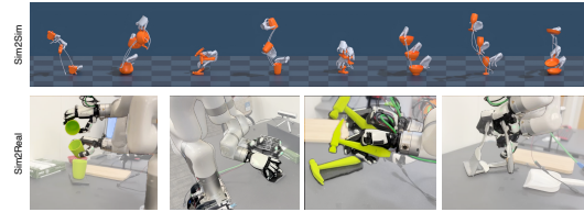
Figure 6: Sim-to-sim and sim-to-real transfer, in real time ( 1x speed, 30 Hz ), demonstrating physical feasibility of the learned dexterous behaviors.
