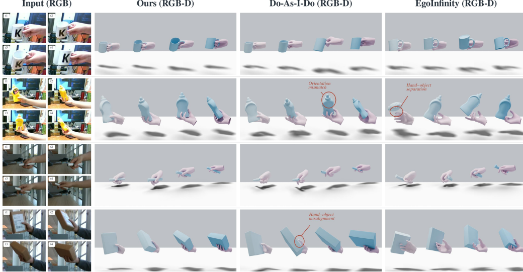
Figure 8: Qualitative comparison of hand-object reconstruction. Each row shows four time steps from an interaction, with RGB inputs arranged in reading order and reconstructions ordered from left to right. Do-As-I-Do and EgoInfini are adapted to use the provided depth maps and calibrated camera intrinsics. Our reconstructions more closely preserve the object orientations and grasp configurations observed in the input videos.
