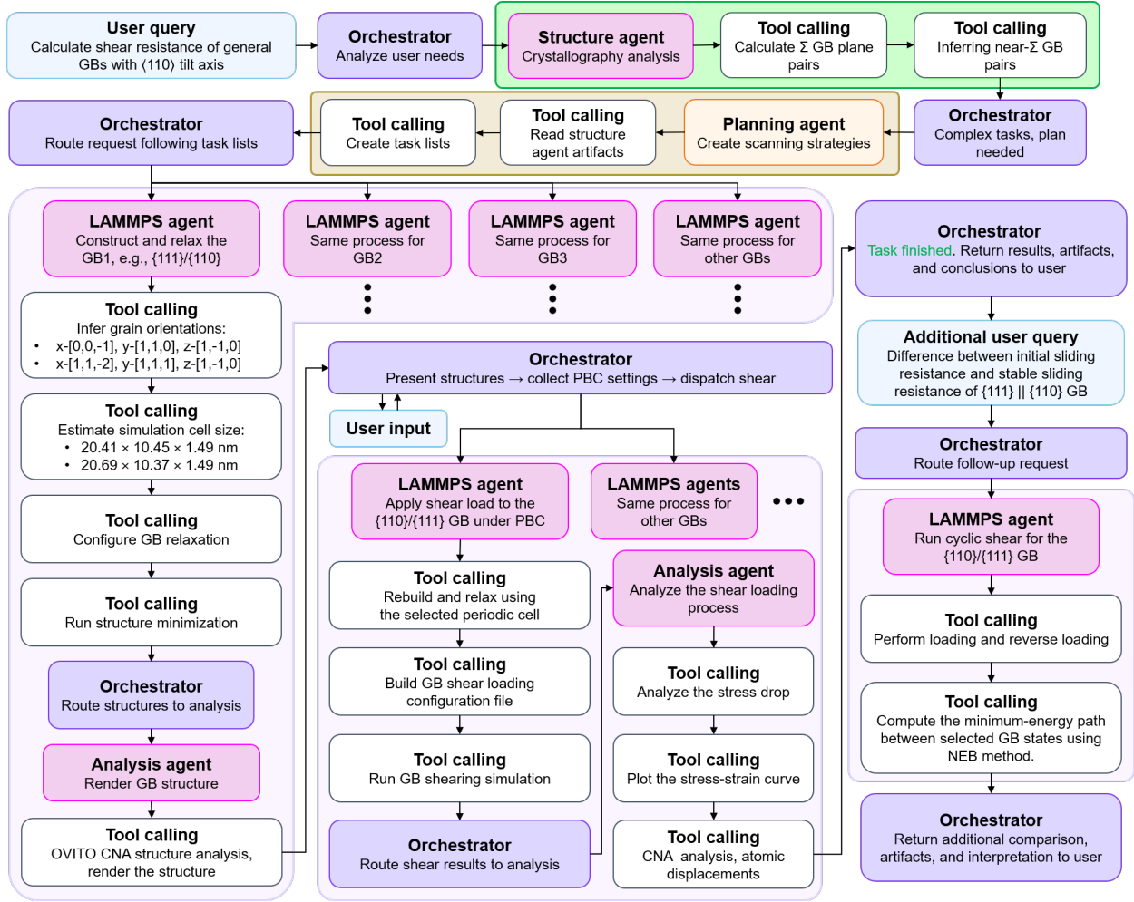
Fig. S2 | Detailed GBClaw workflow for investigating GB shear strength. Automated tasks and researcher guidance connect crystallographic screening, simulation planning, parallel bicrystal construction and relaxation, selection of periodic boundary conditions, shear simulations, and structural and mechanical analysis of general asymmetric \{110\} tilt GBs. The \{110\}/\{111\} GB illustrates an adaptive investigation, in which an unexpected shear response prompted researcher-directed follow-up analyses using cyclic shear simulations and NEB calculations.
