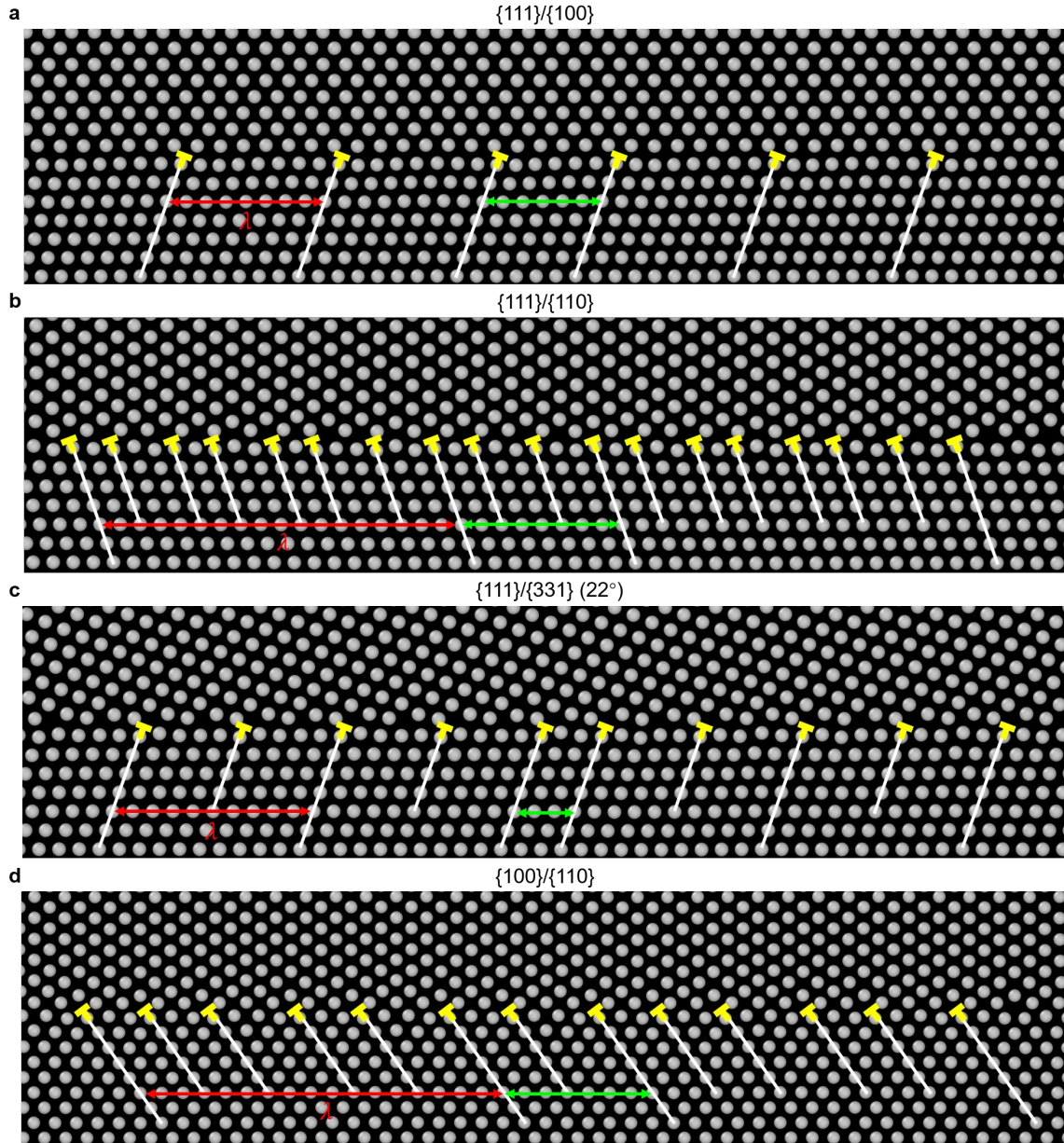
Fig. S4 | Identification of SGMDs from projected atomic-column arrangements in simulated structures. a, \{111\}/\{100\} GB. b, \{111\}/\{110\} GB. c, \{111\}/\{331\} ( 22^\circ ) GB. d, \{100\}/\{110\} GB. All configurations are viewed along the common \langle 110 \rangle tilt axis. White lines trace edge-on atomic planes, and yellow markers identify their interfacial terminations. Red double-headed arrows indicate the primary structural periodicity \lambda . Green double-headed arrows span the altered row correspondence within SGMD cores. Comparing core and reference row counts gives the Burgers vector magnitudes listed in Table S2, consistent with Table 2 and the near-CSL analysis in Fig. S6.
