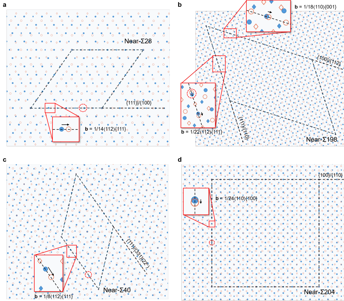
Fig. S6 | Determination of SGMD character from near-CSL dichromatic patterns of the four pure-sliding GBs. a , \{111\}/\{100\} GB; b , \{111\}/\{110\} GB; c , \{111\}/\{331\}(22^\circ) GB; d , \{100\}/\{110\} GB. Blue and orange symbols distinguish the two grain lattices, while circles and diamonds distinguish alternating atomic layers along the \langle 110 \rangle tilt axis. Black dashed lines indicate the near-CSL cells and GBs. Black arrows indicate the shortest DSC translations connecting lattice sites in the two grains within the same atomic layer. These translations define the SGMD Burgers vectors and agree with those obtained from the projected atomic-column analysis in Fig. S4 and Table S2. Red dashed circles mark symmetry-related site pairs that produce DSC translations equal in magnitude but opposite in sign to those indicated in red solid boxes.
