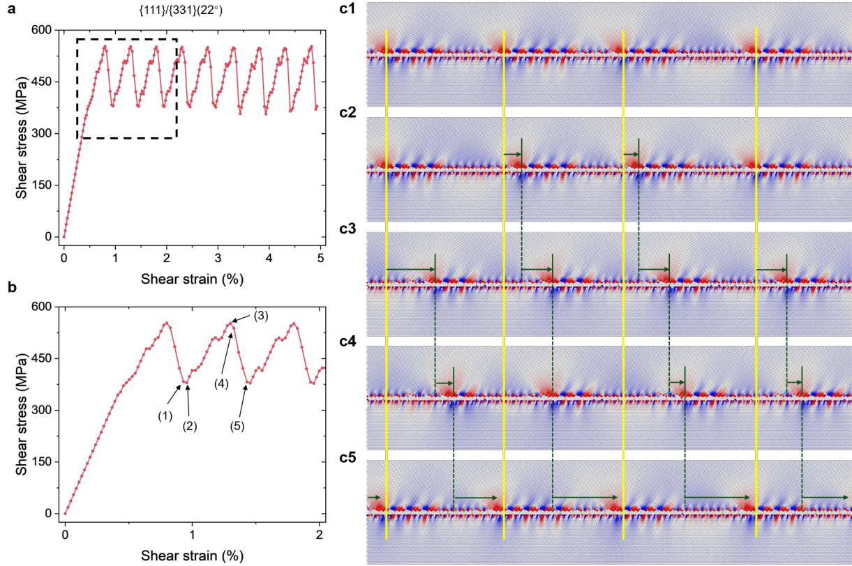
Fig. S7 | Boundary sliding through nonuniform glide of SGMDs in the \{111\}/\{331\}(22^\circ) GB. a , Shear stress as a function of applied shear strain. b , Magnified view of the stress response, with states (1) to (5) marking a representative sliding cycle. c1 to c5 , Atomic configurations corresponding to the marked states. Large red regions identify SGMD cores. Yellow lines mark equivalent SGMD positions at the beginning and end of the cycle. Green lines track dislocation positions, and arrows indicate movement between consecutive configurations.
