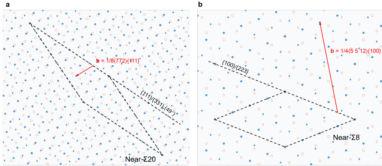
Fig. S10 | Analysis of near-CSL dichromatic patterns associated with shear-coupled migration. a, \{111\}/\{331\}(49^\circ) GB. b, \{100\}/\{223\} GB. Colors distinguish the grain lattices, and symbol shapes distinguish layers along the \langle 110 \rangle tilt axis. Dashed lines indicate the near-CSL cells and GB traces. Red arrows mark DSC vectors selected by comparison with the signed tangential-to-normal displacement ratios measured during migration (Fig. S9). Crystallographic directions are referenced to the grains indicated in each panel.
