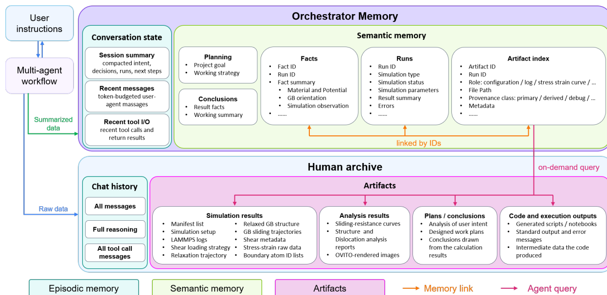
Fig. S1 | Memory organization and identifier-based information flow in GBClaw. Conversation state retains the session summary, recent messages, and recent tool inputs and outputs. Semantic memory stores project plans, conclusions, facts, run records and an artifact index. Shared run IDs connect fact records with simulation conditions and outputs, while artifact IDs link indexed entries to the corresponding files for retrieval on demand. Complete interaction and tool execution histories are archived for human review. Green and blue arrows represent summarized and raw information, respectively. Orange arrows denote memory links, and magenta arrows indicate artifact queries.
