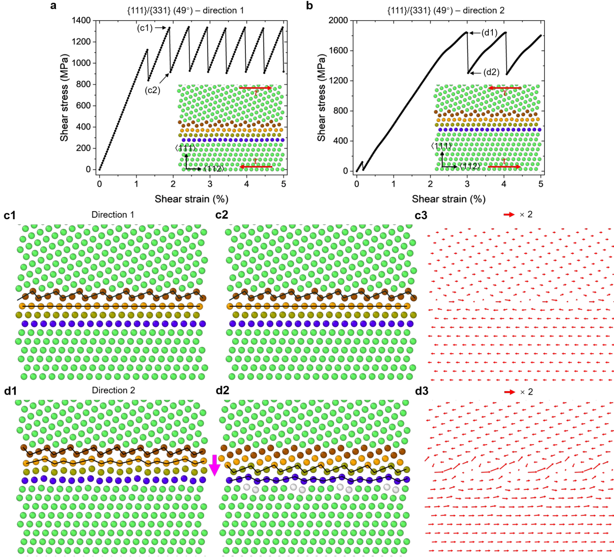
Fig. 6 | Shear asymmetry in the \{111\}/\{331\}(49^\circ) GB. a, b , Shear stress as a function of applied shear strain along directions 1 and 2, respectively. Insets show the initial boundary structures and shear directions. c1-c3 , Pure GB sliding when sheared along direction 1. d1-d3 , Shear-coupled GB migration when sheared along direction 2. c1, d1 and c2, d2 show configurations before and after, respectively, the stress drops indicated in a and b . c3, d3 , Corresponding atomic displacement vectors, amplified twofold for clarity. Selected atomic rows are colored to highlight structural changes. Black lines mark terminating planes. The magenta arrow indicates downward boundary
