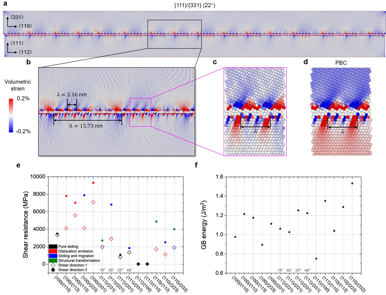
Fig. 3 | Atomic structures, structural periodicities, and shear responses of selected asymmetric incommensurate GBs. a , Extended GB in a Ni bicrystal after energy minimization, joining {331} and {111} terminating planes at a 22° misorientation angle, denoted as {111}/{331}(22°). b , Magnified view of the interface. Small and large red regions near the {331} terminating plane identify the cores of PGMDs and SGMDs, respectively. The primary period ( \lambda = 2.16 \text{ nm} ) is the spacing between the repeating arrangement of PGMDs, and the secondary period ( \Lambda = 15.73 \text{ nm} ) is the spacing between adjacent SGMDs. c , Magnified view of the boundary showing adjacent PGMDs separated by one \lambda . d , Periodic supercell constructed from the structure in c and relaxed under PBCs to eliminate normal stress components for uniform sliding simulation. Atoms in a-d are colored according to atomic volumetric strain. e , Athermal shear strengths of the selected asymmetric incommensurate GBs loaded in opposite directions parallel to the GB plane and perpendicular to the \langle 110 \rangle tilt axis. Directions 1 and 2 denote the lower and higher shear resistance, respectively. Symbol colors represent the observed deformation modes. f , Relaxed GB
