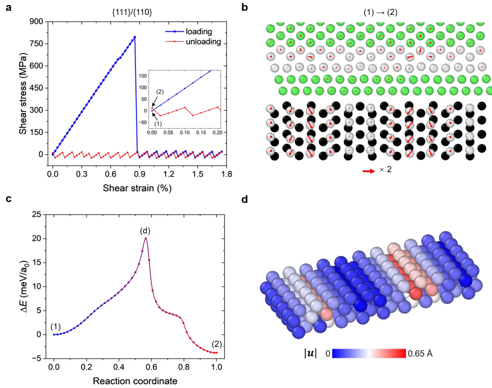
Fig. 5 | Loading-induced local reconstruction and associated energy barrier in the \{111\}/\{110\} GB. a. Shear stress-strain response during loading (blue) and unloading (red). The inset shows the residual shear stress of the initial relaxed configuration (1) and the final unloaded configuration (2), both evaluated at zero applied shear strain. b. Edge-on (upper) and plan (lower) views of configuration (2). Red arrows indicate atomic displacement vectors from configuration (1) to (2), scaled by a factor of two. c. Minimum energy path from an NEB calculation connecting configurations (1) and (2) at zero applied shear strain. d. Atomic configuration at the saddle point in c . Atoms are colored by their displacement magnitude relative to configuration (1).
