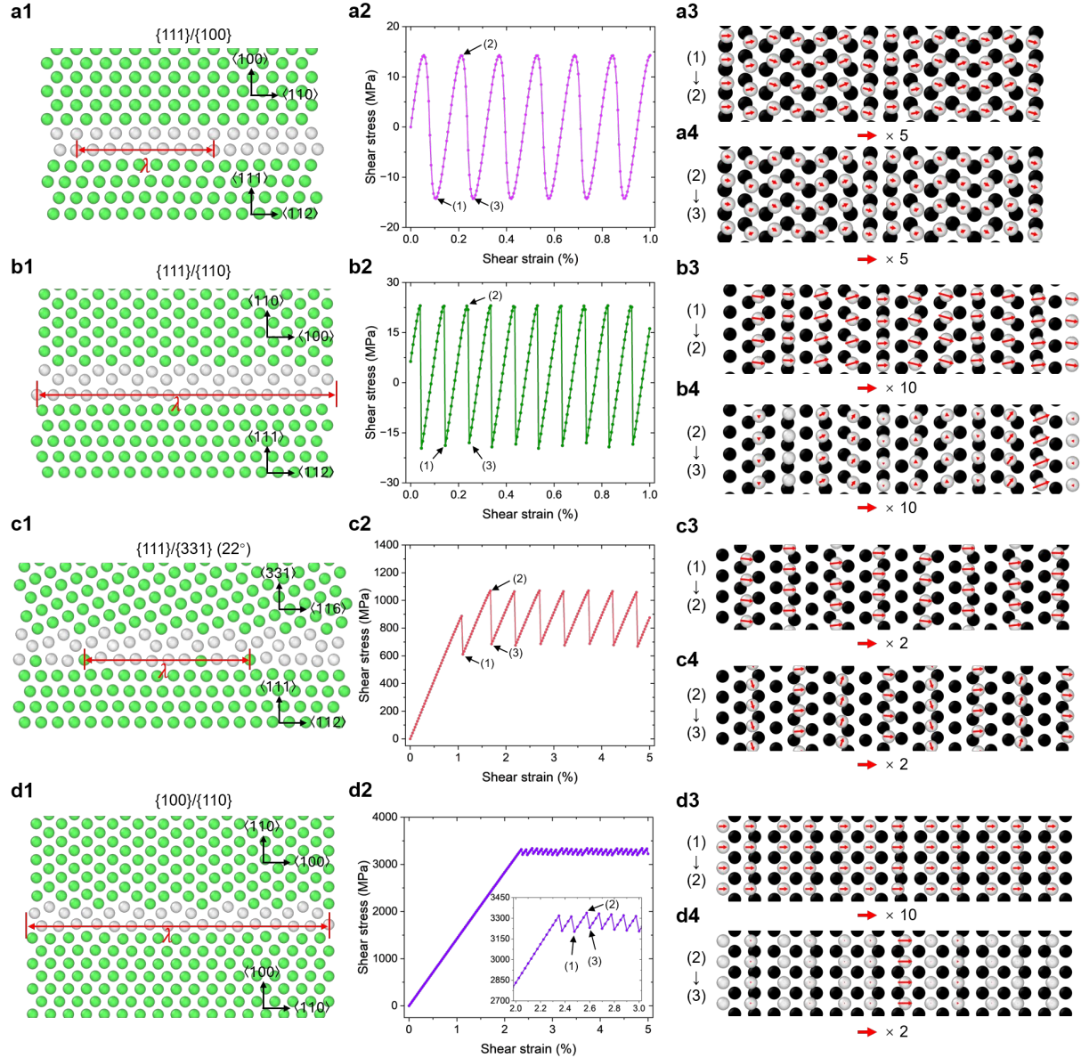
Fig. 4 | Supercell atomic structures, shear stress-strain responses, and displacement fields of GBs exhibiting pure sliding. a1–a4, \{111\}/\{100\} GB; b1–b4, \{111\}/\{110\} GB; c1–c4, \{111\}/\{331\}(22^\circ) GB; d1–d4, \{100\}/\{110\} GB. For each boundary, panel 1 shows the relaxed atomic structure in a compact supercell with PBCs applied in the boundary plane, with
