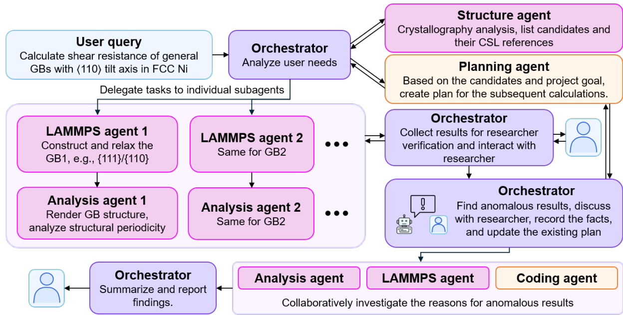
Fig. 2 | Agentic GBClaw workflow for systematic screening and mechanistic analysis of GB shear strength. The workflow combines automated exploration with human-in-the-loop domain guidance across six key stages: crystallographic screening, simulation planning, parallel bicrystal construction and structural analysis, researcher review, dynamic replanning, and targeted investigation of anomalous shear responses in general asymmetric \{110\} tilt GBs.
