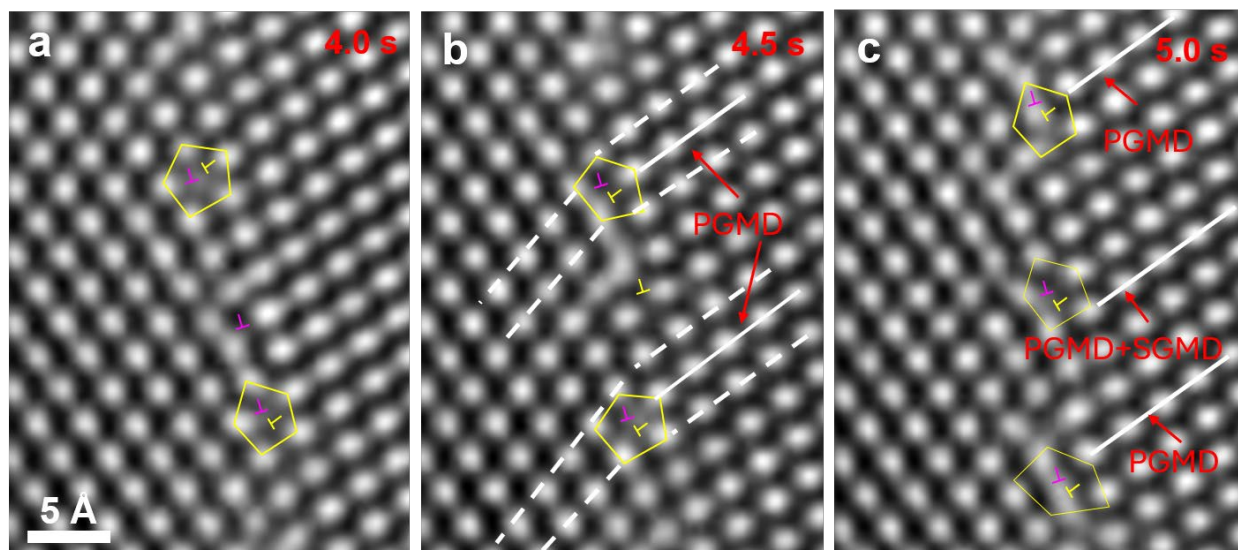
Fig. S5 | Identification of SGMDs from projected atomic-column arrangements in in situ HRTEM images of a \{111\}/\{331\}(22^\circ) GB undergoing sliding , adapted from Wang et al 35 . a, b , Each image shows two PGMDs. In b , solid white lines trace extra \{111\} half-planes, whose interfacial terminations identify the PGMD cores. c , An SGMD identified by an additional \{111\} half-plane. The associated atomic-column arrangement is consistent with the simulated structure shown in Fig. S4c.
