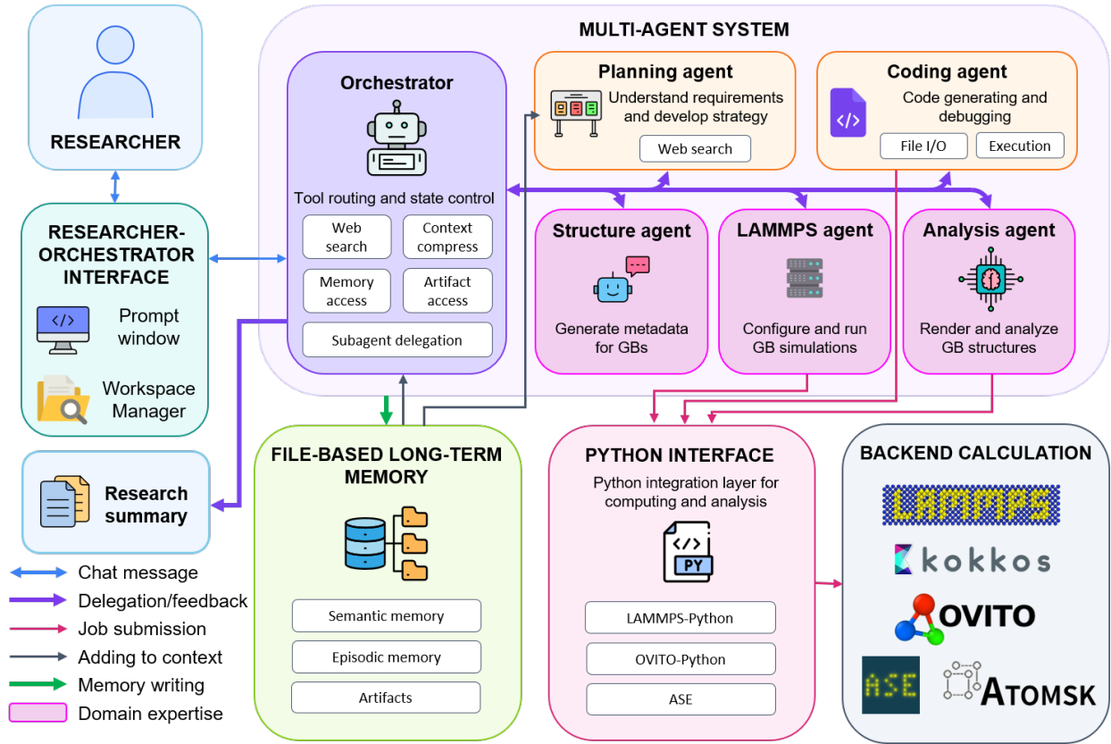
Fig. 1 | Agentic architecture of GBClaw for researcher-guided grain boundary research. The orchestrator serves as the central coordination hub, interfacing the researcher with five specialized agents, domain-specific scientific software tools, and a file-based hierarchical memory system. The modular architecture enables automated task decomposition and delegation, parallel simulation execution, structured information exchange, and interactive, human-in-the-loop workflow refinement.
