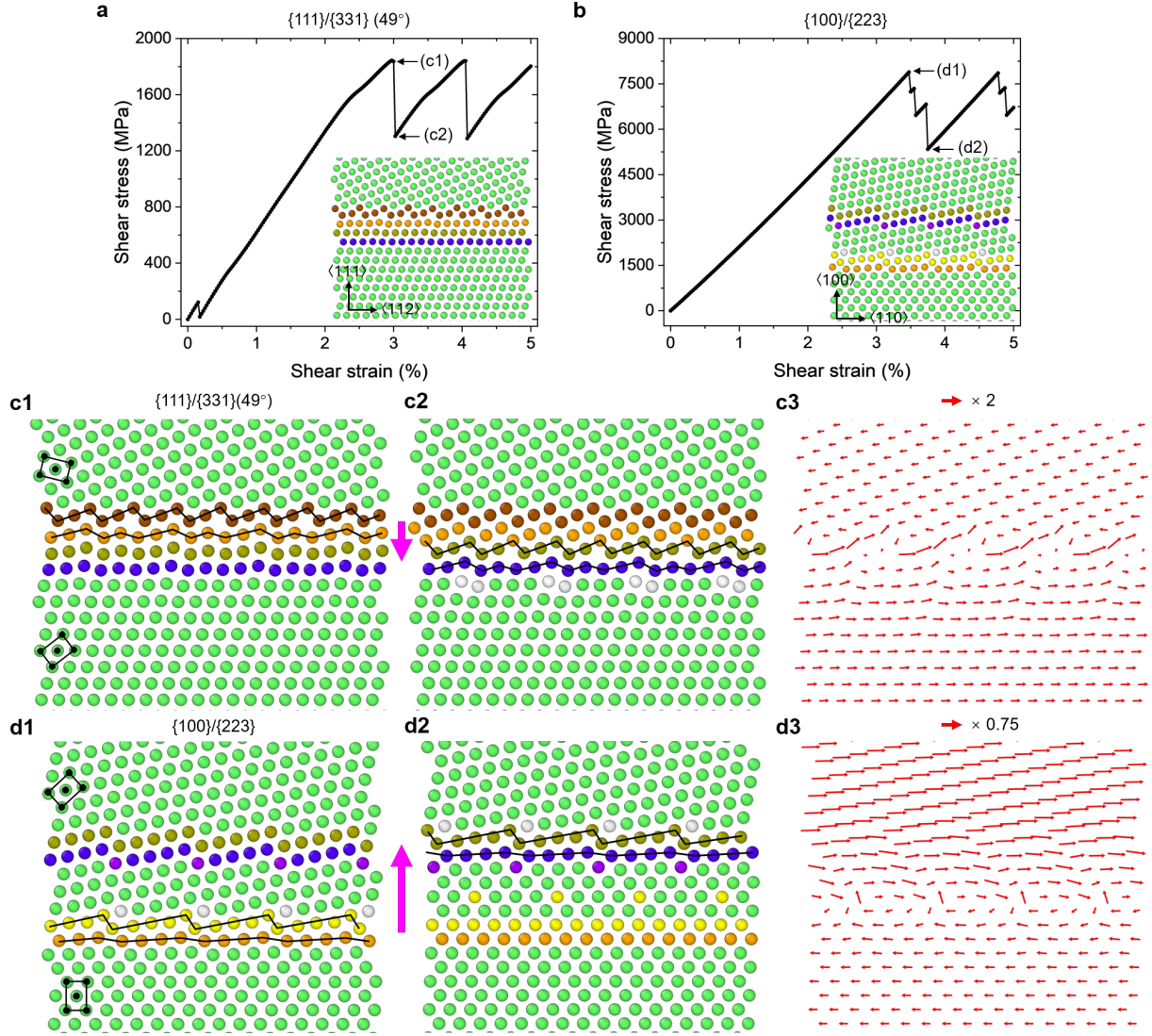
Fig. S9 | Spatially periodic atomic shuffling during shear-coupled GB migration. Shear stress as a function of applied shear strain for a , \{111\}/\{331\} (49°) GB loaded in direction 2 and b , \{100\}/\{223\} GB. Insets show the corresponding initial GB structures. Atomic configurations of the \{111\}/\{331\} (49°) GB, c1 , before and, c2 , after the selected migration interval. d1-d2 , Corresponding atomic configurations of the \{100\}/\{223\} GB. Selected atomic sites are shown in distinct colors to facilitate structural tracking. Black lines trace the terminating atomic planes, outlined crystallographic cells indicate the orientations of the two grains, and magenta arrows mark the directions of GB migration. c3 , d3 , Differential atomic displacement vectors from c1 to c2 and from d1 to d2 , respectively. The red vectors are amplified by factors of 2 and 0.75, respectively. All atomic configurations are viewed along the \langle 110 \rangle tilt axis.
