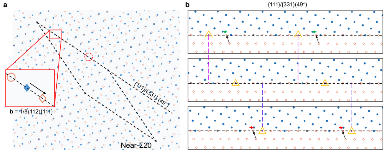
Fig. S8 | SGMD Burgers vector derived from the near-CSL pattern of the \{111\}/\{331\}(49^\circ) GB. a , Near-CSL dichromatic pattern. Blue and orange symbols distinguish between the two grain lattices, while circles and diamonds distinguish atomic layers along the \langle 110 \rangle tilt axis. Dashed outlines indicate the near-CSL cell. The black arrow in the inset marks the shortest DSC vector connecting sites of the two lattices, yielding \mathbf{b}_s = 1/8\langle 112 \rangle \{111\} , identical to that of the 22^\circ boundary in Fig. S6c. The dashed circle marks a symmetry-related pair of sites with opposite relative offsets in the reference pattern. b , Local interfacial configurations, with the blue and orange grains positioned above and below the GB, respectively. Taking the middle configuration as the reference, the orange atoms are held fixed, while the blue atoms are translated left by -\mathbf{b}_s to obtain the upper configuration and right by +\mathbf{b}_s to obtain the lower configuration. Green and red arrows denote these opposite tangential translations, each equal in magnitude to the Burgers vector of the SGMD ( \mathbf{b}_s ). Black arrows indicate the resistance from second-nearest-neighbor atoms beneath the terminating plane. Yellow triangles highlight coincidence lattice sites, and vertical dashed guides provide positional references across the three registries.
