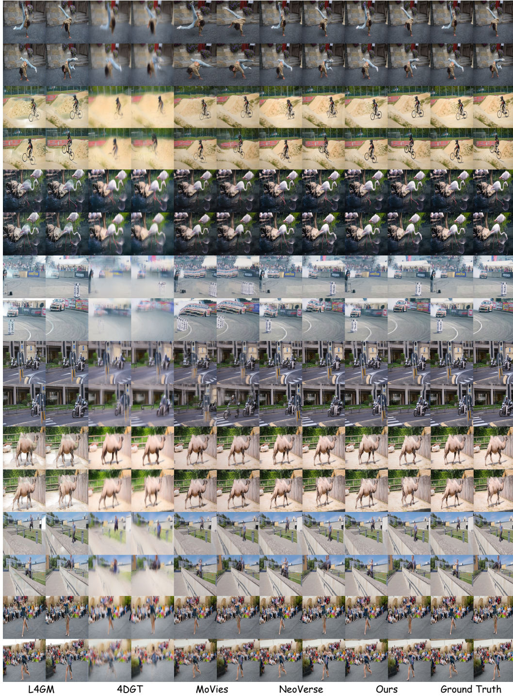
Figure 4: Additional qualitative reconstruction comparisons on DaVis. AEON produces more coherent geometry and finer details in dynamic regions.
