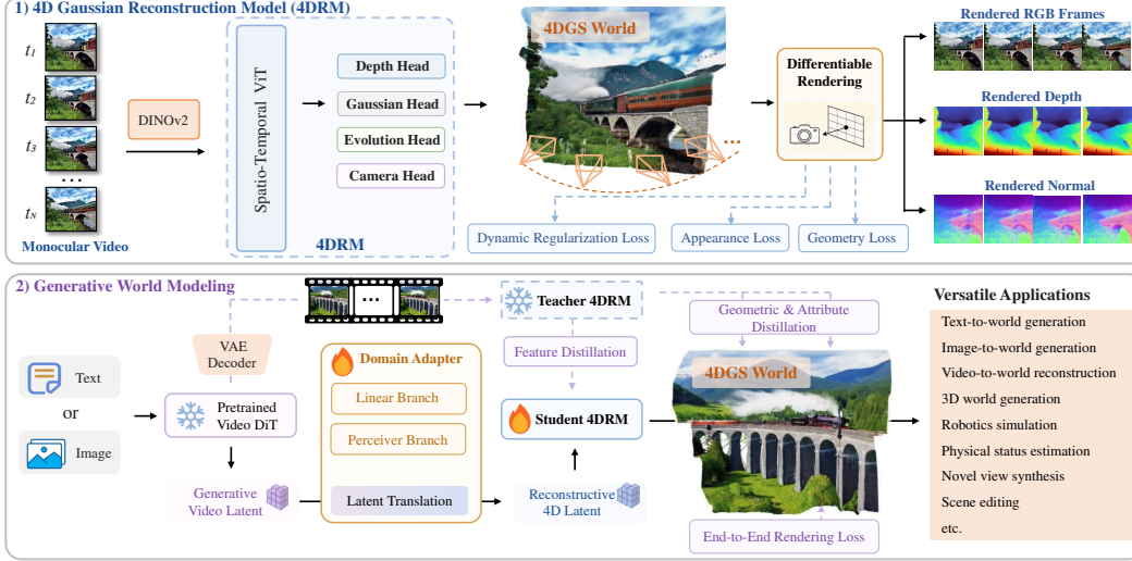
Figure 2: Overview of AEON. Top (1). The 4D Reconstruction Model (4DRM) decodes a monocular video into a 4DGS world through four task-specific heads that respectively predict depth, Gaussian appearance, dynamic evolution, and camera poses. The resulting primitives are rasterized into RGB, depth, and normal maps for end-to-end supervision. Bottom (2). We train AEON for generative world modeling by distilling the world generative capability of a frozen video diffusion model (e.g., Wan 2.2 [38]) and the 4D reconstructive capability of a teacher 4DRM via a Domain Adapter and a learnable student 4DRM. The generated explicit 4DGS world enables versatile world modeling applications.
