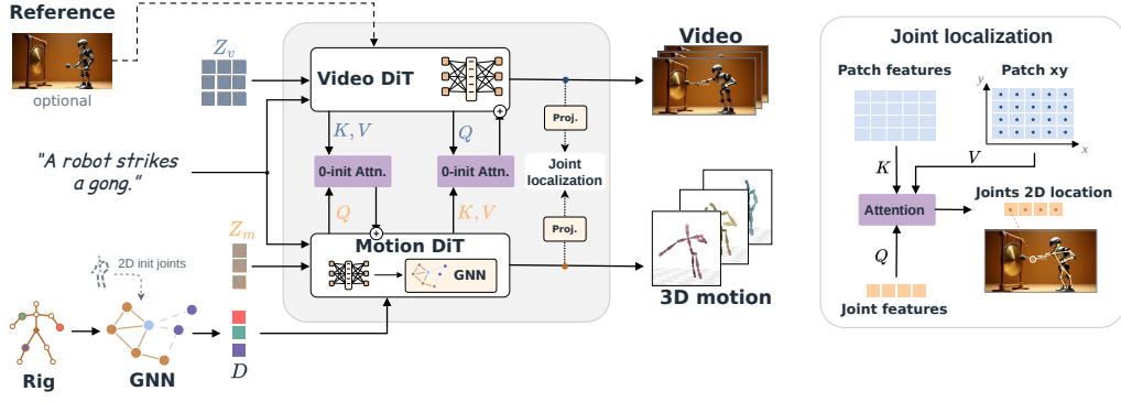
Figure 2: Architecture overview. Given a text prompt, a rig, and an optional reference image, the model jointly denoises video latents Z_v and motion tokens Z_m . A graph network encodes the rig into per-joint descriptors D , using the joints’ 2D locations in the reference image, and these condition the motion branch; a graph-attention layer inside each Motion DiT block propagates features along the rig edges. Zero-initialized cross-attention bridges exchange features in both directions at paired blocks, each branch querying the other’s intermediate features, so joint training begins from the two pretrained branches acting as they did in isolation. An auxiliary joint-localization head (right) attends from joint features to video patches and returns each joint’s image position as a weighted combination of patch coordinates, giving 2D–3D correspondences used to fit a camera.
