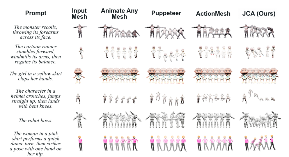
Figure 3: Text-driven rig animation across diverse assets. Each row shows a text prompt, an input mesh, and sampled poses from animations generated by competing methods and JCA (ours). Our method more faithfully captures the requested actions while preserving the asset’s geometry.
