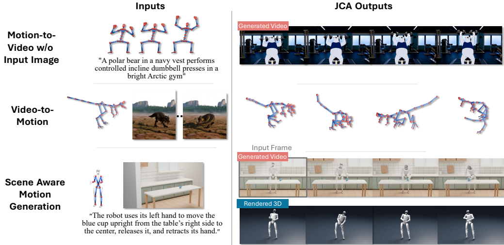
Figure 4: Additional Applications of our model. Top: Unlike the setting in fig. 1, we generate a video from a rig motion sequence and a text prompt, without an input image. Middle: An additional video-to-motion example with a different skeletal topology. Bottom: Given the rig and mesh of a real Unitree G1 robot, a 3D scene, an initial pose, and text, we jointly generate video and motion; we show the video alongside the mesh driven by the generated motion and rendered in the scene.
