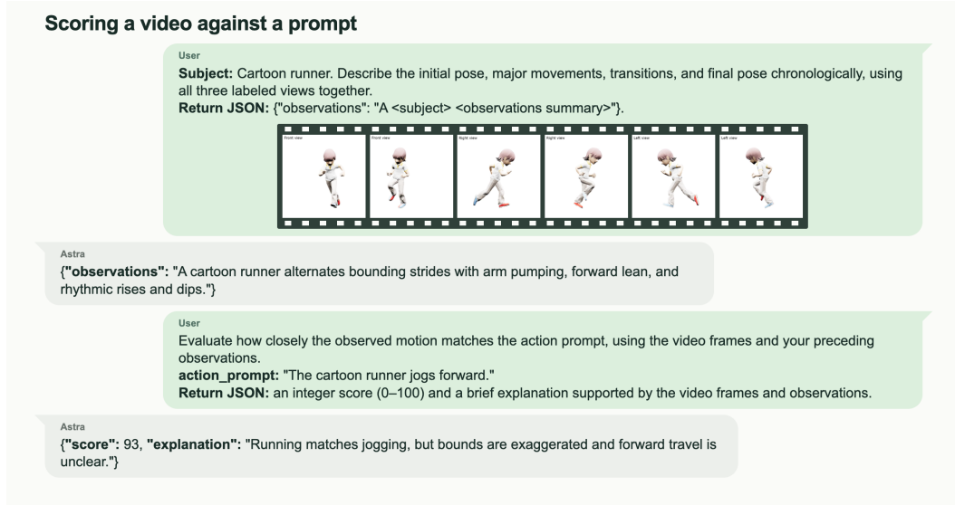
Figure 6: Prompt-adherence evaluation of one animation with GPT-6 Astra. In the first turn, the judge is given the asset’s short description and 48 frames of the animation, 16 from each of the front, right, and left views, each frame labeled with its view; the figure shows two frames per view. It is asked to describe the motion it observes in chronological order. In the second turn, it scores the motion against the action prompt. The complete prompts and responses are given in section B.3.
