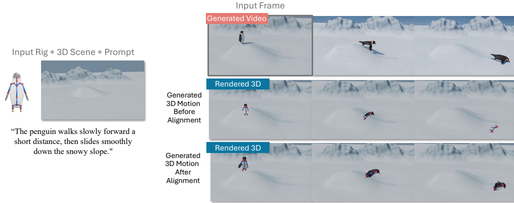
Figure 5: Scene-aware rig animation and motion localization. Given a penguin rig, a rendered initial frame of a snowy 3D scene, and a text prompt, our model jointly generates video and 3D rig motion. Top: frames from the generated video, where the penguin moves forward and slides down the snowy slope. Middle: the raw 3D motion produced by the motion branch, rendered in the input scene before localization. The penguin’s motion is not aligned with the depicted scene geometry and, in later frames, appears beneath the snow surface. Bottom: the same generated motion after applying our joint-localization and camera-alignment scheme described in section 3.3. The estimated alignment correctly places the motion on the visible penguin and registers it with the generated video and scene.
