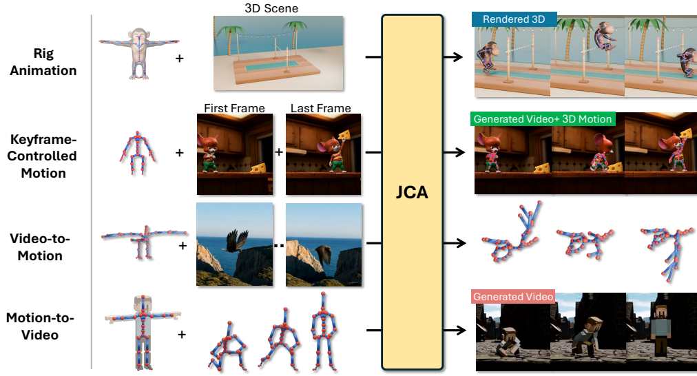
Figure 1: Joints, Camera, Action! (JCA) generates a video and a synchronized 3D motion trajectory for a user-supplied rig of any topology. One model covers joint generation (top two rows) and either conditional direction (bottom two rows). Mesh animation: a rigged monkey clears a scene’s high-jump bar, adapting its motion to the surroundings. Keyframe control: given a first and last frame, JCA fills in the rig motion and video between them. Video-to-motion: recovering 3D motion from an input video. Motion-to-video: video following prescribed 3D motion.
