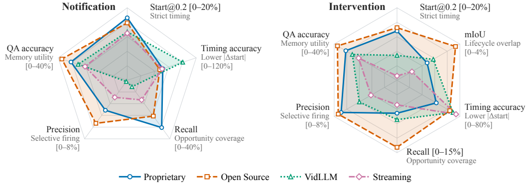
Figure 21: Notification- and intervention-level radar summaries for ProactEgoMem-Sci , task-averaged per model family. Axes and normalization follow Figure 5.
