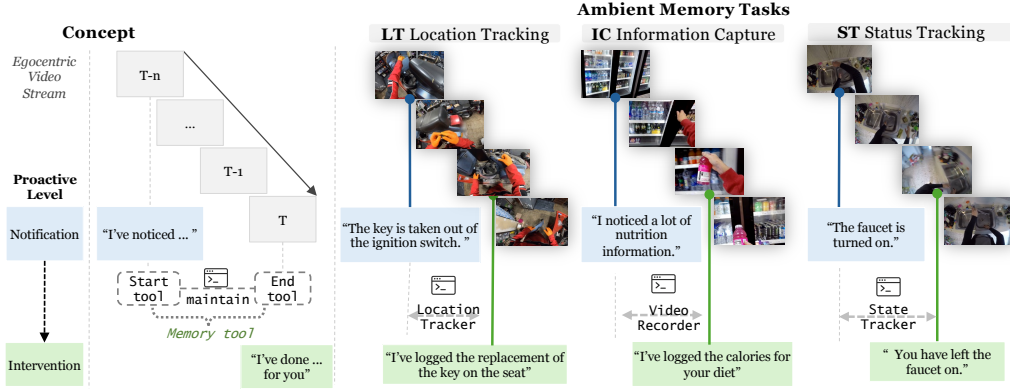
Figure 2: ProactEgoMem measures proactive memory as lifecycle behavior in egocentric streams. At the Notification Level the agent sends one timely message; at the Intervention Level it starts, maintains, and ends a memory tool, and releases a message when the task is completed.
