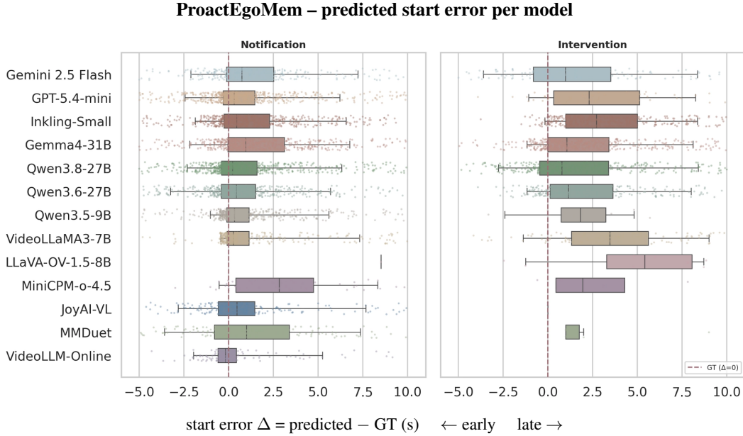
Figure 13: Predicted start-error distributions by model, pooled across the three tasks, for notification and intervention levels. Points are individual matched starts; the dashed vertical line marks the ground-truth boundary, with positive values late and negative values early. Empty intervention rows indicate that no valid matched intervention was available for that model.
