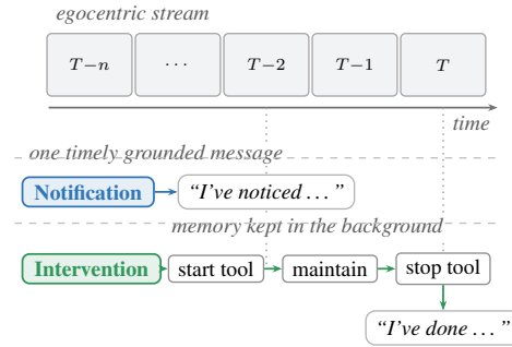
Figure 3: Two-level proactive modes.
