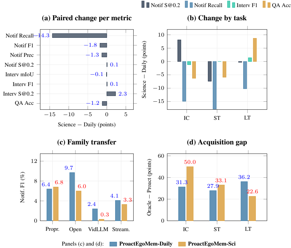
Figure 14: Daily-to-Science transfer over the expanded paired results: 39 model-task cells for notification and intervention, and 36 for QA (VideoLLM-Online excluded). (a) Mean change per metric: only opportunity coverage moves substantially. (b) The same change split by task: the direction reverses between tasks for strict timing, intervention F1, and QA. (c) Notification-level F1 by model family: the open-source lead in daily life does not survive the move to the laboratory. (d) Mean gap between oracle and proactively acquired memory: acquisition costs more in the laboratory on IC and ST, less on LT.
