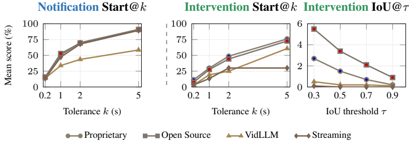
Figure 12: Group-level mean Start@ k and intervention IoU@ \tau over tasks and models as each criterion is relaxed. Note the collapsed scale of the rightmost panel: the best group mean stays below 6%.
