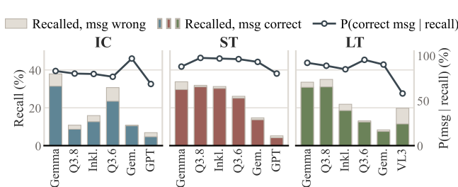
Figure 8: Message accuracy conditioned on recall
