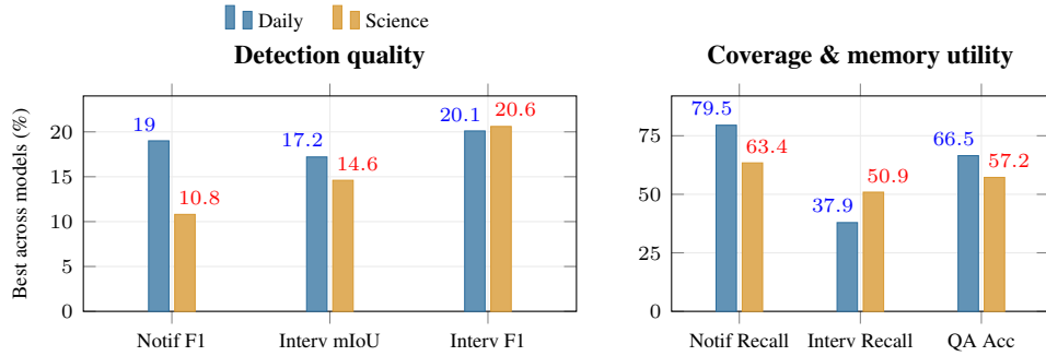
Figure 15: Daily vs. Science, best value across models per metric. Moving to the laboratory lowers notification F1, intervention mIoU, notification coverage, and memory-backed QA. The higher best intervention recall and F1 come from two different single-model LT spikes.
