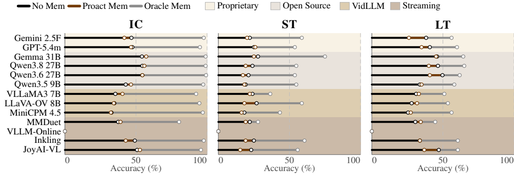
Figure 22: ProactEgoMem-Sci ProactEgoMem-QA performance by task. Each model is shown as a horizontal accuracy bar: black marks No Memory, brown marks Proact Memory, and gray marks Oracle Memory.
