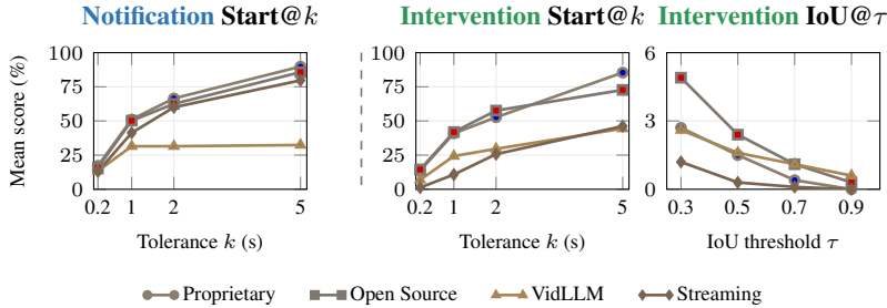
Figure 20: ProactEgoMem-Sci group-level mean Start@ k and intervention IoU@ \tau over tasks and models as each criterion is relaxed. Note the collapsed scale of the rightmost panel: the best group mean stays below 6%.
