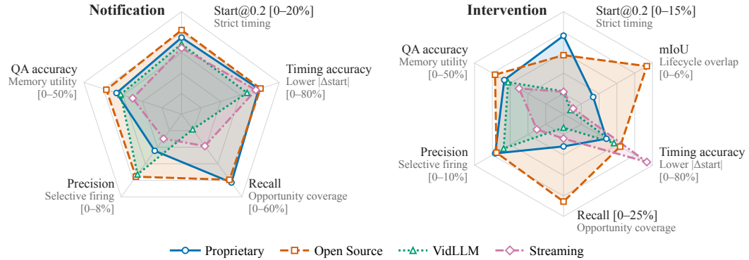
Figure 5: Proactive competence by model family , averaged over the three tasks: proprietary, open-source, video-language, and streaming models on the notification and intervention axes.
