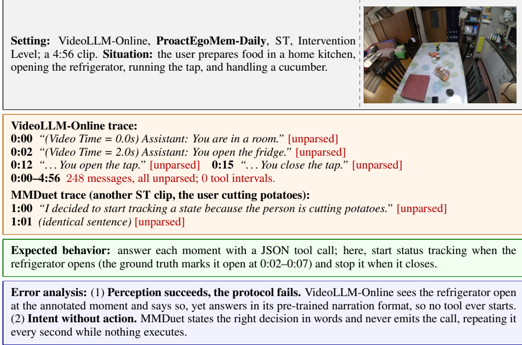
Figure 19: Video-language models fail to follow instructions: VideoLLM-Online narrates and MMDuet describes its decision instead of calling the tool.
