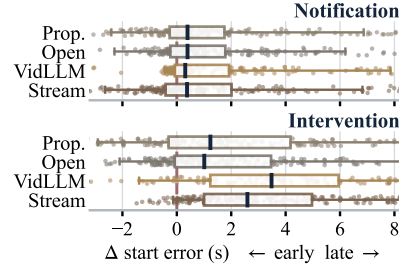
Figure 9: Start error by family
