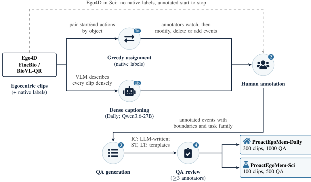
Figure 11: ProactEgoMem construction pipeline. Native labels are greedily paired into candidate events; for Daily, a VLM densely captions every clip in addition to the greedy pairing. Annotators then watch each clip and modify, delete, or add events (Ego4D clips in Sci are annotated from scratch because native labels are missing). Every QA is reviewed by at least three annotators before being finalized.
