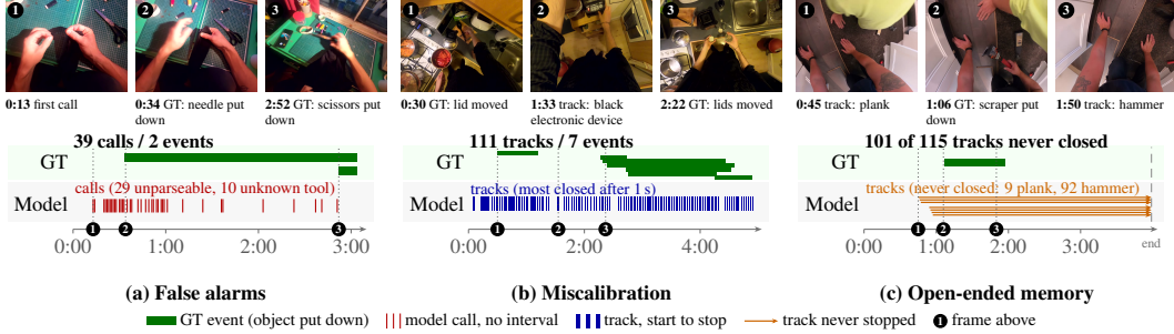
Figure 10: Failure modes on LT clips (Intervention Level): (a) MMDuet, 39 calls for 2 GT events; (b) Gemma4-31B, 111 one-second tracks for 7 events; (c) VideoLLaMA3-7B, tracks never stopped.
