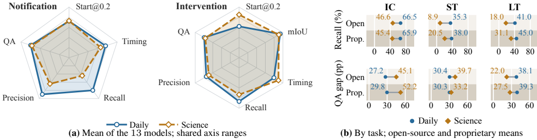
Figure 7: From daily life to the laboratory: (a) the two tracks on the radar axes of Figure 5; (b) notification recall and QA acquisition gap per task.
