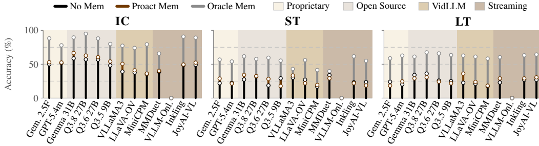
Figure 6: QA accuracy by task. The No-Memory-to-Oracle gap is the acquisition headroom.
