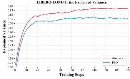
(a) LIBERO-LONG critic explained variance.
