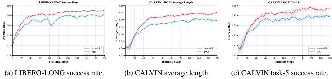
Figure 6: Training curves on LIBERO-LONG and CALVIN ABC-D.
