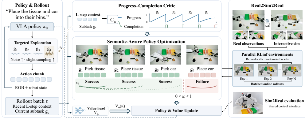
Figure 2: Overall pipeline of AtomicRL. (a) Progress–Completion Critic: PCC identifies atomic task boundaries and estimates atomic task progress from interaction histories. (b) Semantic-Aware Policy Optimization: SAPO uses these signals to regulate cross-subtask advantage propagation based on subtask execution outcomes. (c) Bottleneck-Adaptive Targeted Exploration: BATE adapts task sampling and local exploration according to subtask mastery, focusing training on insufficiently mastered bottleneck subtasks. (d) Real2Sim2Real workflow: A complementary Real2Sim2Real pipeline enables parallel simulation-based training and transfer to real-world robots.
