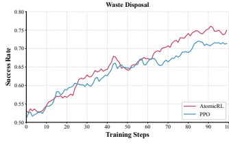
(b) WD success rate.
