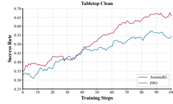
(c) TC success rate.
