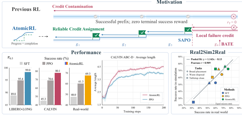
Figure 1: Overview of AtomicRL. Unlike previous RL methods that use standard GAE which may suffer from credit contamination, AtomicRL uses SAPO to promote more reliable credit assignment. Together with BATE and the Real2Sim2Real pipeline, AtomicRL achieves strong performance on long-horizon manipulation tasks in both simulation and the real world.
