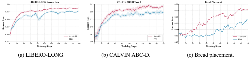
Figure 4: Training curves on LIBERO-LONG and CALVIN ABC-D and Real-World(BP).
