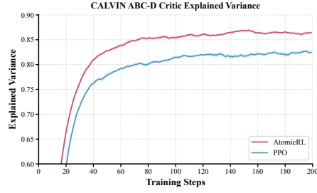
(b) CALVIN critic explained variance.
