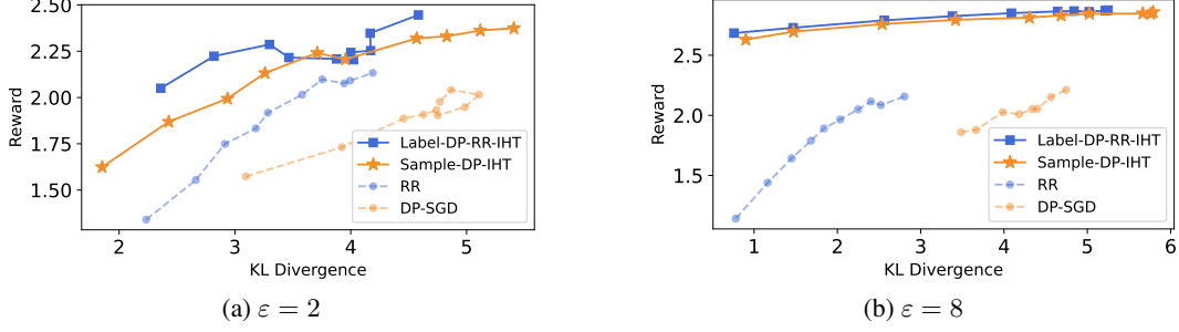
Figure 1: IMDb Sentiment Generation with Llama-7B under different privacy budgets ( \varepsilon ).
