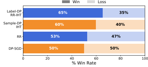
Figure 4: Safety Alignment with Gemma-3-1B ( \varepsilon = 2 ).
