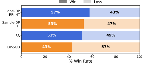
Figure 4: Safety Alignment with Gemma-3-1B ( \varepsilon = 2 ).
