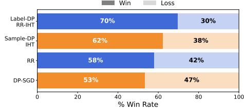
Figure 2: Safety Alignment with Gemma-3-1B ( \epsilon = 8 ).
