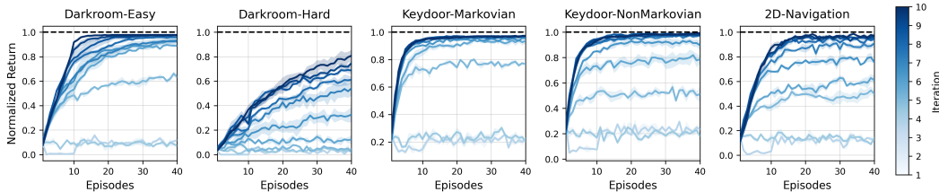
Figure 19: The test-time efficiency of ASTEROID increases significantly with more iterations of asymmetric on-policy distillation, demonstrating that as the context dataset grows, the policy can adapt over longer horizons, making exploration more efficient.
