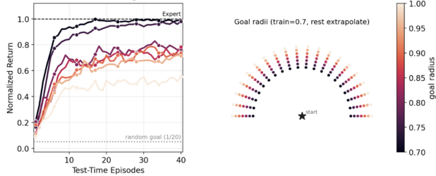
Figure 20: Generalization under shifted latent priors in 2D Navigation. Training goals lie at radius 0.7; evaluation goals are sampled at increasing radii up to 1.0. Performance degrades gradually with shift magnitude.
