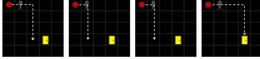
(a) The agent finds the key in earlier episodes, can reference it back in its context, and always picks up the key before searching for the door.
