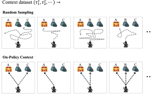
Figure 25: On-policy contexts ensure efficient coverage over relevant histories, while random exploration [42] can generate uninformative contextual information that harms training.
