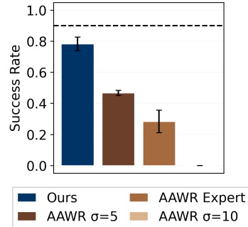
Figure 14: ASTEROID generates data online, while AAWR is sensitive to the quality of offline datasets.
