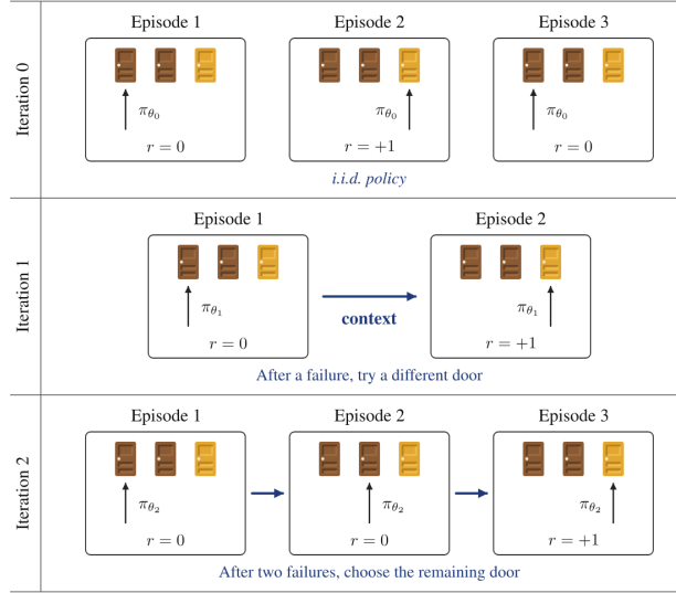
Figure 4: We iteratively learn to adapt exploration using feedback over longer contexts.
