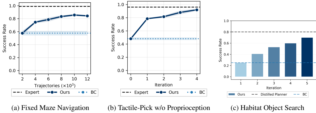
Figure 16: ASTEROID learns to solve POMDPs such as maze navigation, robot manipulation, and Habitat object search, where agents must act under limited fields of view, random resets, and partial sensing.
