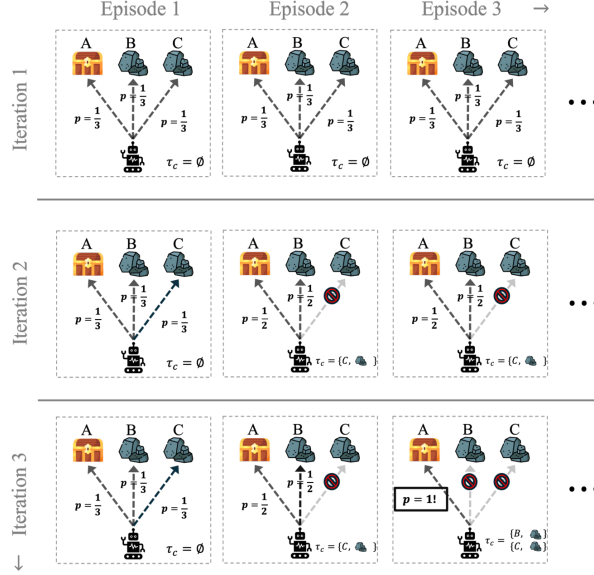
Figure 24: Toy example demonstrating that ASTEROID learns adaptive in-context behavior, where it effectively explores based on history.
