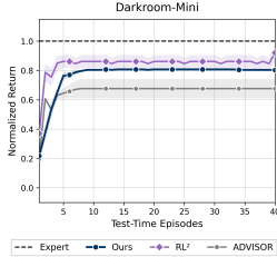
Figure 18: RL is effective over short horizons, but ASTEROID uses supervised updates to be effective across long-horizon tasks as well.
