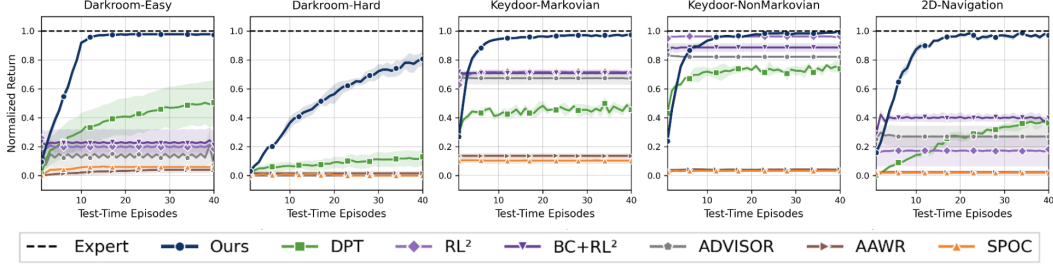
Figure 6: Performance on discrete exploration tasks requiring memory and goal inference. We observe that ASTEROID outperforms all baselines in terms of test-time efficiency. It performs efficient exploration and almost converges to the expert after inferring the hidden task variables.
