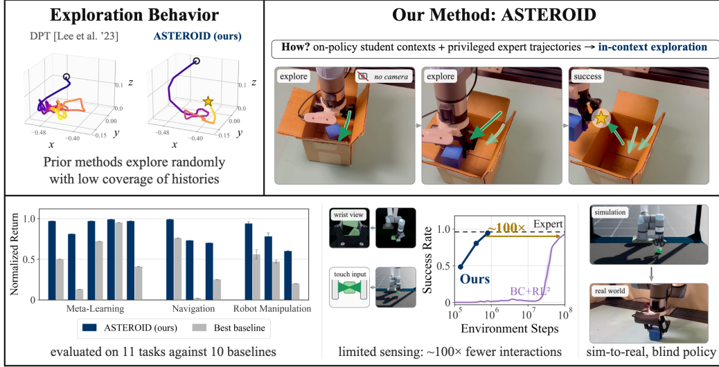
Figure 1: ASTEROID provides a simple and reliable method for learning efficient exploration in partially observed domains via on-policy asymmetric student-teacher distillation.
