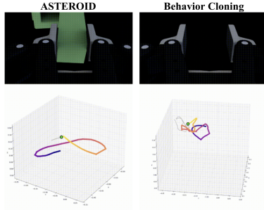
Figure 10: Robot positions (bottom row) during exploration for Peg-Insertion from wrist images (top row). ASTEROID learns policies that sweep the table to locate the peg and successfully place it in the hole, whereas direct imitation policies collapse under limited observability.
