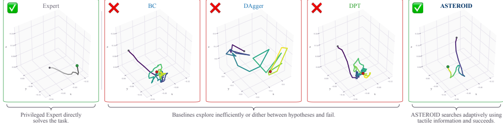
Figure 9: End-effector trajectories on the tactile cube-pick task, where the policy must locate and lift a cube using proprioception and touch sensing. The privileged state expert (gray) observes the cube pose and grasps it directly. Under partial observability, the baselines fail to adapt their actions, whereas ASTEROID performs in-context exploration, exploring the table until contact, then grasping and lifting the cube.
