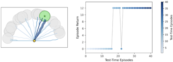
Figure 21: In 2D navigation, ASTEROID adapts its exploration based on context, converging to the true goal.
