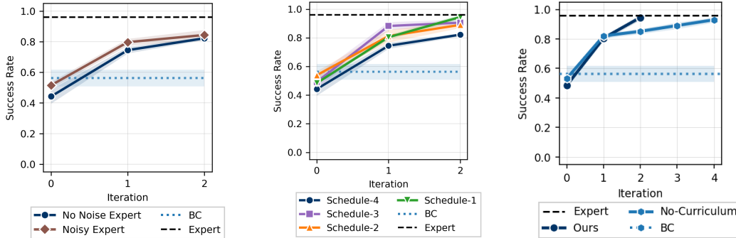
Figure 17: We run ablations on different parts of ASTEROID in the Tactile-Pick task. Left: we run ASTEROID with a noisy expert and observe no performance drop. Middle: we sweep over different curricula with increasing exploration horizons and find minimal sensitivity. Right: we show that adding curriculum improves the efficiency of ASTEROID by ensuring that as the horizon increases over iterations, the learned policy does not suffer from OOD histories or generating random actions.
