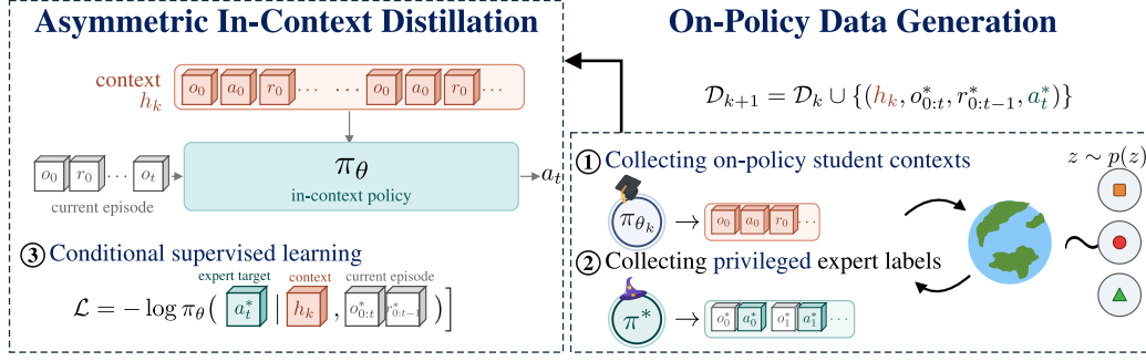
Figure 3: In each iteration, ASTERIOD (1) collects on-policy context from the student \pi_{\theta_k} and then (2) expert trajectories from \pi^* , under the same hidden parameters z . With this dataset, we can (3) train policies that perform in-context exploration.
