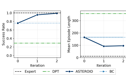
Figure 7: ASTEROID improves success while reducing episode length on Procgen Maze; BC succeeds non-trivially via random exploration but is much less efficient.
