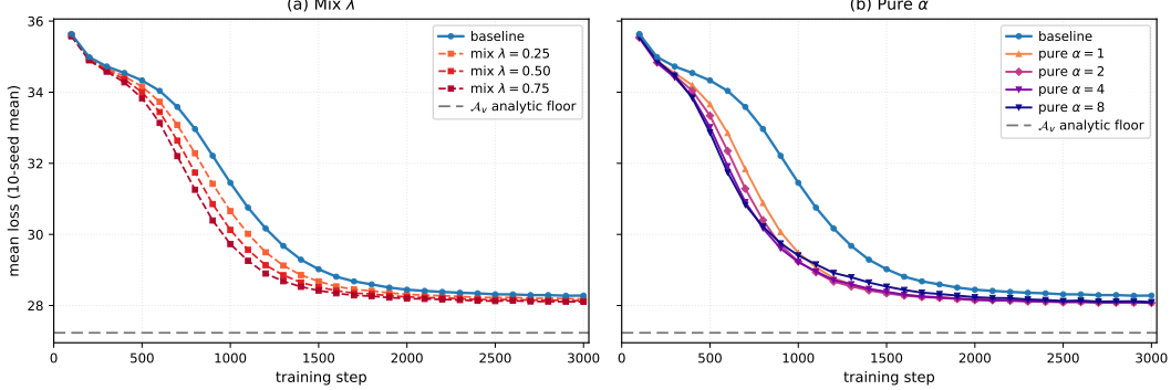
Figure 3: Sampler-side t -sampler interventions on a controlled d = 16 , K = 32 GMM. Ten-seed mean loss for the baseline and gap-guided samplers using a proxy source disjoint from the paired test. Gap arms lie below baseline past the peak-learning step; pure \alpha = 2 is lowest at the plateau, while pure \alpha = 4 is lowest near the peak-learning step.
