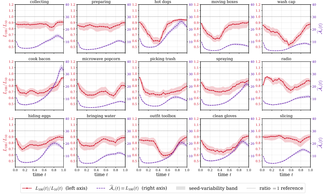
Figure 8: Per-task ratio profiles and large-budget reference profile on BEHAVIOR-1K. Each panel shows one leakage-free trio from the fifteen-task BEHAVIOR-1K diagnostic panel over multiple demonstration seeds. The left axis plots the per-bin ratio L_{100}(t)/L_{10}(t) with the ratio = 1 reference line; the right axis plots the large-budget reference profile L_{100}(t) , which is an upper-biased proxy for \mathcal{A}_v(t) rather than an absolute Bayes-floor estimate. All fifteen trios improve in mean loss from N = 10 to N = 100 , but the temporal location of improvement is task-dependent.
