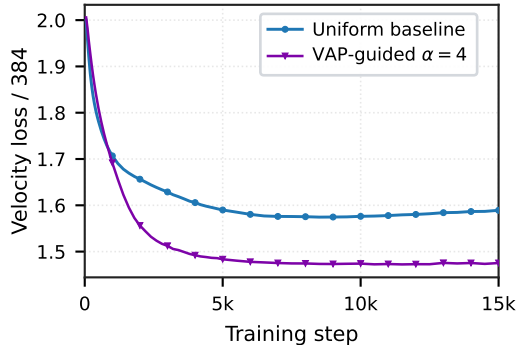
Figure 4: Uniform-time evaluation during DINOv2 feature-flow training. The gap-guided sampling lowers uniformly evaluated velocity loss. Curves show means over five paired training seeds.
