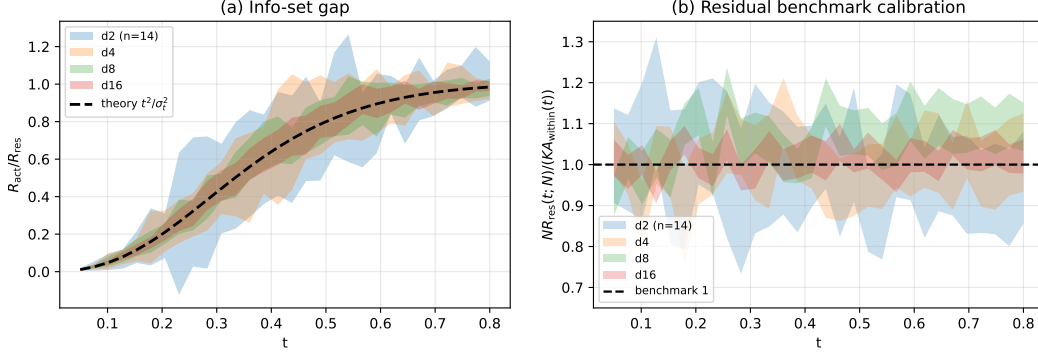
Figure 5: Info-set decomposition and residual benchmark calibration. (a) The empirical ratio R_{\text{act}}(t; N)/R_{\text{res}}(t; N) from a closed-form ablation ( N=2000 , K=4 , \sigma=0.5 , no MLP) collapses onto the analytic curve t^2/\sigma_t^2 (dashed) across d \in \{2, 4, 8, 16\} . (b) The residual-regression oracle, normalized as NR_{\text{res}}(t; N)/(K\mathcal{A}_{v,\text{within}}(t)) , is centered at the unit benchmark from Theorem 5. All scalar summaries in the text use the full 20-seed run for every d . Panel (a) shows seed-level spread for the ratio readout, while panel (b) shows standard error around the mean for residual calibration. Together these panels show that the label-and-action oracle is strictly tighter at small t , while the residual oracle is calibrated to the theorem’s sharp residual-regression benchmark.
