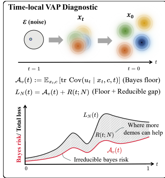
Figure 1: Velocity ambiguity profiles localize where flow matching needs data. The flow matching path defines a continuum of velocity prediction problems. VAP separates the irreducible ambiguity floor from the reducible excess error that more data or a different estimator can affect.
