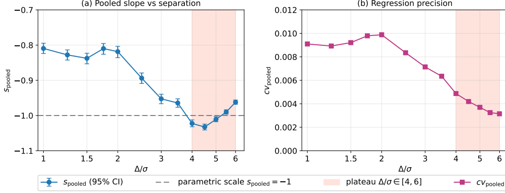
Figure 2: Canonical d=4 dense controlled transition on a K=4 , \sigma=0.5 Gaussian mixture. The 13-row front/plateau window shows the reliability-filtered signed log-log slope s_{\text{pooled}} = \partial \log \hat{R} / \partial \log N and regression precision; the shaded band marks \Delta/\sigma \in [4, 6] , where s_{\text{pooled}} \approx -1 , equivalently the positive exponent \alpha_{\text{pooled}} = -s_{\text{pooled}} \approx 1 . Full rows and filter sensitivity are in Appendix D.3.
