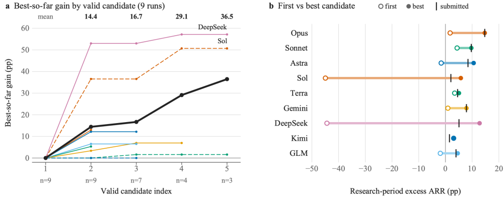
Figure 5 Research-period progress of the nine iterative runs. (a) Best-so-far excess ARR gain over the first valid candidate; means use the runs available at each index. (b) First, best, and committed candidates on 2022–2023.
