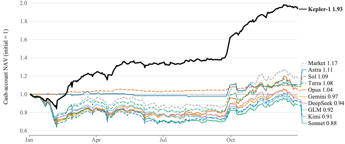
Figure 7 Cash-account NAV in 2024 for the nine models’ best iterative configurations and Kepler-1, against the gross equal-weight market.
