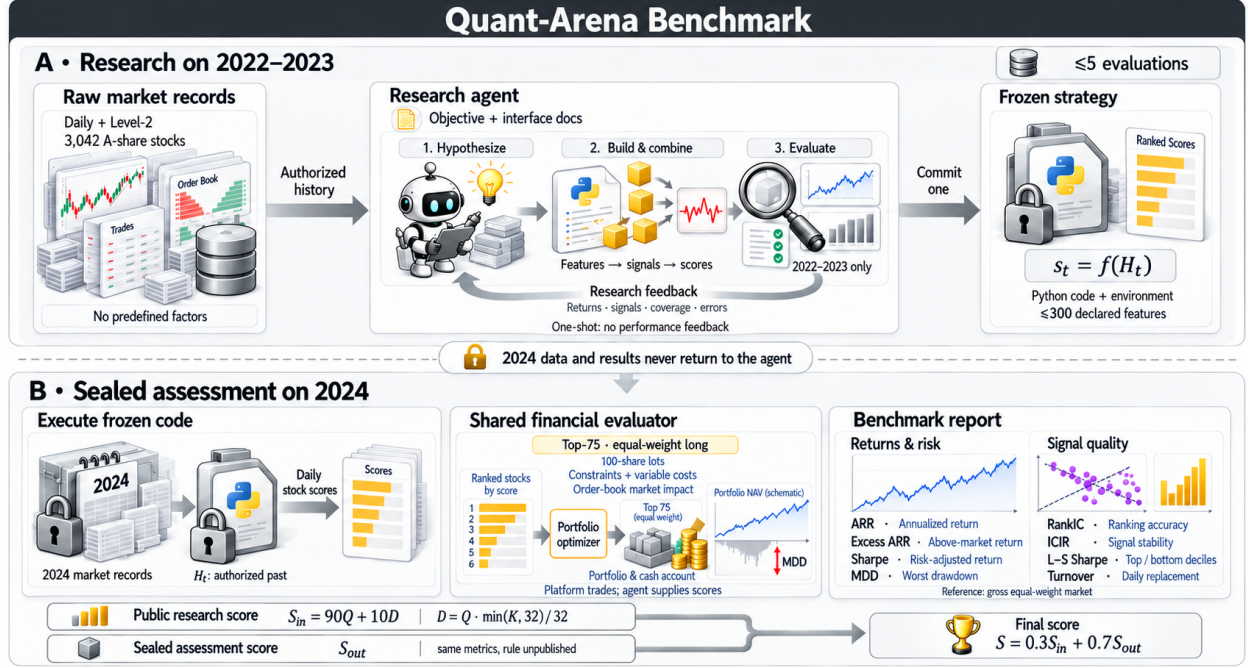
Figure 2 A model constructs features and stock-scoring code from raw market observations, revises candidates using research-period feedback, and freezes one strategy for assessment on the sealed period under common portfolio and execution rules.
