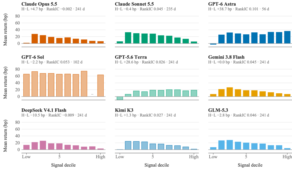
Figure 3 Mean next-day return by daily score decile for the nine models’ best iterative configurations in 2024, in basis points (bp). H-L is the highest-minus-lowest decile spread, and the last entry in each header is the number of days with a signal.
