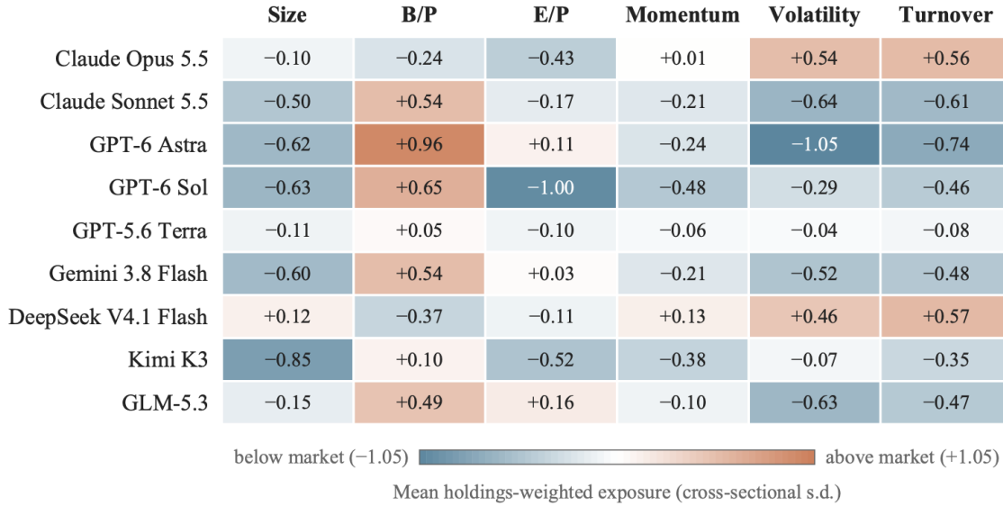
Figure 6 Holding-value-weighted style exposure of the nine models' best iterative configurations in 2024, in cross-sectional standard deviations relative to the market. Astra's estimates use its 61 invested days.
