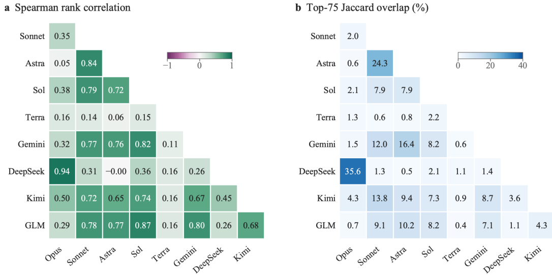
Figure 8 Pairwise mean daily Spearman signal correlations (a) and Top-75 Jaccard overlaps (b) among the nine models' best iterative configurations in 2024 (36 pairs). Portfolio overlap measures the selected score sets, rather than identical realized trades under execution constraints.
