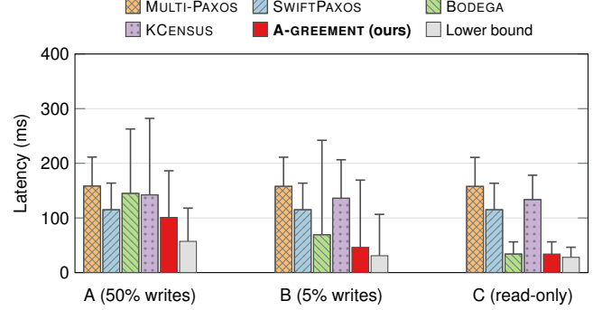
Figure 5: Failure-free latency averaged with equal weight over the six deployments with 5 or 9 replicas. Bars report mean latency, while upper whiskers report p99 latency. Lower bound is the idealized communication baseline.
