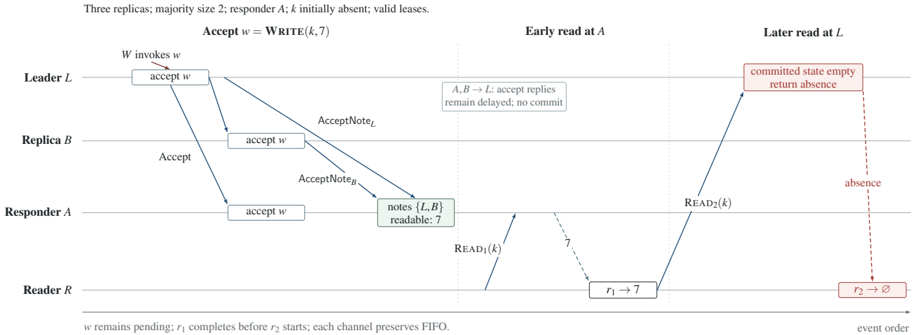
Figure 13: Counterexample to Bodega's early-accept read optimization. All replicas accept w , but delayed acceptance replies prevent L from committing it. Accept notifications let A return 7, while a subsequent read at L returns absence.
