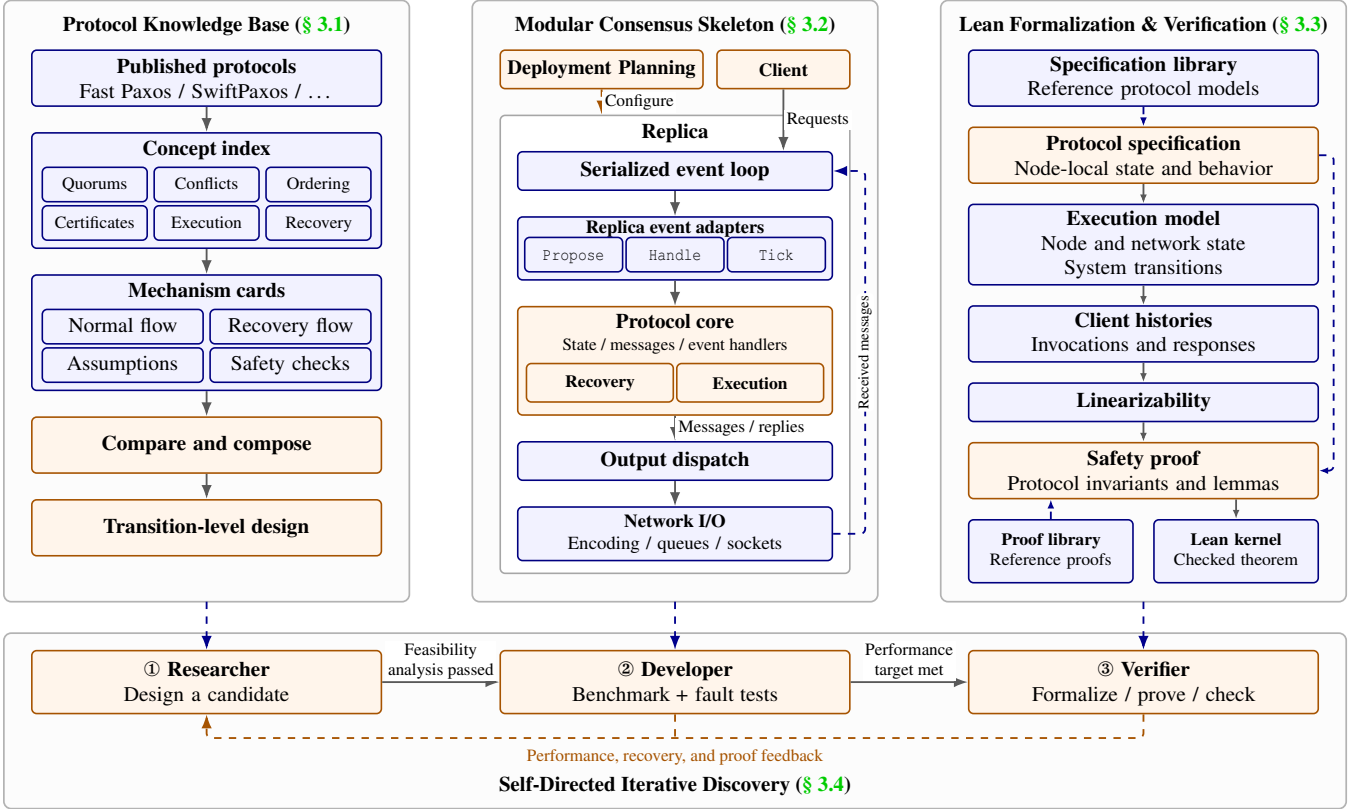
Figure 3: AI-GREEMENT harness architecture. Blue components provide reusable knowledge, interfaces, execution semantics, and proof support; orange components contain protocol-specific logic supplied by the agent. In the verification column, protocol specifications and proofs build on a shared execution model and linearizability definition.
