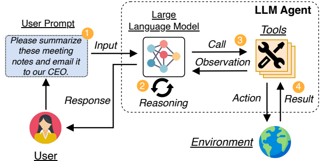
Figure 1: The workflow of an LLM agent.
