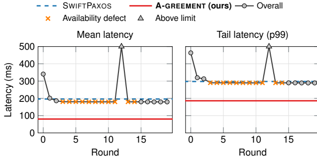
Figure 2: Mean and tail (P99) latency of discovered consensus protocols across 20 search iterations, using the original CODEX harness and the GPT-6.1 Sol model (with high reasoning effort).
