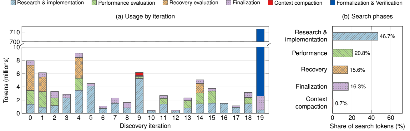
Figure 7: Stage-attributed token usage, including input and output tokens. (a) Per-iteration usage in millions of tokens, with a broken axis omitting the range from 10 to 700 million. Formalization and verification adds 710.31 million tokens at iteration 19. (b) Phase shares within the search, excluding formalization and verification.
