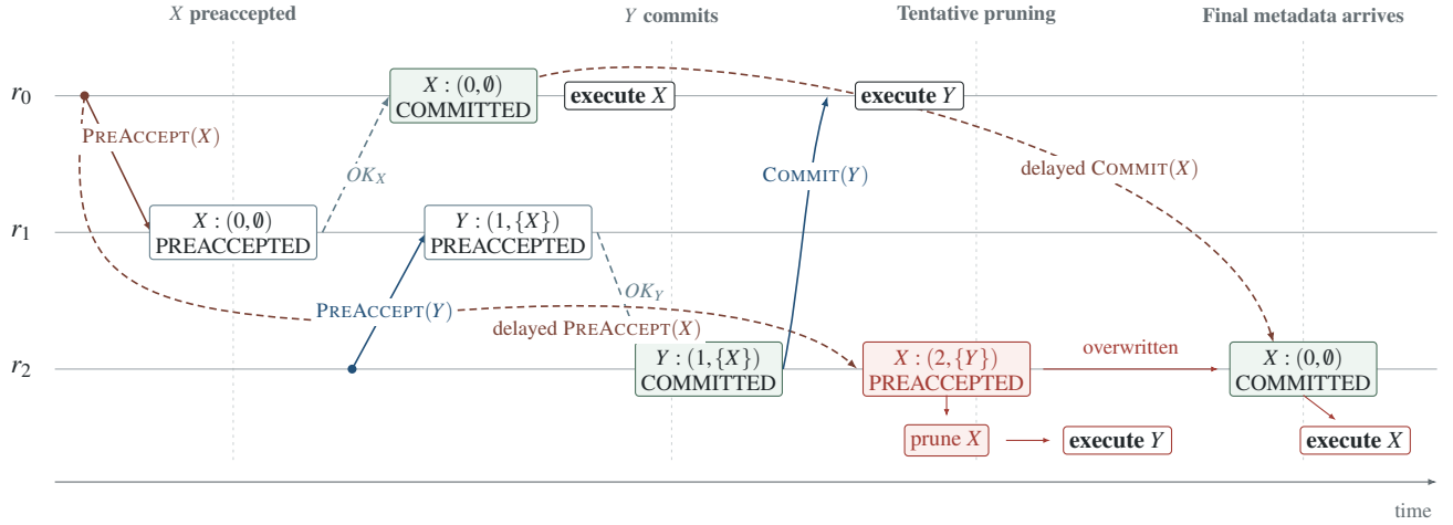
Figure 11: Pruning with tentative metadata reverses conflicting command order: r_0 executes X before Y , while r_2 prunes X using its tentative tuple and executes Y before X .
