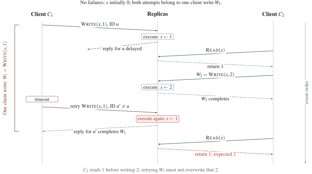
Figure 14: A Bodega client retry can repeat a write that has already taken effect. The first attempt sets x = 1 , but its reply is delayed. After C_2 reads 1 and completes a write of 2, a retry with a new identifier overwrites x with 1. If both attempts represent one client write, the final read must return 2.
