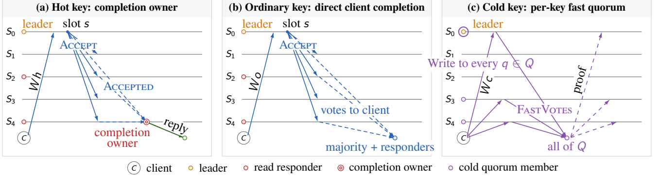
Figure 4: Message propagation in A-GREEMENT on the hot (left), ordinary (middle) and cold write (right) paths.
