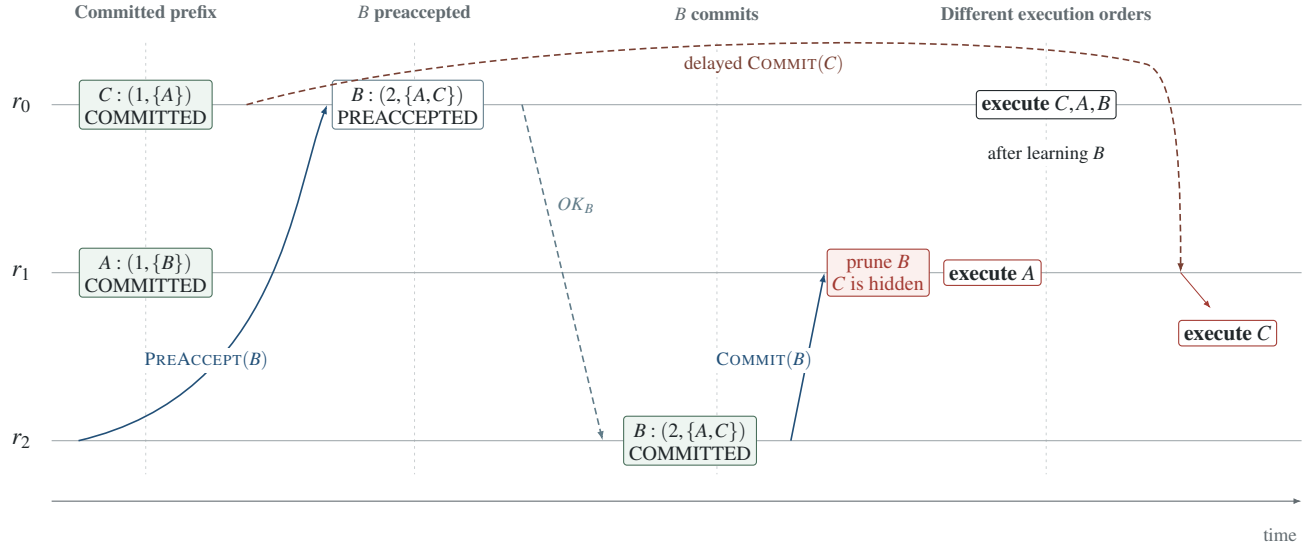
Figure 12: Pruning committed B hides C , allowing r_1 to execute A before C while r_0 executes C before A .
