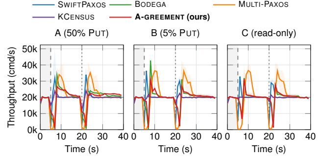
Figure 6: Recovery throughput with five replicas under workloads A, B, and C (left to right). Lines show mean completed requests per second across three topologies; bands show their minimum–maximum range.
