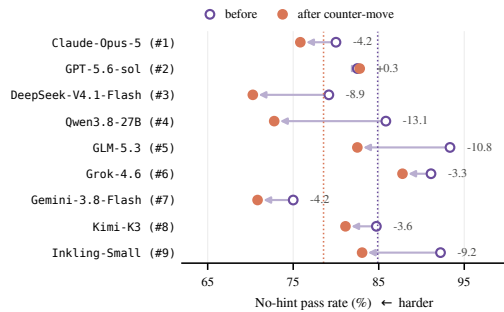
Figure 4: Pass rate before and after the counter-move. Stronger solvers improve less.
