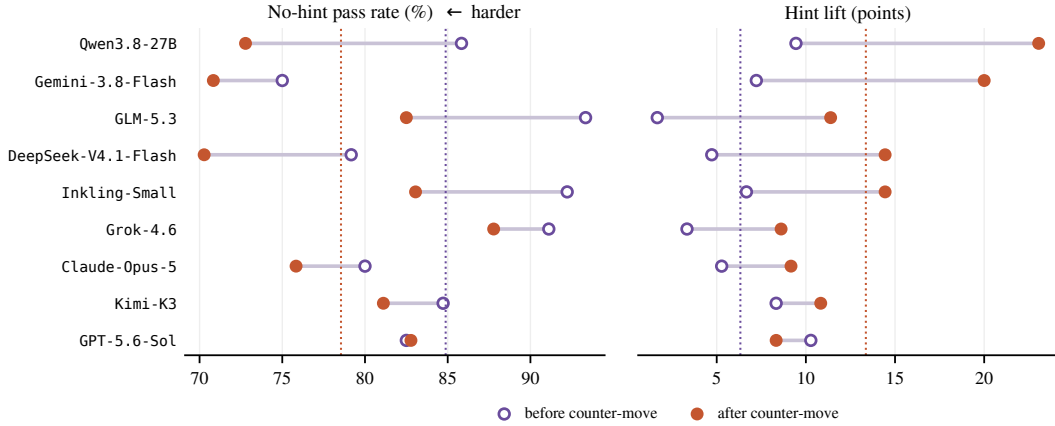
Figure 6: Before and after the counter-move. Each author’s no-hint pass rate (left, lower is harder) and hint lift (right), before (open) and after (filled) its counter-move; dotted lines mark the averages over all authors. Authors are ordered by their gain in hint lift.
