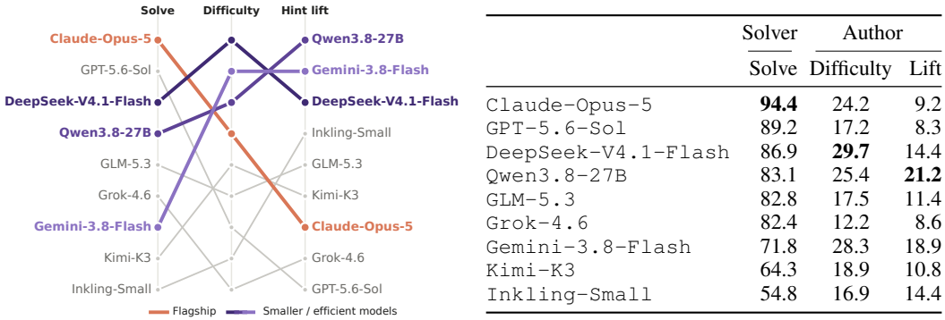
Figure 2: Overall ranking in Environment Duels. Each model’s rank on Solve, Difficulty and Hint lift, with the underlying scores (best in bold). The strongest solvers lead Solve, while three smaller models lead both authoring axes. Difficulty is the no-hint fail rate of all nine solvers on the model’s environments, and Hint lift is in points; hint-lift ties are broken by solve rank.
