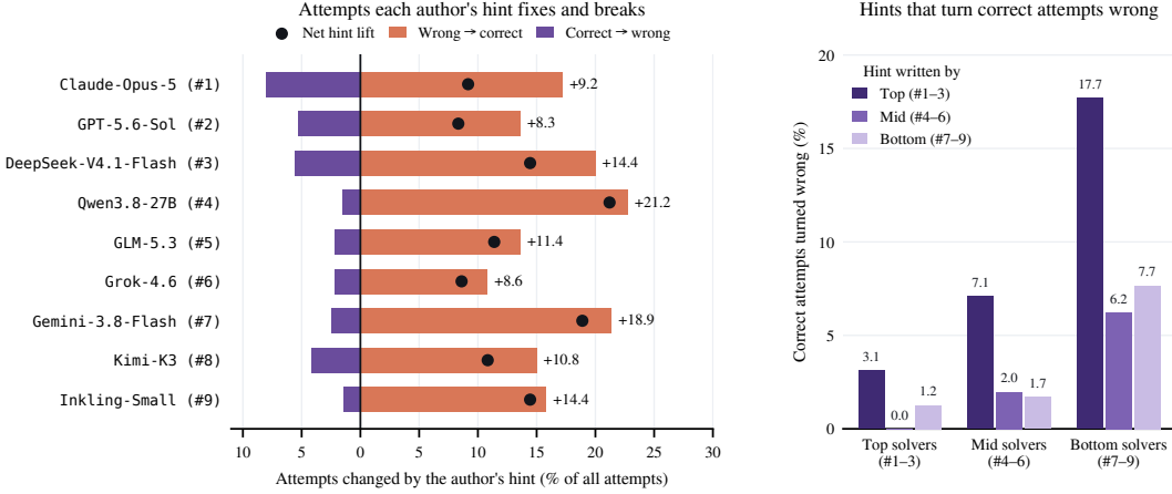
Figure 3: The best teacher is not the best solver. Left: attempts each author’s hint fixes (orange) and breaks (purple); a mid-ranked solver writes the most useful hints. Right: the breaks come from strong authors’ hints reaching weak solvers, while strong solvers are almost never harmed.
