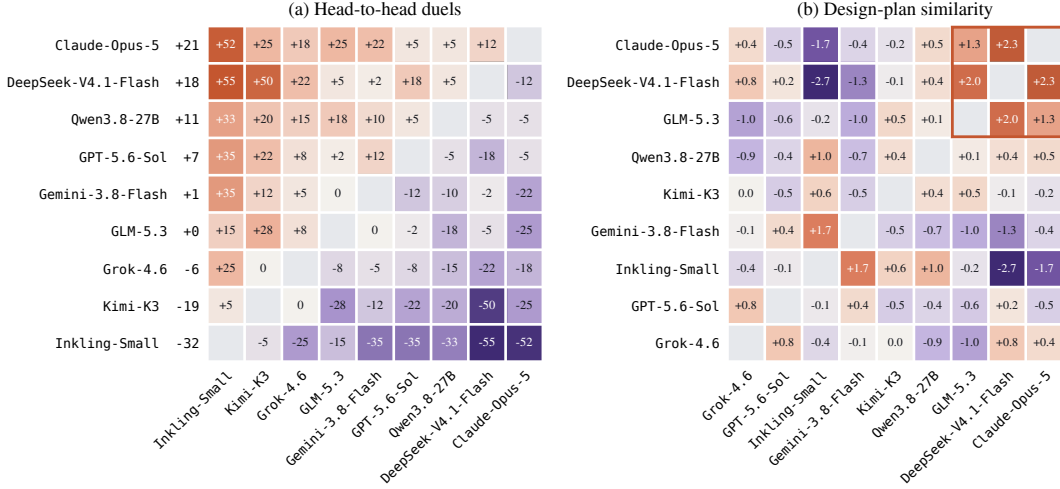
Figure 5: What the duel matrix shows beyond the scores. (a) Duels give a stable ranking: each cell is the row model’s pass rate on the column model’s environments minus the reverse (points), orange means the row model wins, and no model loses to one ranked below it. (b) Some authors design alike: each cell is how much more alike two authors’ design plans are than their general similarity predicts ( \times 100 ), and Claude-Opus-5, DeepSeek-V4.1-Flash and GLM-5.3 form the one clear cluster (outlined).
