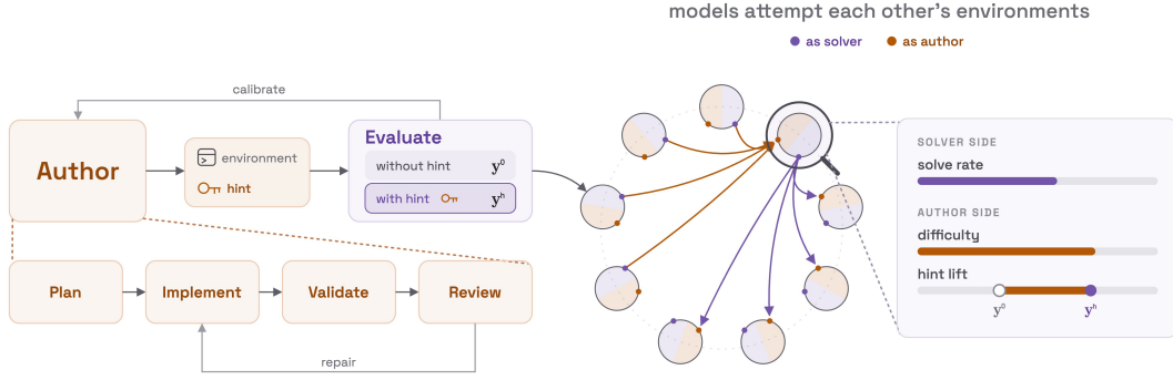
Figure 1: Overview of Environment Duels. Frontier LLMs create and solve each other’s environments. These interactions form a microcosm of the real-world model ecosystem.
