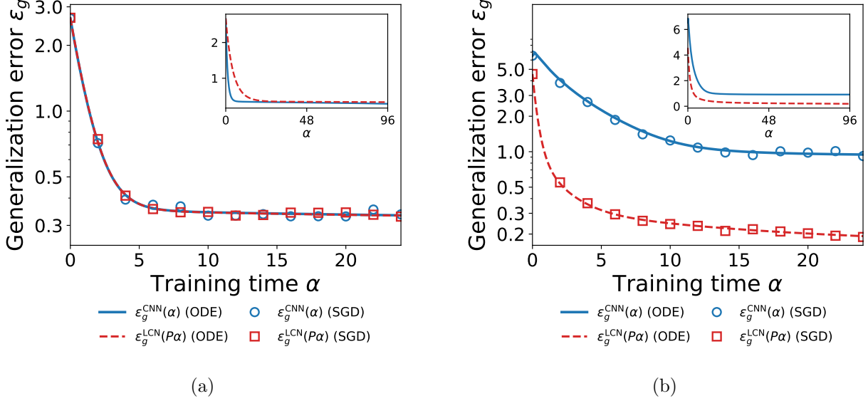
Figure 2: Generalization errors \varepsilon_g^{\text{CNN}}(\alpha) of the CNN and \varepsilon_g^{\text{LCN}}(P\alpha) of the LCN. Lines are the order-parameter ODEs and symbols mark simulations of a single SGD trajectory. Insets show the ODE curves without the time rescaling. (a) For independent positions ( c = 0 ) the trajectories coincide. (b) In the presence of spatial correlations ( c = 0.5 ) the rescaling fails and the LCN converges faster (see inset). Parameters: g = \text{erf} , k_t = 2 , k_s = 3 , P = 4 , \eta = 1 , \sigma = 0 , T = 1 , SGD at D = 1000 .
