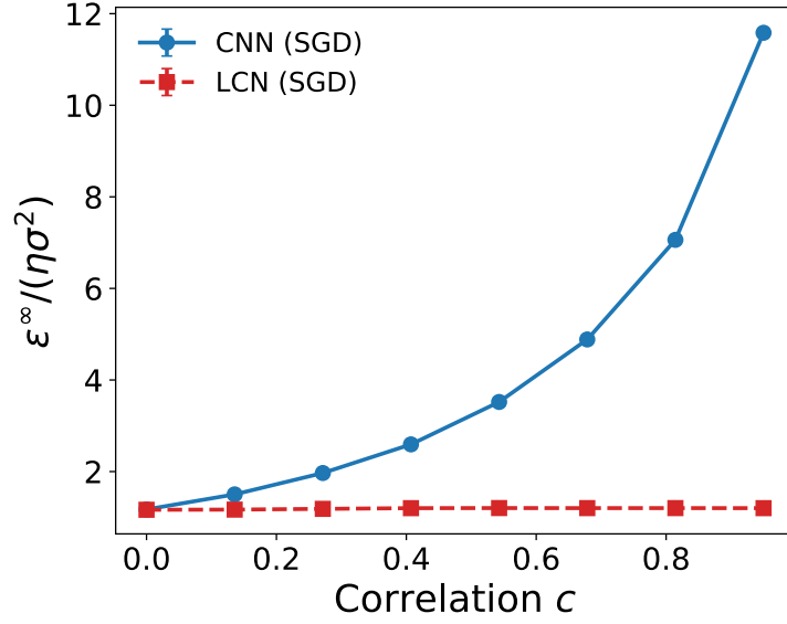
Figure 10: Rescaled noise floor \varepsilon^\infty/(\eta\sigma^2) of the two students with the ReLU activation, where \varepsilon^\infty is the asymptotic generalization error under label noise. It is measured by online SGD from the specialized initial condition and averaged over seeds, with the generalization error computed exactly from the student weights. Standard errors are smaller than the marker size. As for erf (Figure 5), the CNN's floor grows with the data correlation c while the LCN's stays flat. Parameters: g(z) = \max(0, z) , k_s = k_t = 2 , P = 4 , D = 400 , \eta = 0.1 , T = 1 , \sigma = 1 , runs up to \alpha = 800 , 8 seeds.
