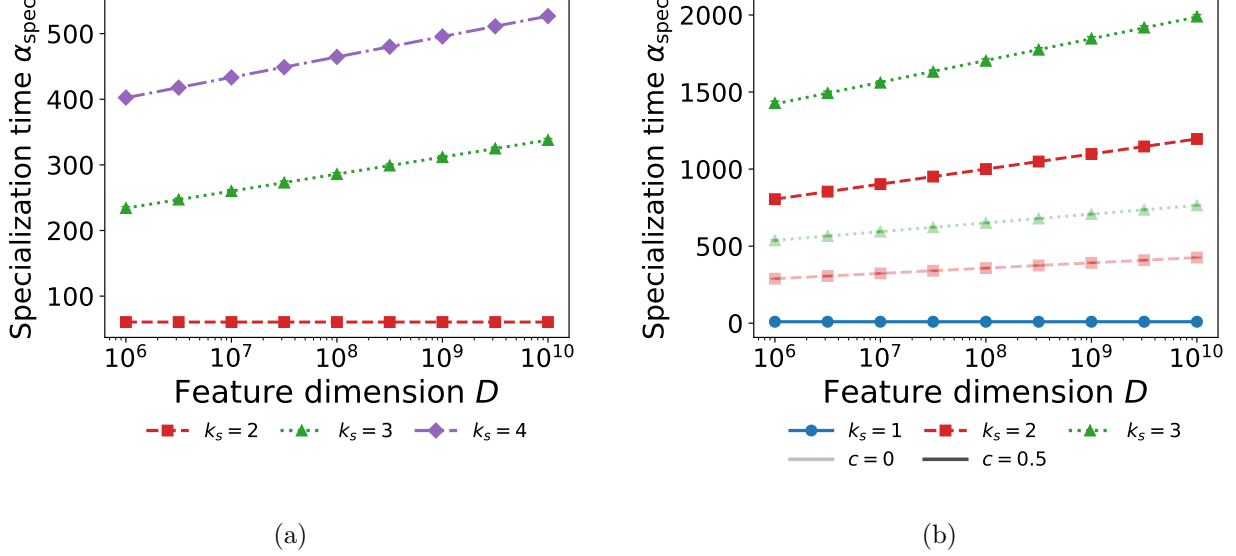
Figure 7: Specialization time of the CNN against the feature dimension, as in Figure 3b. Color denotes the student kernel size. Markers are averages over random initializations, each obtained by integrating the ODEs (17) from the order parameters of a random initialization at dimension D . Standard errors are smaller than the marker size. Lines are fits a + b \ln D . (a) A teacher of kernel size k_t = 2 . The matched case k_s = k_t = 2 is flat in D and the two wider kernels grow logarithmically. (b) Correlated positions, at k_t = 1 , with c = 0 faded and c = 0.5 at full strength. The plateau at k_s > k_t survives the correlation. Parameters: g = \text{erf} , P = 6 , \eta = 0.5 in panel (a) and \eta = 0.2 in panel (b), T = 1 , \sigma = 0 , c = 0 in panel (a), D from 10^6 to 10^{10} , 128 random initial conditions.
