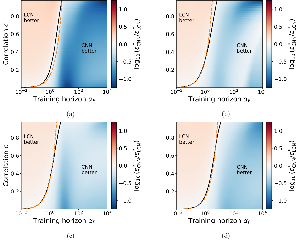
Figure 9: Phase diagram of Figure 6 for other parameter values. The color shows \log_{10}(\epsilon_{\text{CNN}}^*/\epsilon_{\text{LCN}}^*) on a common scale. Solid line: boundary \epsilon_{\text{CNN}}^* = \epsilon_{\text{LCN}}^* , obtained by integrating the ODEs numerically. Dashed line: analytical prediction c = c_0 \alpha_F of the early-time expansion, Eq. (30). Each panel changes one parameter of Figure 6: (a) P = 8 , (b) k_s = k_t = 2 , (c) T = 2 , (d) \sigma = 2 . Other parameters: g = \text{erf} , P = 4 , k_s = k_t = 1 , T = 1 , \sigma = 1 , random initial condition in the limit D \rightarrow \infty .
