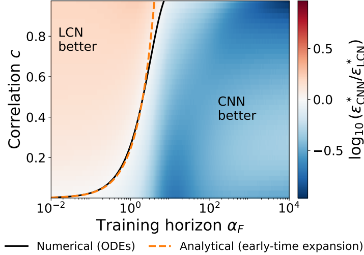
Figure 6: Comparison of the CNN and the LCN at training horizon \alpha_F and correlation c , each at its optimal constant learning rate. The color shows the log-ratio of the errors \varepsilon^* . Solid line: boundary \varepsilon_{\text{CNN}}^* = \varepsilon_{\text{LCN}}^* , obtained by integrating the ODEs numerically. Dashed line: analytical prediction Eq. (30) of the early-time expansion. Parameters: g = \text{erf} , P = 4 , k_s = k_t = 1 , T = 1 , \sigma = 1 , random initial condition in the limit D \rightarrow \infty .
