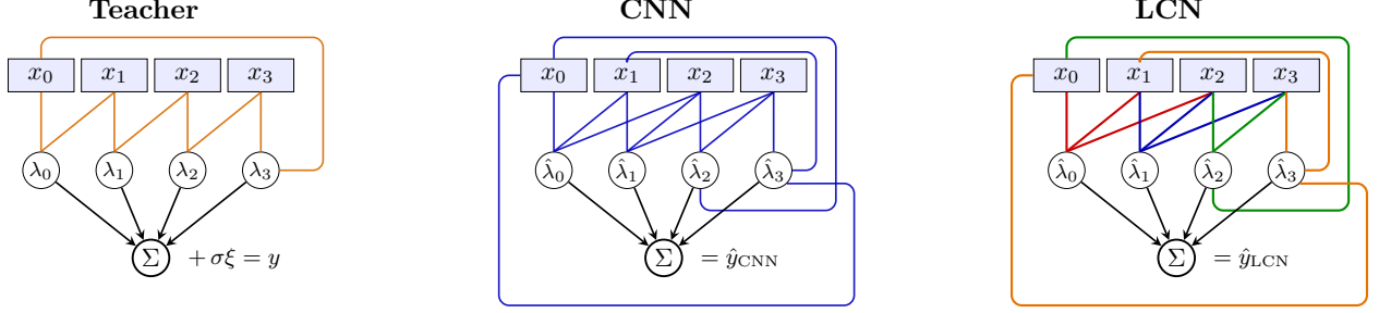
Figure 1: Teacher and the two student architectures with P input positions. Colors indicate weight sharing. The teacher is a two-layer CNN with kernel size k_t . The CNN student has kernel size k_s and weight sharing. The LCN has the same receptive fields as the CNN but no weight sharing. Boundary conditions are cyclic. Here, P = 4 , k_s = 3 , and k_t = 2 .
