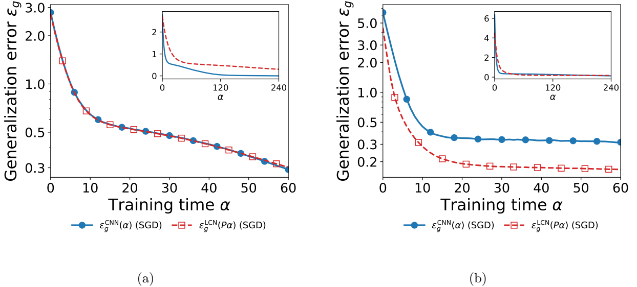
Figure 11: Rescaling test of Figure 2 with the ReLU activation. Generalization errors \varepsilon_g^{\text{CNN}}(\alpha) of the CNN and \varepsilon_g^{\text{LCN}}(P\alpha) of the LCN, from online SGD averaged over 16 runs per student. Standard errors are smaller than the marker size. Insets show the curves without the time rescaling. (a) c = 0 . (b) c = 0.5 . Parameters: g(z) = \max(0, z) , k_t = 2 , k_s = 3 , P = 4 , \eta = 0.2 , \sigma = 0 , T = 1 , D = 1000 .
