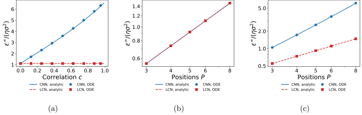
Figure 5: Asymptotic noise floor \varepsilon^\infty/(\eta\sigma^2) of the CNN and the LCN at kernel size k_s = k_t = 2 , as a function of the data correlation c and the number of positions P , where \varepsilon^\infty is the asymptotic generalization error under label noise. Lines are the closed forms (31) and (32) and markers are the noise floors located numerically from the order-parameter ODEs at finite learning rate. (a) Floor vs. c at P = 6 . The CNN grows steeply with c while the LCN stays flat. (b) Scaling with P at c = 0 . The CNN and the LCN coincide and are both linear in P . (c) Scaling with P at c = 0.5 . The LCN is still linear in P while the CNN grows quadratically. Parameters: g = \text{erf} , k_s = k_t = 2 , \eta = 2 \times 10^{-3} , \sigma = 1 , T = 1 .
