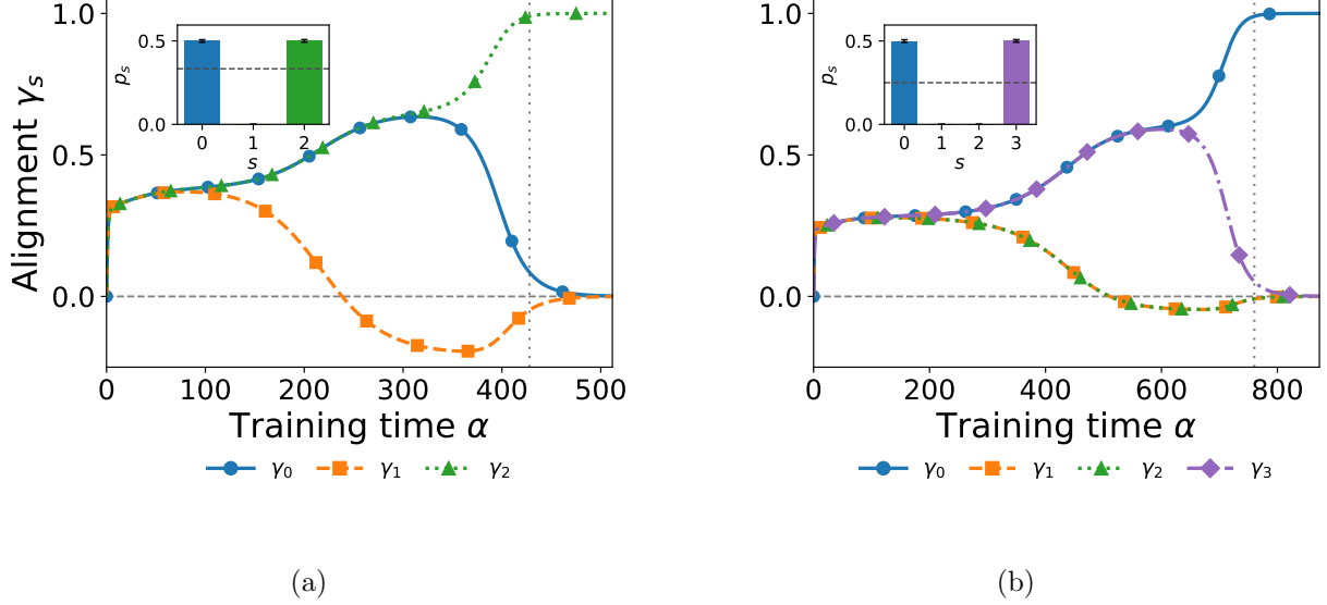
Figure 4: Alignment \gamma_s of the CNN kernel with the solution s vs. training time \alpha , for (a) k_s = 3 and (b) k_s = 4 . The dotted line marks the specialization time \alpha_{\text{spec}} and the dashed line \gamma_s = 0 . Insets: probability p_s that solution s is selected, over 4096 random initial conditions (dashed line: uniform). All curves are solutions of the ODEs (17). Parameters: D = 10^{12} , g = \text{erf} , k_t = 1 , P = 6 , S = I , \eta = 0.5 , T = 1 , \sigma = 0 .
