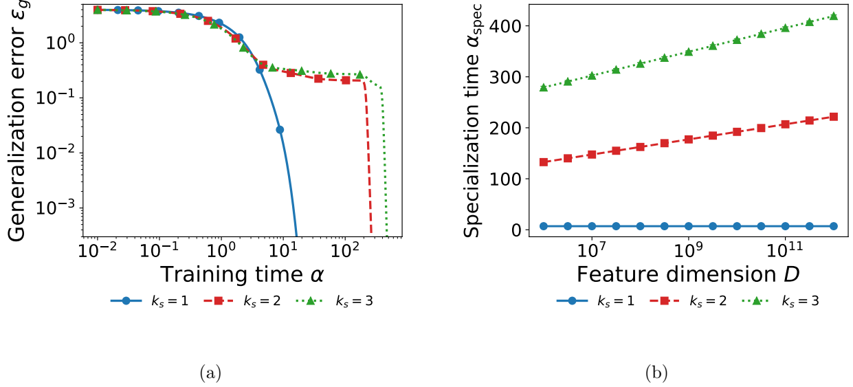
Figure 3: CNN students that match the teacher kernel size ( k_s = k_t ) learn with \mathcal{O}_D(D) samples, while students with k_s > k_t take \mathcal{O}_D(D \log D) samples. (a) Generalization error vs. training time \alpha for three kernel sizes, obtained by integrating the ODEs (17) from the order parameters of a random initialization at dimension D . (b) Specialization time \alpha_{\text{spec}} (Eq. (25), with \gamma_{\text{th}} = 0.99 ) against the feature dimension D . Markers are averages over random initializations, each obtained by integrating the ODEs (17) from the order parameters of a random initialization at dimension D . Standard errors are smaller than the marker size. Lines are fits a + b \ln D . Parameters: D = 10^{12} in panel (a), g = \text{erf} , k_t = 1 , P = 6 , S = I , \eta = 0.5 , T = 1 , \sigma = 0 , 128 random initial conditions in panel (b).
