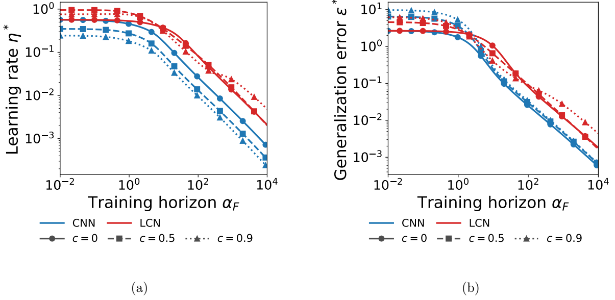
Figure 8: (a) Optimal learning rate \eta^* and (b) corresponding generalization error \varepsilon^* (Section 4.3) against the training horizon \alpha_F , for the CNN and the LCN at three values of the correlation c , from the same ODE solutions as Figure 6. Parameters: g = \text{erf} , P = 4 , k_s = k_t = 1 , T = 1 , \sigma = 1 , random initial condition in the limit D \rightarrow \infty .
