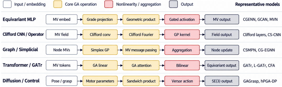
Figure 4 | Canonical design motifs in GA-native architectures. Different model families reuse a shared set of GA primitives but combine them in distinct computational patterns.
