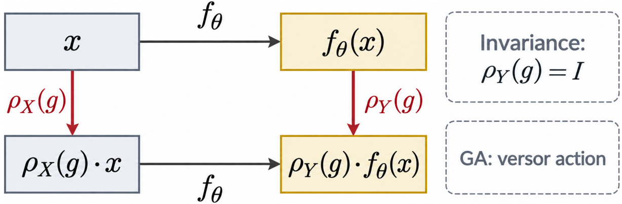
Figure 3 | Commutative view of equivariance. A NN layer is equivariant when transforming the input and then applying f_\theta yields the same result as applying f_\theta first and then transforming the output. Invariance is the special case with trivial output action.
