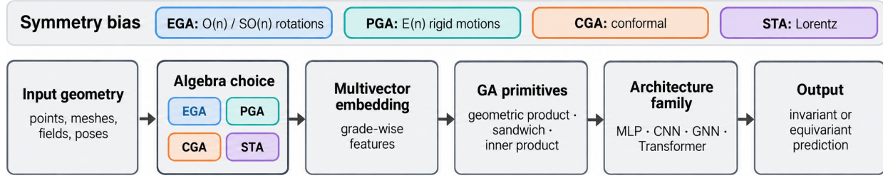
Figure 2 | Generic GA-native neural-network pipeline. The choice of algebra fixes the geometric vocabulary and symmetry bias; multivector embeddings are then processed by GA primitives and assembled into architecture families matched to downstream tasks.
