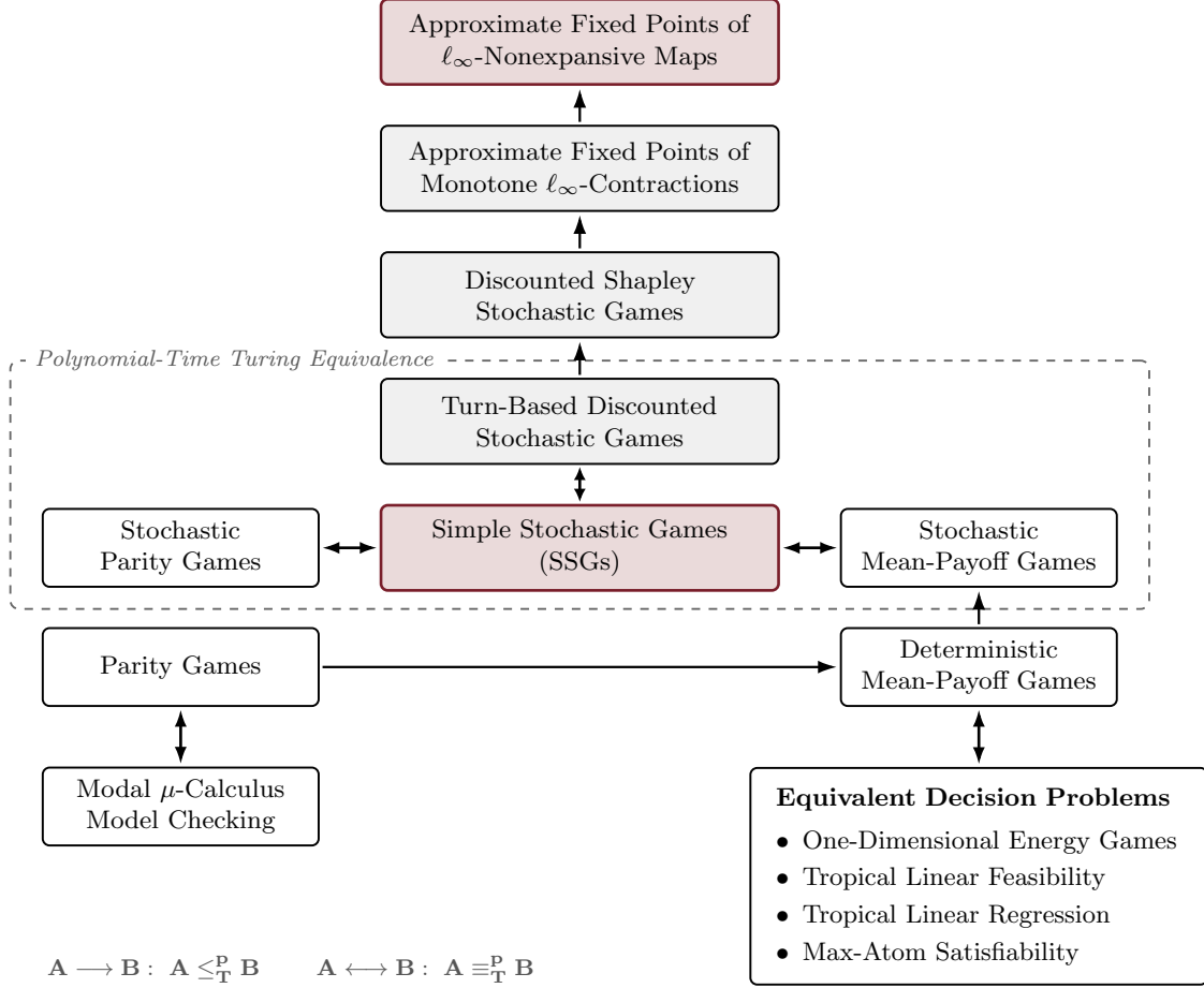
Figure 1: Polynomial-time reduction hierarchy connecting approximate \ell_\infty fixed-point computation to stochastic games and related decision problems. The dashed box groups turn-based, perfect-information stochastic games that are polynomial-time Turing equivalent [AM09a]. The upper reductions arise from the fixed-point formulation of discounted stochastic games, where sufficiently accurate approximations also yield exact solutions to SSGs [Sha53, BFG + 25]. The lower reductions connect parity games, modal \mu -calculus model checking, and decision problems equivalent to deterministic mean-payoff games [Jur98, EJS01, BCD + 11, AGG12, AGQS23, AM09b]. The red boxes highlight our main result and its application to SSGs, the gray boxes indicate intermediate problems, and the white boxes show further consequences.
