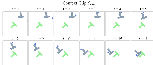
Figure A9: Qualitative Example of an Exploratory In-Context Interaction Clip C_{eval} in the Push-T Environment. This in-context interaction clip is used by PhysCalWorld to generate the open-loop rollout results in Figure A8. The clip is collected using a CoM-agnostic PPO policy and encoded by the context encoder g_\phi into a physics descriptor token to calibrate the world model's predictions.
