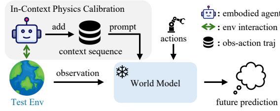
Figure 1: In-Context Physics Calibration for World Models. In a test environment with unknown transition dynamics, an embodied agent first executes exploratory actions to collect an in-context interaction sequence. This sequence is then provided as prompt to calibrate the world model such that future predictions adhere to the actual dynamics of the test environment.
