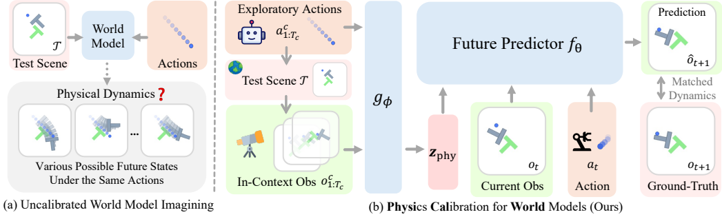
Figure 2: Method Overview. PhysiCalWorld calibrates action-conditioned world models to the actual dynamics of a test scene via prompting with in-context interaction. In (a), the current visual observation alone cannot identify the physical dynamics of the test scene \mathcal{T} , forcing the world model to guess among multiple potential future states. In (b), starting from the top left, exploratory actions a_{1:T_c}^c are first executed in the test scene \mathcal{T} , yielding observations o_{1:T_c}^c . The context encoder g_\phi then extracts physics information from this obs-action sequence and compresses it into a physics descriptor token \mathbf{z}_{\text{phy}} . Conditioned on \mathbf{z}_{\text{phy}} , the world model is able to generate future predictions \hat{o}_{t+1} consistent with the test scene’s dynamics.
