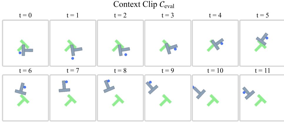
Figure A2: Qualitative Example of an In-Context Interaction Clip C_{eval} used in the Push-T Environment. We provide the in-context interaction clip used by +PhysiCal (Ours) to generate the main-text rollout results in Figure 4 (a). This clip is collected via the same policy (i.e., a CoM-agnostic PPO policy) that is used to generate the training dataset. This clip is encoded by the context encoder g_\phi into a physics descriptor token , which is used to calibrate the world model’s predictions.
