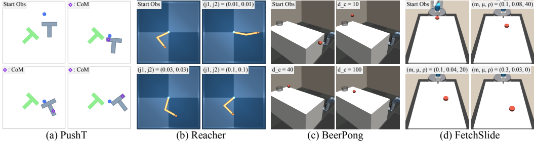
Figure 3: Environment Demonstrations. We evaluate our method on four simulation environments featuring diverse variations of physics properties. For each environment, we show four images: the top-left image is a random initial observation, while the remaining three images demonstrate how executing the same action sequence yields different future states due to different physics parameters of the scenes. Specifically, in (a) Push-T, the center of mass of the T-block is varied; in (b) Reacher, the joint damping of the two-link arm is varied; in (c) BeerPong, the energy dissipation upon table contact is varied; in (d) FetchSlide, three physics properties vary concurrently: puck mass, surface friction, and aerodynamic drag.
