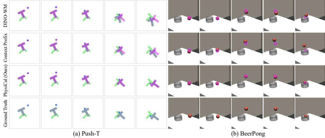
Figure 4: Qualitative Open-Loop Rollout Results in Push-T and BeerPong. We show a subset of the full rollouts due to limited space and crop the synthesized images in BeerPong for clearer view. We use ■ masks to indicate the ground-truth location of the target objects. Note that the physics configuration of these test scenes is unknown to the models and PhysiCal calibrates the predictions solely based on a given in-context interaction clip (Figure A2 and Figure A3), yielding results that closely match the ground truth.
