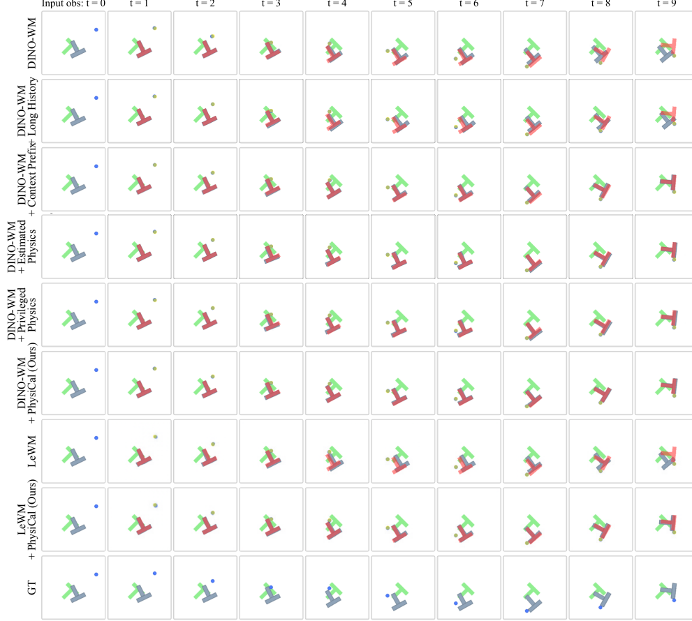
Figure A8: Qualitative Open-Loop Rollouts in the Push-T Environment. We present open-loop rollouts, where models are only given the initial observation and autoregressively predict future observations. All context-conditioned models use the interaction clip shown in Figure A9. DINO-WM + Ours, LeWM + Ours, DINO-WM + Privileged Physics, and DINO-WM + Context Prefix closely match the ground-truth motion, while the remaining baselines exhibit substantial prediction errors. Though Context Prefix predicts accurately, it directly attends to the full context sequence, making its inference substantially slower.
