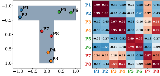
Figure 7: Cosine Similarity of Physics Descriptor Tokens of Different CoMs in Push-T. We compute descriptor token z_{\text{phy}} of 8 unseen centers of mass and visualize their pairwise cosine similarity. Trained without any physics labels, our method can still learn a structured, physics-correlated latent space, e.g., adjacent centers of mass yield high similarity while remote pairs yield negative values.
