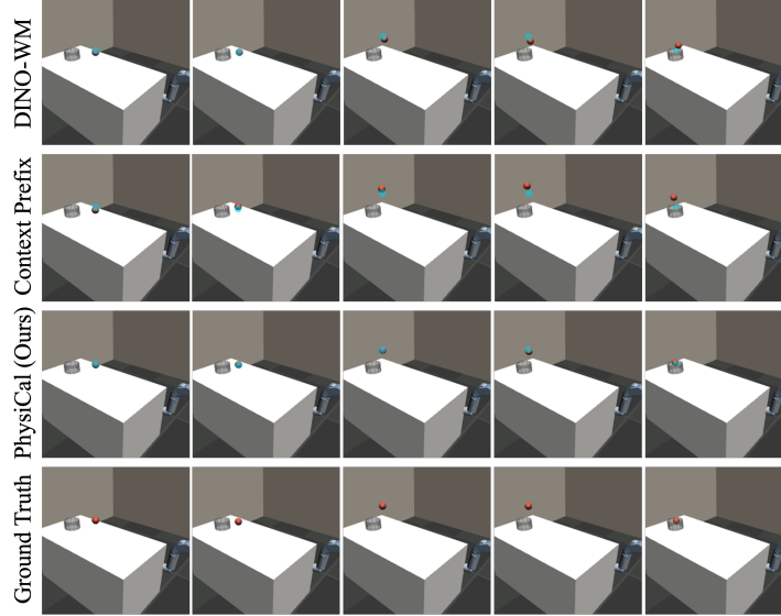
Figure A5: Uncropped Open-Loop Rollouts in the BeerPong Environment. We present the full-scene view of the BeerPong rollouts shown in Figure 4(b), displaying the predicted ball trajectories relative to the table and cup. DINO-WM + Ours accurately predicts the ball’s bounce, while DINO-WM and DINO-WM + Context Prefix overestimate its rebound height. The semi-transparent cyan overlay marks the ground-truth ball position.
