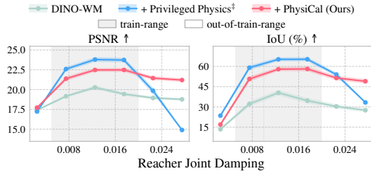
Figure 8: Extrapolation to Out-of-Distribution Physics Parameters in Reacher. We report results of open-loop rollouts. For each circle, we sample 15 damping values within a bin centered at its x -coordinate evaluated on 5 episodes per value, 75 total.
