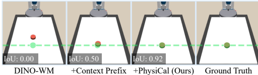
Figure 5: Qualitative Comparison in FetchSlide. Visual comparison of open-loop rollout predictions under identical striking actions in an unseen test scene. We only demonstrate the final frame due to space limit. The green mask denotes the ground-truth puck position.
