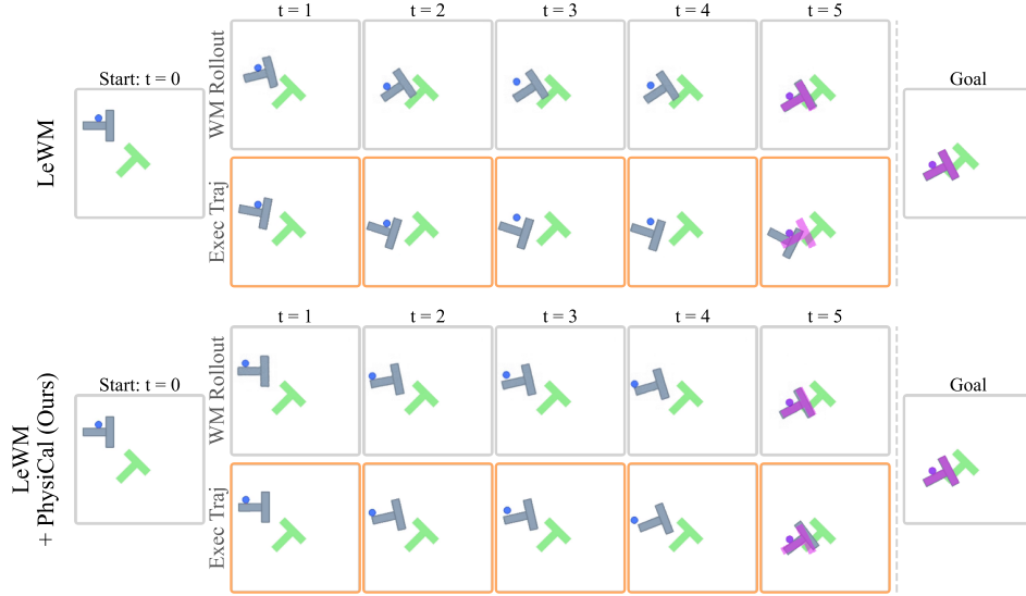
Figure A18: Qualitative Planning Rollouts in the Push-T Environment, LeWM-Based Models. Action sequences generated by CEM to reach a goal observation are executed in the environment and compared with the world models’ predictions. LeWM + Ours uses the interaction clip presented in Figure A19 and accurately predicts the resulting motion. In contrast, LeWM underestimates the effect of the push at t = 3 , with the T-block moving and rotating substantially farther than predicted at t = 4 .
