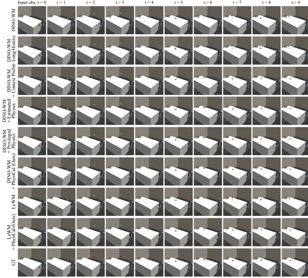
Figure A12: Qualitative Open-Loop Rollouts in the BeerPong Environment. We provide open-loop predictions of the ball’s trajectory, generated autoregressively without subsequent ground-truth observations. All models that use context receive the interaction clip in Figure A13. DINO-WM + Ours, LeWM* + Ours, DINO-WM + Privileged Physics, and DINO-WM + Context Prefix accurately reproduce the ball’s bounce, while the remaining baselines overestimate its rebound. The accuracy of Context Prefix, however, comes at the cost of substantially slower inference due to direct attention over the full context sequence. LeWM* denotes TC-LeWM in BeerPong, as we find that this variant can significantly boost the performance of LeWM in BeerPong.
