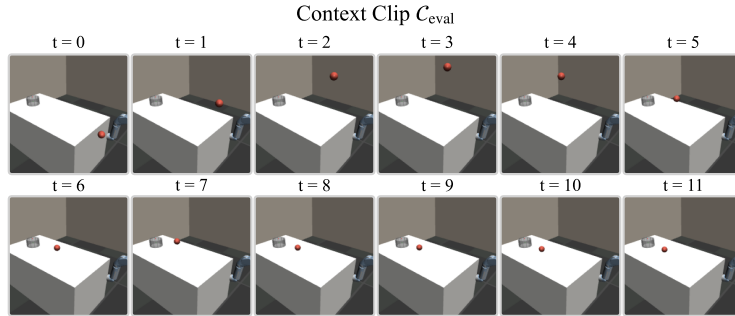
Figure A13: Qualitative Example of an Exploratory In-Context Interaction Clip C_{eval} in the BeerPong Environment. We present the in-context interaction clip used by PhysiCalWorld to generate the open-loop rollout results in Figure A12. The context encoder g_\phi encodes this clip, collected using a randomly sampled throw action, into a physics descriptor token that calibrates the world model’s predictions.
