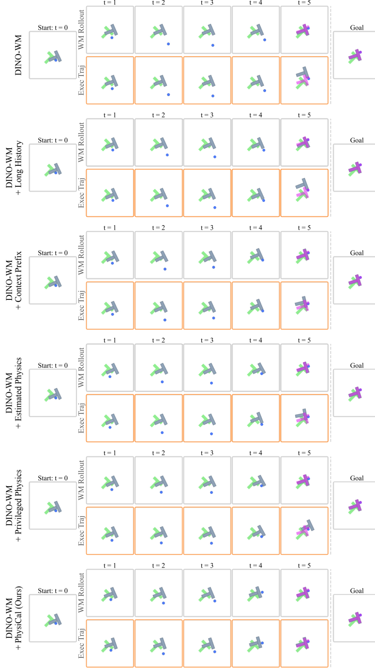
Figure A16: Qualitative Planning Rollouts in the Push-T Environment, DINO-WM-Based Models. We use CEM to optimize action sequences toward a goal observation and execute them in the environment, comparing model predictions with the resulting motion. All context-conditioned models use the interaction clip shown in Figure A17. DINO-WM + Ours closely matches the executed motion, while the remaining models misrepresent the T-block's translational and rotational dynamics.
