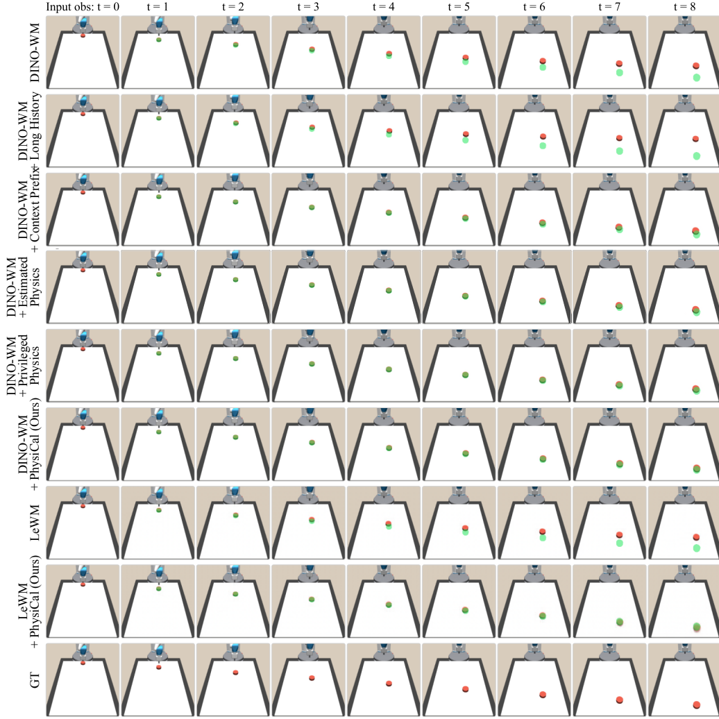
Figure A14: Qualitative Open-Loop Rollouts in the FetchSlide Environment. We present an eight-frame open-loop rollout, in which each model predicts future observations autoregressively without receiving additional ground-truth observations. The interaction clip shown in Figure A15 is shared by all context-conditioned models. DINO-WM + Ours, LeWM + Ours, and DINO-WM + Privileged Physics closely match the ground-truth puck motion. DINO-WM + Context Prefix slightly underestimates its movement, while the remaining baselines without context exhibit more pronounced underestimation.
