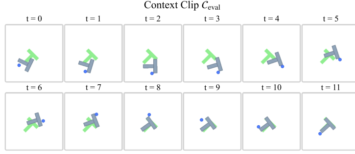
Figure A17: Qualitative Example of an In-Context Interaction Clip C_{eval} in the Push-T Environment. We provide the in-context interaction clip used by PhysiCalWorld to generate the planning results in Figure A16. Collected using a CoM-agnostic PPO policy, this clip is encoded by the context encoder g_\phi into a physics descriptor token , which is used to calibrate the world model’s predictions during planning.
