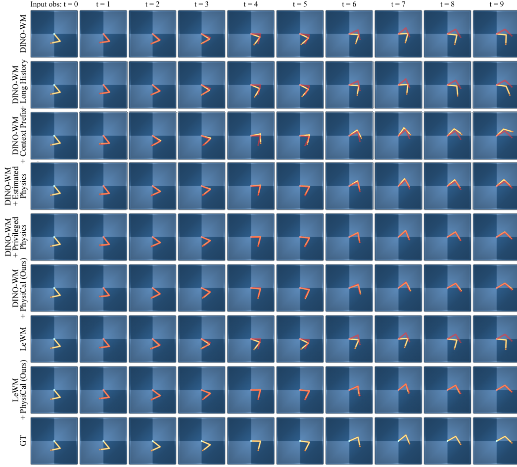
Figure A10: Qualitative Open-Loop Rollouts in the Reacher Environment. We show autoregressive predictions of the arm’s motion without providing further ground-truth observations during the rollout. All the models that ingest a context clip use the same one as presented in Figure A11. DINO-WM + Ours, LeWM + Ours, and DINO-WM + Privileged Physics accurately predict the arm’s motion. Context Prefix overestimates the motion, whereas the remaining baselines underestimate it, suggesting that it uses the context to adjust its predictions but remains less accurate than our models.
