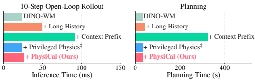
Figure 6: Inference Speed Comparison of Open-Loop Rollout and Planning in Push-T. For planning, we use the same Cross-Entropy Method (CEM) setup as DINO-WM. See Appendix C.3 and C.4 for additional results.
