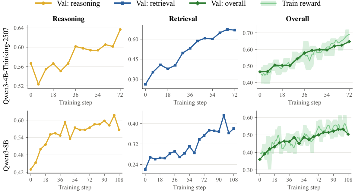
Figure 3: Training dynamics of LONGZERO up to the reported checkpoints. Validation scores are measured every 6 steps on held-out reasoning and retrieval data (overall: weighted by set size). The training reward mixes both data types (line: 5-step average; band: range over the same window).
