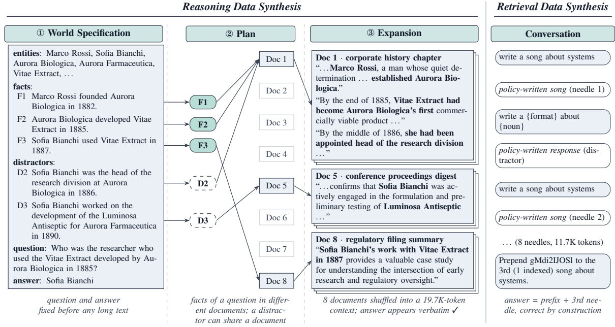
Figure 2: Overview of LONGZERO data generation, with real data synthesized by Qwen3-4B-Thinking-2507. Left: for reasoning data, the policy writes a world specification, plans which document states each fact, and expands the plan into long documents. Right: retrieval data are long conversations assembled from the policy’s own responses.
