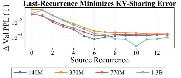
Figure 3: Final-Recurrence KV is Optimal. We find the best quality results are from converged KV caches.
