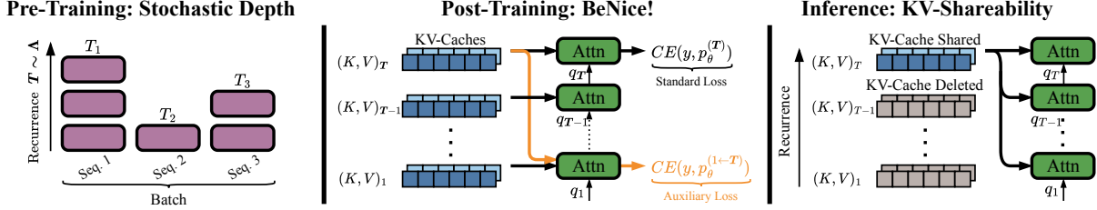
Figure 1: Stochastic Depth, BeNICE!, and KV-Shareability. ( Left ) During pretraining, stochastic depth induces contractive residual dynamics. ( Middle ) BeNICE! post-trains by injecting the final recurrence KV-caches into the first recurrence. Together, they enable KV-shareability in looped models, retaining only the final recurrence’s KV-cache without degrading quality ( Right ).
