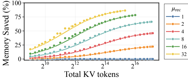
Figure 8: Global Memory Reduction of KV-Sharing. We measure and fit the memory overhead of KV-sharing, varying test-time recurrences. KV-sharing using Mooncake traces [51].
