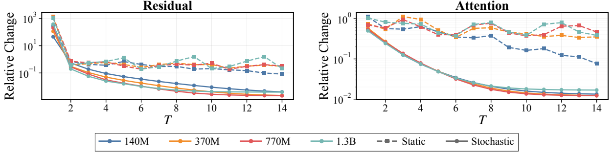
Figure 2: Residuals and Attention Convergence. Relative step-to-step change of the residual stream ( \|h_i - h_{i-1}\|/\|h_{i-1}\| , left ) and attention pattern ( \|A_i - A_{i-1}\|/\|A_{i-1}\| , right ) across recurrence depth T . Stochastic-depth training exhibits fixed-point convergence, while static-depth does not.
