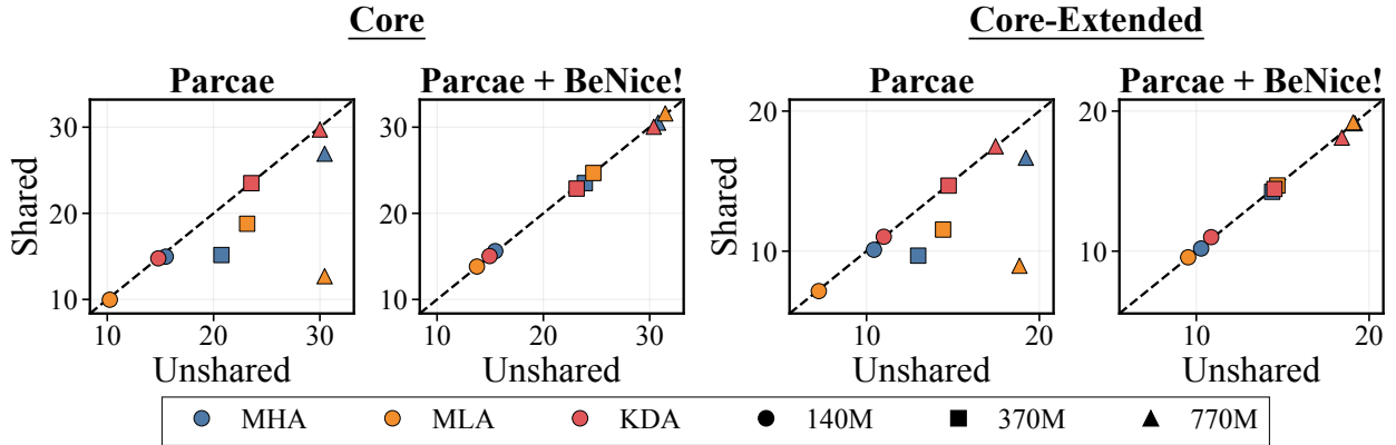
Figure 6: KV-Shareability with Memory-Efficient Sequence Mixers. We train Parcae [50] models with MHA [68], MLA [13], and KDA [65]. We find that BE NICE! allows memory-efficient sequence mixers to have KV-shareability, reducing inference overhead.
