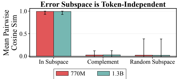
Figure 5: KV-Sharing Error Subspace Similarity. We find that tokens are strongly aligned within the subspace, but orthogonal in its complement and a random 8-dimensional subspace.
