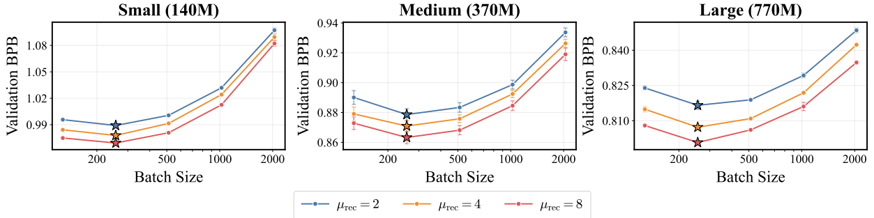
Figure 15: Transferability of Batch Size. Optimal batch size transfers strongly across deeper recurrences for all model backbones.
