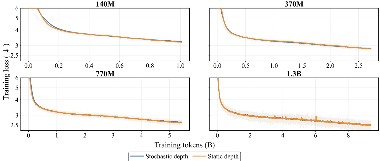
Figure 13: Training Curves for Stochastic- and Static-Depth Models. Training loss as a function of training tokens across model scales. The curves closely overlap, showing that stochastic- and static-depth training exhibit similar optimization dynamics.
