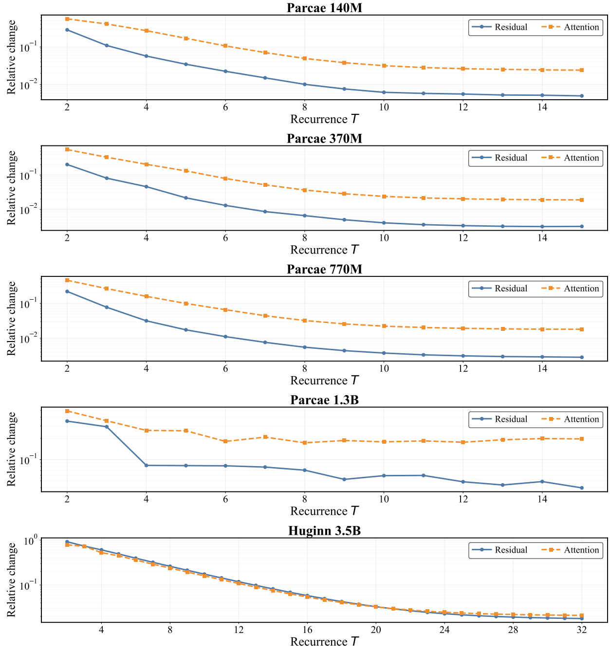
Figure 12: Fixed-point convergence of pretrained looped models. Relative changes in the recurrent residual state and attention pattern decrease with recurrence depth for the released Parcae models and Huginn.
