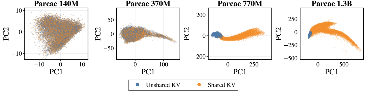
Figure 4: KV-Sharing Failures Converge to Incorrect Fixed Points. We visualize fixed points of several tokens after T = 8 test-time recurrence with unshared and shared KV-caches. Models with KV-shareability (e.g., 140m and 370m) converge to the same fixed point under both setups, while models without KV-shareability (e.g., 770M and 1.3B) do not. See Section H for extended details.
