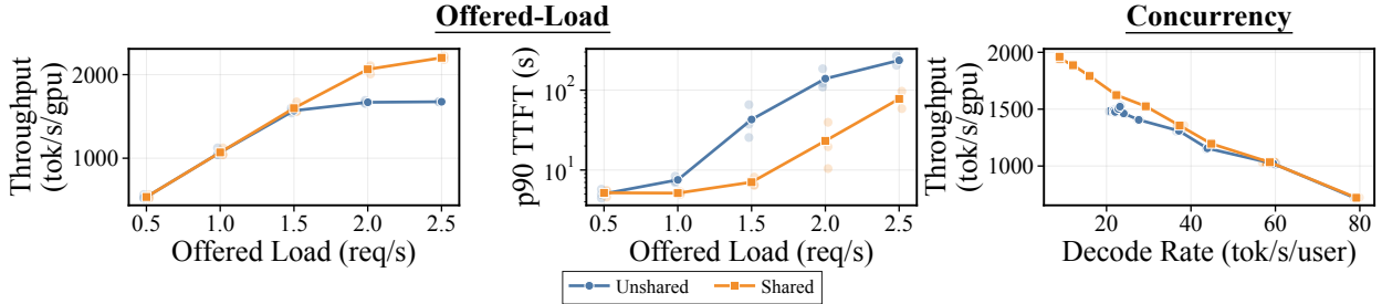
Figure 10: Throughput Frontier of KV-Sharing. (Left) Under increasing offered load, KV-Sharing improves throughput and reduces TTFT over unshared looping. (Right) Under high concurrency load, KV-sharing improves overall throughput at matched decode rates.
