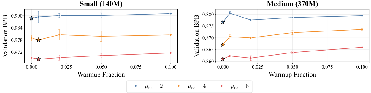
Figure 17: Transferability of Warmup Ratio. We observe optimal warmup ratios to transfer well across recurrences, with some minor variation in relatively flat regions.
