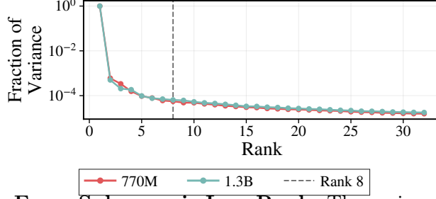
Figure 11: KV-sharing Error Subspace is Low Rank. The variance within KV-sharing error subspace is well explained with a few directions.
