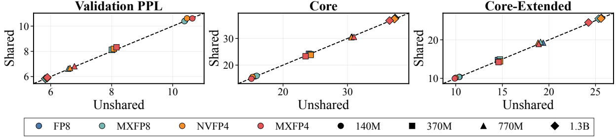
Figure 7: Quality of KV-Sharing and -Quantization. We report changes in climbmix PPL [16], Core, and Core-Extended [38] after quantizing the KV-shared cache across MHA [68] model scales. KV-sharing maintains quality across cache precisions.
