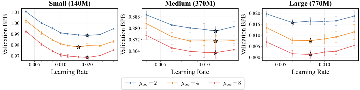
Figure 14: Transferability of Learning Rate. Optimal learning rate transfers strongly across deeper recurrences for all model backbones.
