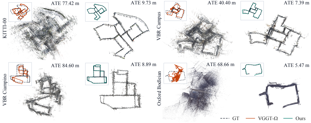
Figure 4: Trajectory comparison on four long sequences with identical VGGT-Omega points.
