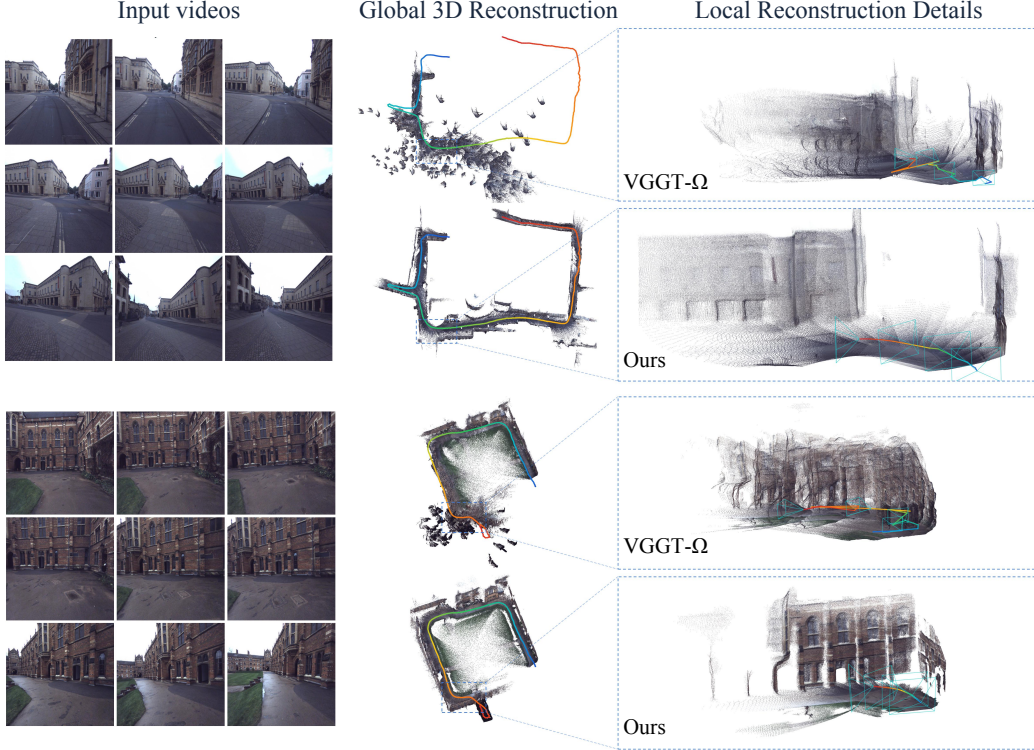
Figure 3: Qualitative comparison between VGGT-Omega chunk placement and HiP3R.
