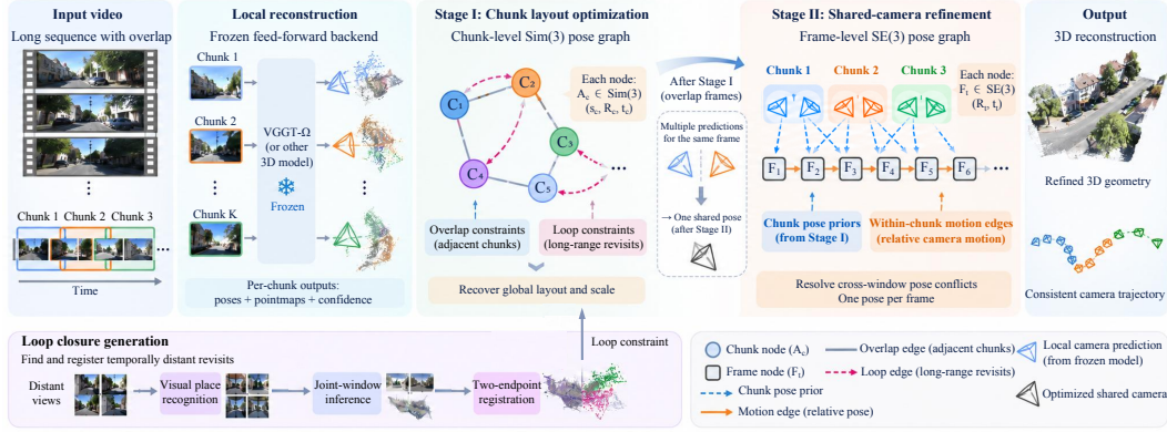
Figure 2: Overview of HiP3R. Frozen backends predict overlapping chunks. Stage I builds a chunk-level \text{Sim}(3) graph from overlap and loop constraints to recover layout and scale. Stage II estimates one shared \text{SE}(3) camera per frame under that layout.
