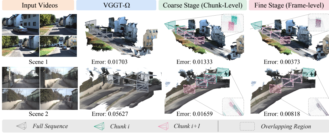
Figure 1: Overlapping predictions recover local geometry in inconsistent frames. Coarse layout optimization corrects global placement and scale, but keeps each chunk’s internal cameras. Shared-camera trajectory refinement estimates one trajectory from predictions and within-chunk motion.
