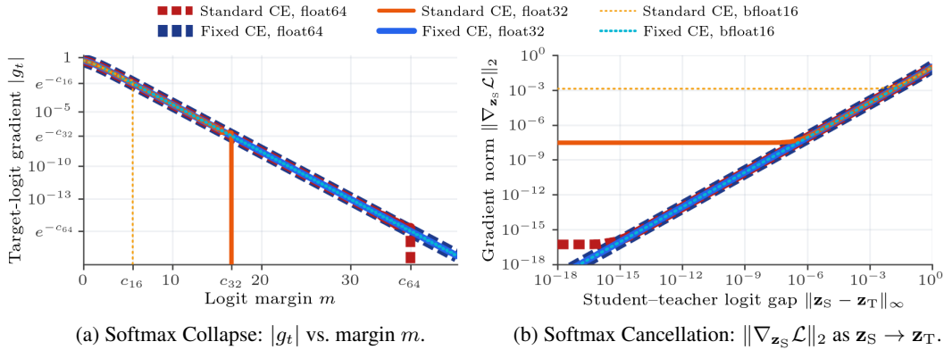
Figure 1: The two bugs in standard softmax and cross-entropy. (a) Softmax Collapse: As a model becomes more confident in the correct class (thereby increasing the logit margin m ), the true gradient on the target logit shrinks exponentially, but standard implementations incorrectly round that gradient to zero once m crosses a precision cliff ( \approx 5.5 in bf16, 16.6 in fp32, and 36.7 in fp64). (b) Softmax Cancellation: In soft-target distillation, as student logits \mathbf{z}_S approach teacher logits \mathbf{z}_T , the true gradient shrinks toward zero, but standard implementations lose precision and plateau at a non-zero noise floor. Our fix eliminates both bugs and yields accurate gradients across all precisions.
