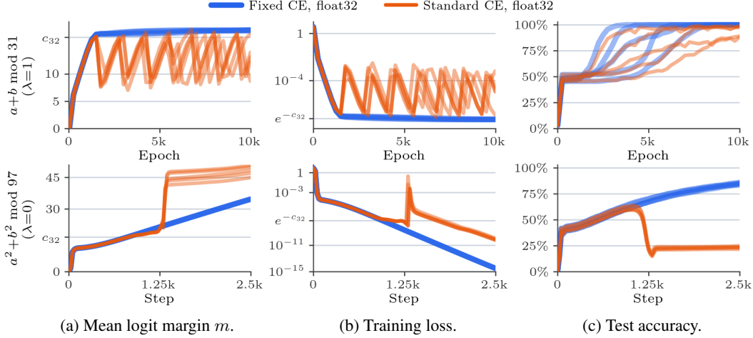
Figure 2: The Slingshot mechanism (Thilak et al., 2022) with and without weight decay (5 random seeds, fp32). Top row ( a + b \bmod 31 , \lambda = 1 , \epsilon = 10^{-8} , Varma et al. 2023): Standard cross-entropy hits the fp32 cliff ( m = c_{32} \approx 16.6 , where loss rounds to 0) and repeatedly drops and rebounds, slowing and degrading grokking; fixed cross-entropy crosses c_{32} smoothly, groks faster on all 5 seeds, and saturates just above c_{32} at m \approx 18.4 (Section 5). Bottom row ( a^2 + b^2 \bmod 97 , \lambda = 0 , \epsilon = 10^{-16} , Doshi et al. 2024): Without weight decay, hitting c_{32} around step 1250 triggers a spike that drops standard cross-entropy test accuracy from 61% to 23%, whereas fixed cross-entropy continues smoothly to 85%.
