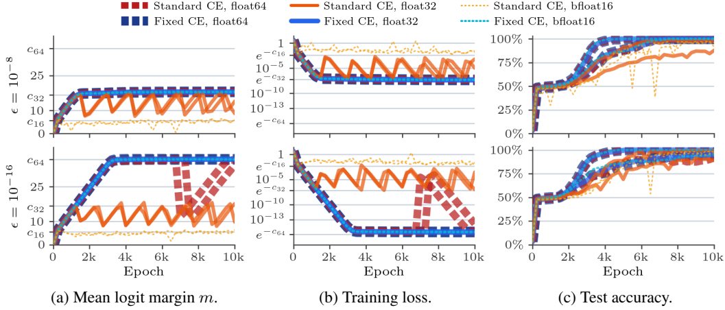
Figure 5: Standard cross-entropy fails at the precision cliff c_d of its floating-point format; fixed cross-entropy removes the cliff across all precisions ( a + b \bmod 31 , \lambda = 1 ; 2 of 5 seeds shown). Top: \epsilon = 10^{-8} . Bottom: \epsilon = 10^{-16} , where even fp64 standard cross-entropy fails at c_{64} while fixed cross-entropy converges smoothly.
