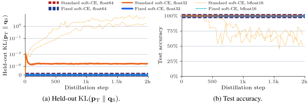
Figure 7: Soft-target distillation when the student is initialized with the teacher’s weights ( \theta_S^{(0)} = \theta_T , T = 4 , \epsilon = 10^{-8} , 2 of 3 seeds shown). Fixed soft-target cross-entropy stays at KL = 0 and 100% accuracy across all precisions; standard soft-target cross-entropy amplifies rounding error into parameter drift in bf16 and a brief KL spike in fp32.
