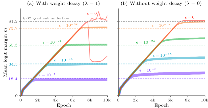
Figure 4: Logit margins when training with our fixed cross-entropy and LaProp on a + b \bmod 31 in fp32 ( \beta_1 = 0.9 , \beta_2 = 0.98 ; 3 seeds per setting as solid lines, analytical predictions as dashed lines). (a) With weight decay ( \lambda = 1 ), the margin for each \epsilon > 0 grows along the \epsilon = 0 trajectory and levels off at the predicted equilibrium m^*(\epsilon) = \log(1/\epsilon) (colored y -ticks), whereas \epsilon = 0 keeps growing until the fp32 gradients themselves underflow at m \approx 81.2 (gray). (b) Without weight decay ( \lambda = 0 ), nothing balances the g_i/\epsilon step, so the margins rise past \log(1/\epsilon) and continue drifting upward.
