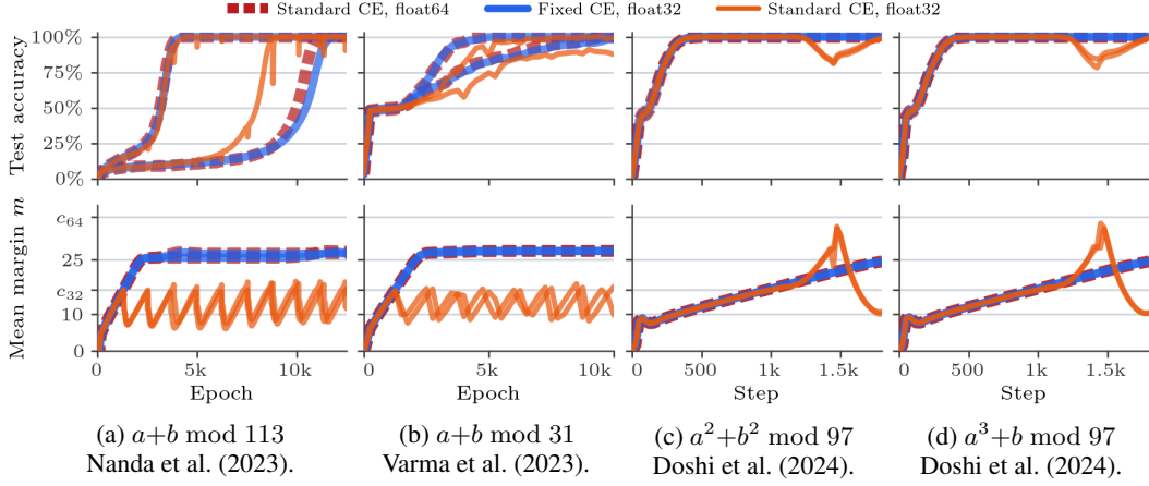
Figure 6: Results across four grokking tasks at \epsilon = 10^{-12} (2 of 3–5 seeds shown): 1-layer Transformers (a, b) and 2-layer MLPs (c, d). Fixed cross-entropy in fp32 (blue) matches fp64 standard cross-entropy (red), while standard cross-entropy in fp32 (orange) breaks at c_{32} .
