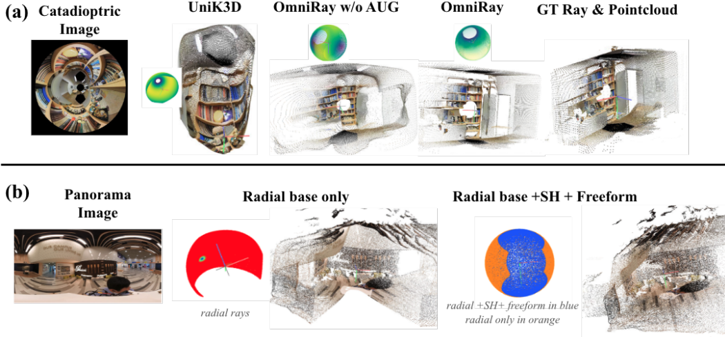
Figure 5: Ablation. (a) Held-out catadioptric camera: predicted ray field and point cloud for UniK3D, OmniRay trained without random-lens augmentation, and the full model, against the ground truth. (b) Panoramic image: the radial base alone covers only part of the sphere (orange) and leaves the reconstruction torn, while the spherical-harmonic and free-form residuals complete the field (blue) and close the geometry.
