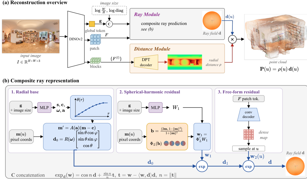
Figure 2: OmniRay Overview. Given a single image, a DINOv2 ViT-L/14 encoder produces global and dense features that drive two branches. The Ray Module progressively builds a camera-agnostic ray field from a monotone radial base, a spherical-harmonic residual, and a free-form residual. The Distance Module predicts a positive radial distance for each pixel. Combining the final ray \mathbf{d} and distance \rho yields the local pointmap \mathbf{P} = \rho \mathbf{d} , recovering 3D geometry up to scale without camera intrinsics or a camera-type label.
