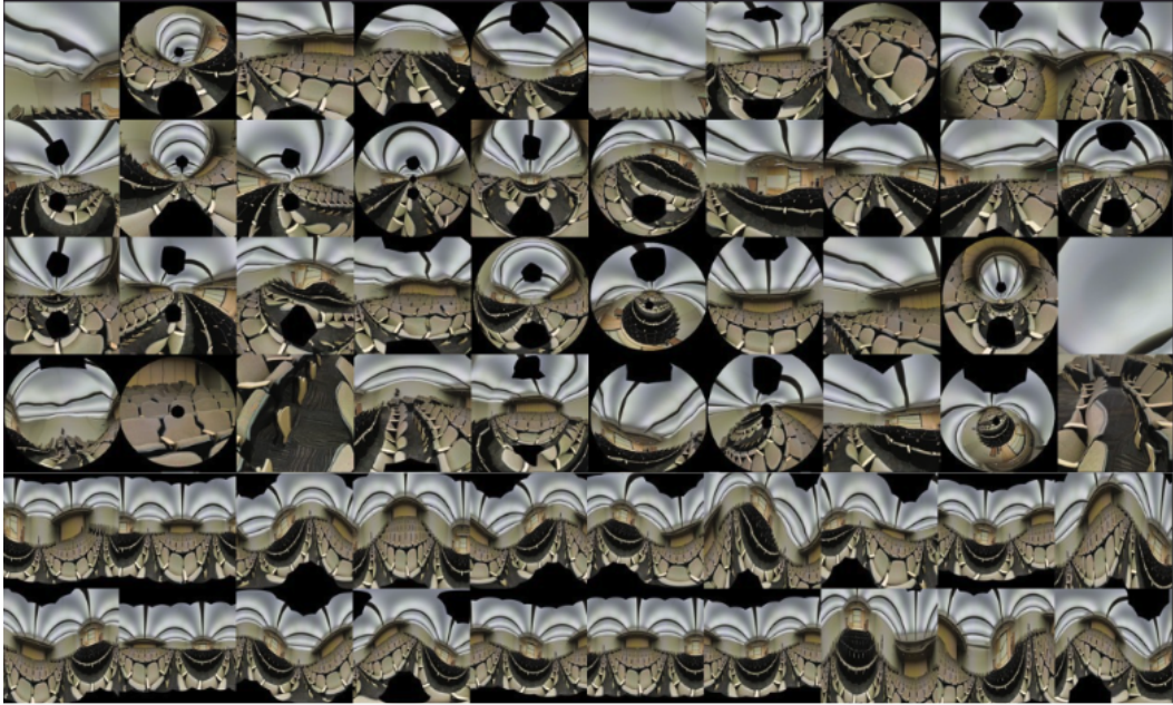
Figure 8: Random-lens augmentation. Images rendered from a single panorama under cameras drawn from the sampling distribution of Sec. 4.2. A camera is a viewing direction, a monotone radial profile and an imaged sensor region, so one family spans narrow perspective crops, wide-angle and fisheye views, off-center and anisotropic sensors, and annular domains. The projection varies continuously from sample to sample, so no fixed map from image position to ray direction fits more than one of them. Draws falling close to either held-out geometry are rejected and never enter training.
