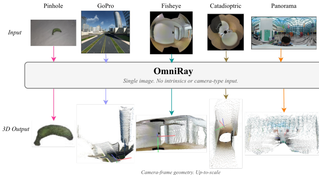
Figure 1: OmniRay reconstructs 3D geometry from a single image across diverse camera geometries. A single model predicts an up-to-scale, camera-frame point cloud without camera intrinsics or camera-type input. Columns show inputs and reconstructions for pinhole, GoPro, fisheye, catadioptric, and panoramic cameras, respectively. Note that the GoPro and catadioptric camera configurations are withheld from training.
