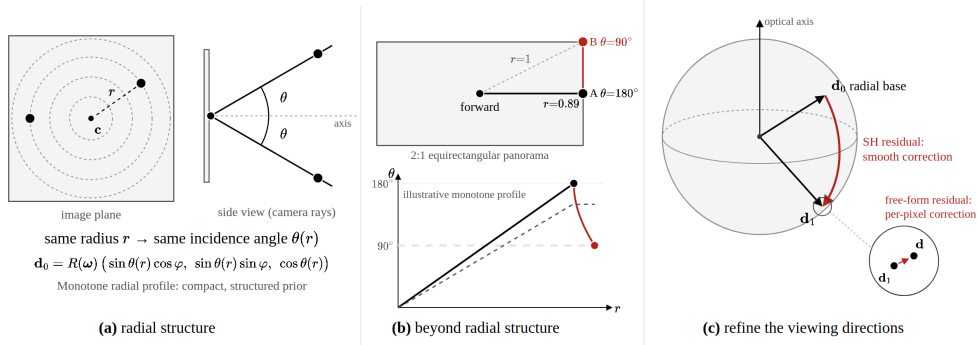
Figure 3: Why combine the radial construction with the residual corrections? (a) The radial representation gives the same incidence angle to pixels that lie at the same radius in the base coordinates. (b) In the centered 2:1 equirectangular projection, point A is closer to the center of the image than point B, yet has a higher incidence angle. A monotone radial function cannot accommodate such ordering under fixed coordinate transformation and orientation. (c) The spherical-harmonic and free-form residuals improve upon the base direction via iterative correction on the unit sphere.
