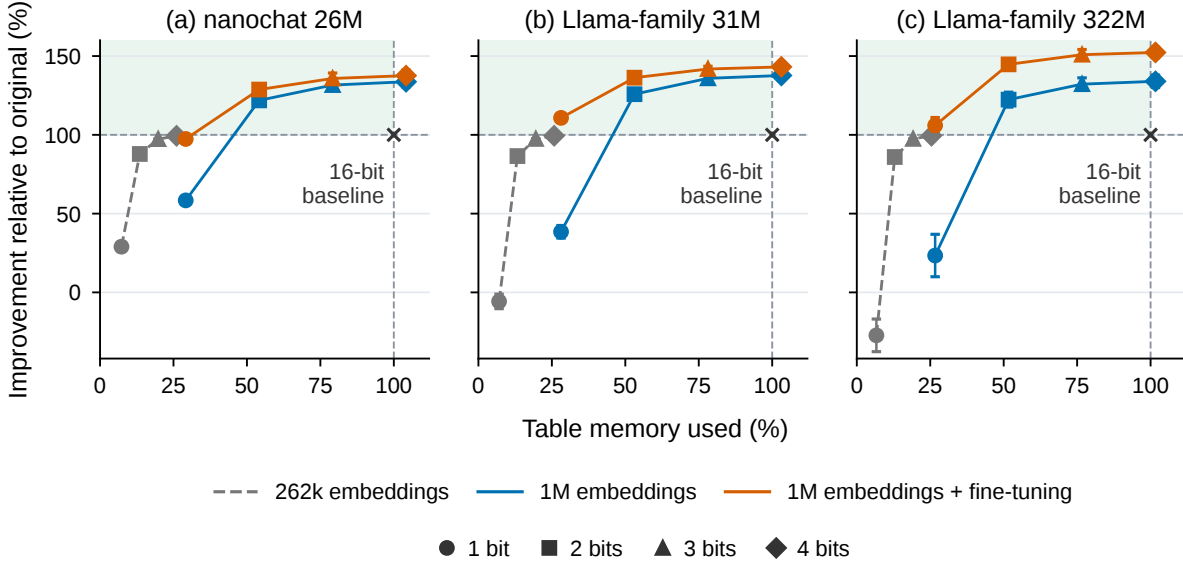
Figure 7: Larger low-bit tables can improve performance while using less memory. Both axes use the original 262k-embedding, 16-bit tables as the reference, marked at (100%, 100%). The shaded region indicates greater improvement while using less memory. Fine-tuning follows compression. Error bars show sample standard deviations over three seeds.
