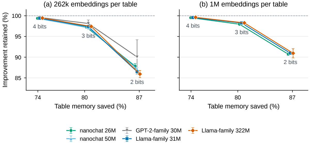
Figure 2: Four-bit embeddings save about 75% of table memory while retaining more than 99% of the improvement. (a) The five models with the default 262k embeddings per table. (b) The 26M nanochat model and both Llama-family models with 1M embeddings per table. Points and error bars show means and sample standard deviations over three seeds. The dashed line matches the original 16-bit tables.
