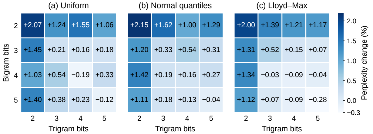
Figure 10: Qwen3.8-Flash-Next: all sixteen bigram/trigram allocations for each codebook, using error-fitted scales. Entries show validation perplexity change (%).
