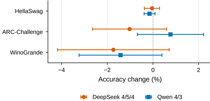
Figure 5: Downstream evaluation of the selected mixed-precision settings. Change in accuracy (%) for DeepSeek 4/5/4 and Qwen 4/3, computed as low-bit accuracy minus original accuracy. Error bars show paired 95% bootstrap confidence intervals. The settings save 46.7% and 55.0% of table memory, respectively.
