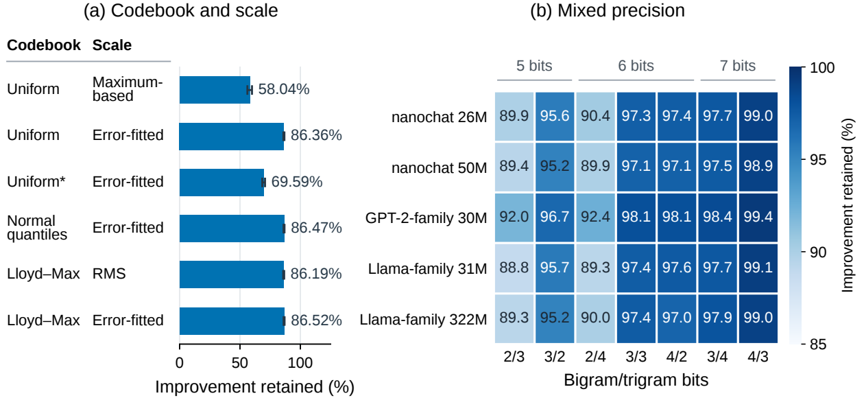
Figure 3: Choosing an appropriate embedding scale is more important than choosing among uniform, normal-quantile, and Lloyd-Max codebooks. (a) Two-bit comparisons on the 31M Llama-family model with 262k embeddings per table. Uniform* is the three-value variant \{-1, 0, 1\} that includes zero. Error bars show sample standard deviations over three seeds. (b) Selected bigram/trigram precision pairs for all five models with the default 262k embeddings per table. Appendix C.3 gives all precision pairs.
