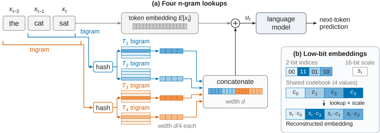
Figure 1: Four n-gram lookups, stored at low precision. (a) The bigram and trigram ending at the current token each retrieve two embeddings. The four embeddings are concatenated and added to the token embedding to form u_t . (b) Each two-bit index selects one of four codebook values. Multiplying each selected value by the embedding’s 16-bit scale reconstructs the embedding. Codebook values use 16 bits and are shared across all embeddings of a table.
