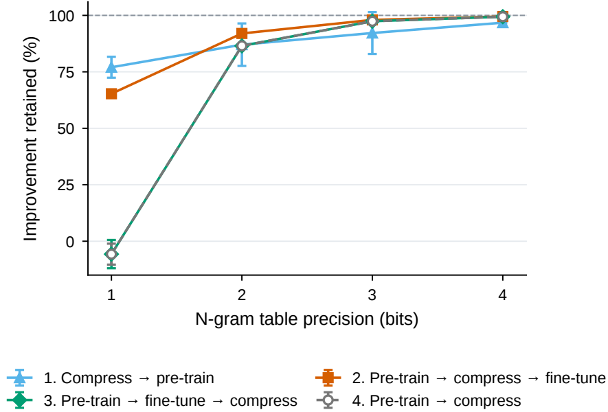
Figure 6: Fine-tuning after compression recovers much of the n-gram improvement. Improvement retained on the 31M Llama-family model, relative to full-precision and no-table models with the same training budget. Error bars show sample standard deviations over three seeds.
