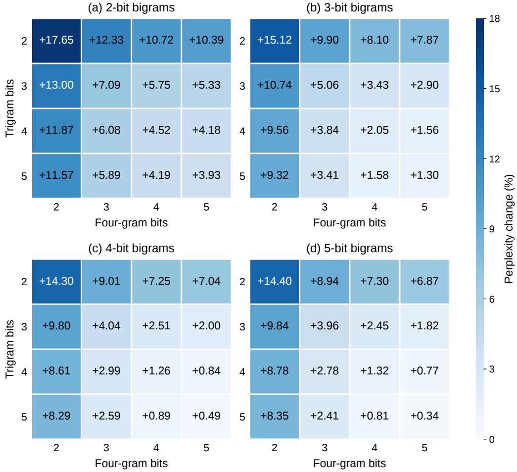
Figure 9: DeepSeek-V4.1-Flash: all 64 bigram/trigram/four-gram precision allocations with Lloyd–Max codebooks and error-fitted scales. Entries show validation perplexity change (%).
