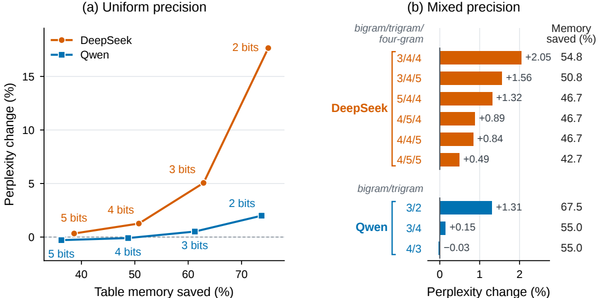
Figure 4: Uniform and mixed precision provide different memory–performance choices in DeepSeek-V4.1-Flash and Qwen3.8-Flash-Next. (a) Two through five bits for every table, with labels giving bits per value. (b) Representative mixed allocations, ordered by n-gram length. Both panels use WikiText-2 validation perplexity.
