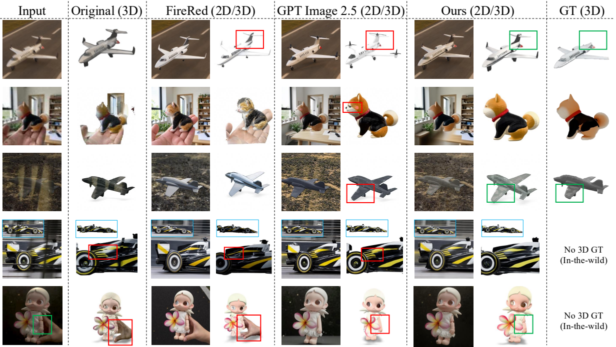
Figure 3. Comparison of images (2D) and Pixal3D outputs (3D). Original (3D) uses unedited inputs. Ours (2D) uses purified images. Boxes mark structure and appearance changes.
