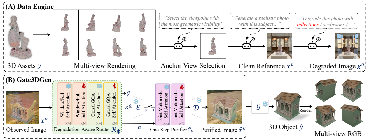
Figure 2. Overview of Gate3DGen. (A) Data Engine. We render 3D assets from multi-view, select informative anchor views, and apply composite degradations to construct aligned observation-reference pairs (x^o, x^c) . (B) Gate3DGen. Router \mathcal{R}_\phi bypasses inputs classified as clean ( \hat{\gamma} = 0 ). Otherwise ( \hat{\gamma} = 1 ), its features h guide the one-step DiT purifier \mathcal{C}_\theta . x^c conditions the frozen 3D generator \mathcal{G} . Clean references and spatial losses are used only in training.
