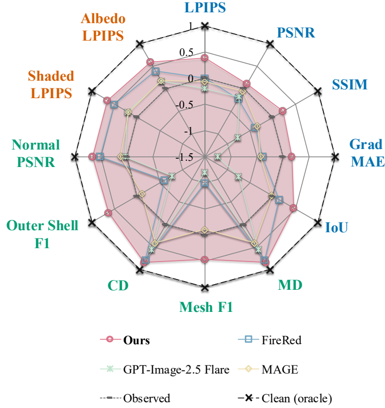
Figure 4. Oracle-normalized comparison of 2D purification and downstream 3D generation. The radar plot summarizes percentage progress from the observed degraded input (0) toward the matched clean-reference oracle (1) using the metrics reported in Tables 2 and 3. Negative values indicate deterioration relative to the observed input. Blue labels denote 2D image metrics, green labels denote 3D geometry and normal metrics, and orange labels denote rendered-appearance metrics. Lower-is-better metrics are direction-adjusted so that farther outward is always better.
