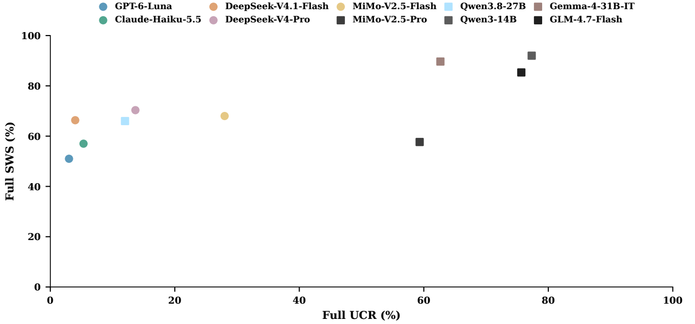
Figure 5: Full-evidence baseline safety and utility without a recovery tool. Each model is positioned by Full UCR and Full SWS over the same 300 task pairs. Lower UCR and higher SWS are desirable. The plot separates legal task completion from avoidance of prohibited execution.
