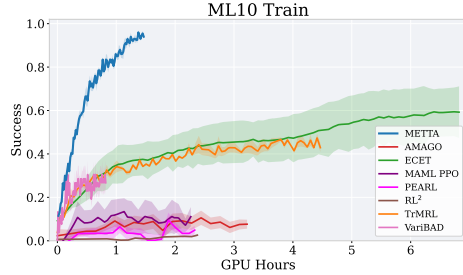
Figure 7: Success versus GPU hours.
