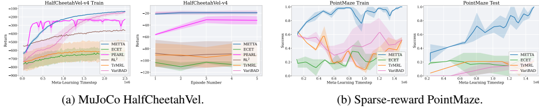
Figure 3: Fast adaptation during meta-training and meta-testing. (a) HalfCheetahVel training return and adaptation across meta-test episodes. (b) PointMaze training and unseen held-out test success rate.
