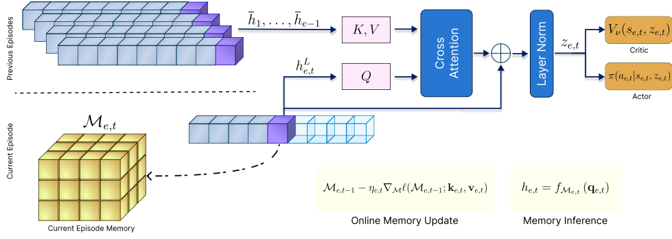
Figure 2: Overview of METTA. The current episode is processed by a within-episode neural memory to produce h_{e,t}^{(L)} . At the end of each episode, the final representation is stored as an episode summary \bar{h}_e . During later episodes, previous summaries are combined with the current representation to form the context representation z_{e,t} . The actor and critic condition on the current state s_{e,t} and z_{e,t} .
