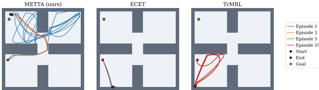
Figure 1: Exploration behavior on a sparse-reward PointMaze task (Fu et al., 2020) across adaptation episodes. Trajectories are shown for Episodes 1, 2, 5, and 10 of the same task. As interaction proceeds, METTA explores new regions and reduces repeated trajectories across episodes, suggesting more effective reuse of past exploration evidence in long-context adaptation. TrMRL (Melo, 2022) is difficult to scale to long multi-episode settings, while ECET (Shala et al., 2025) is limited by its short within-episode context.
