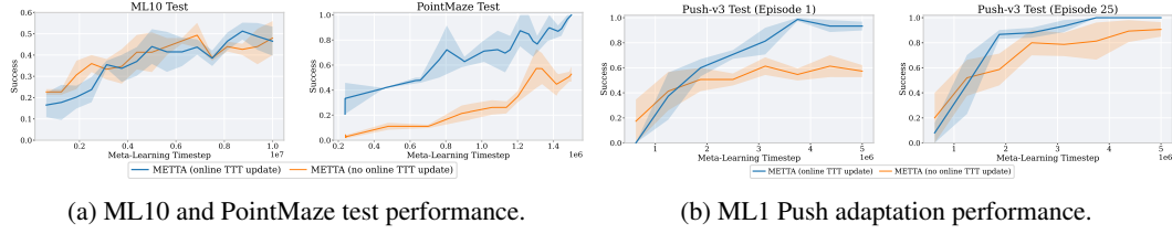
Figure 6: Effect of METTA test-time adaptation. The ML1 Push results report adaptation episodes 1 and 25 within each evaluation trial.
