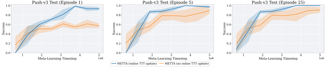
Figure 12: ML1 Push test performance at adaptation Episodes 1, 5, and 25 within each evaluation trial. The episode index denotes the progression of adaptation within the same trial.
