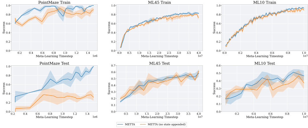
Figure 14: Effect of separating the current state from the learned task context. The default METTA provides s_{e,t} separately to the actor and critic, while the ablated variant must represent both state and task information through the learned context.
