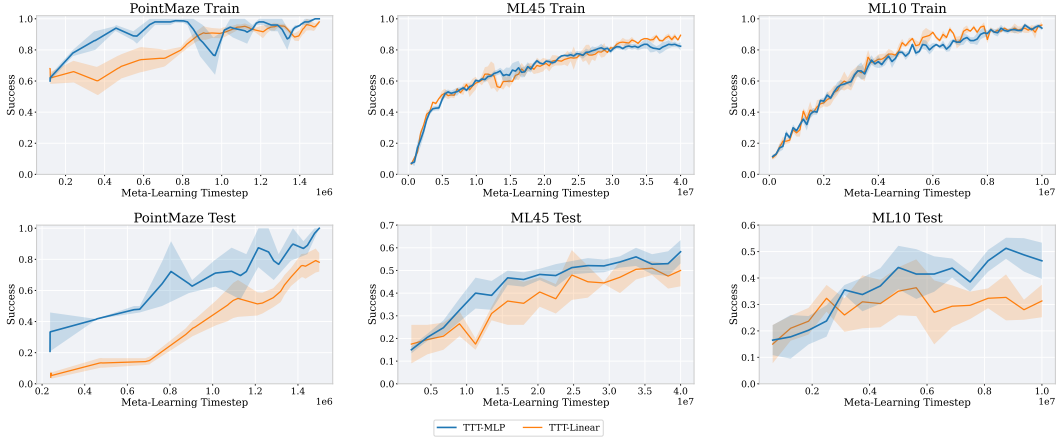
Figure 13: Effect of within-episode memory capacity. We compare the default TTT-MLP memory with the lighter TTT-Linear variant on PointMaze, ML45, and ML10.
