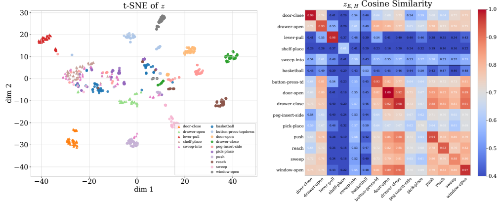
Figure 5: Structure of the learned context representations. Left: t-SNE visualization of z for all episodes. Circles denote training tasks and triangles denote test tasks. Right: pairwise cosine-similarity matrix computed from the final episode representation of each trial.
