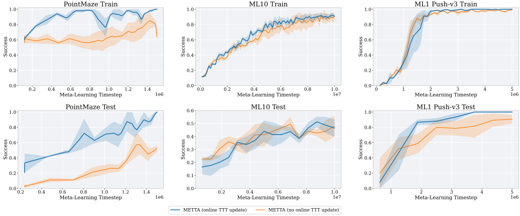
Figure 11: Complete online memory-update ablation on PointMaze, ML10, and ML1 Push. Top: training performance. Bottom: test performance.
