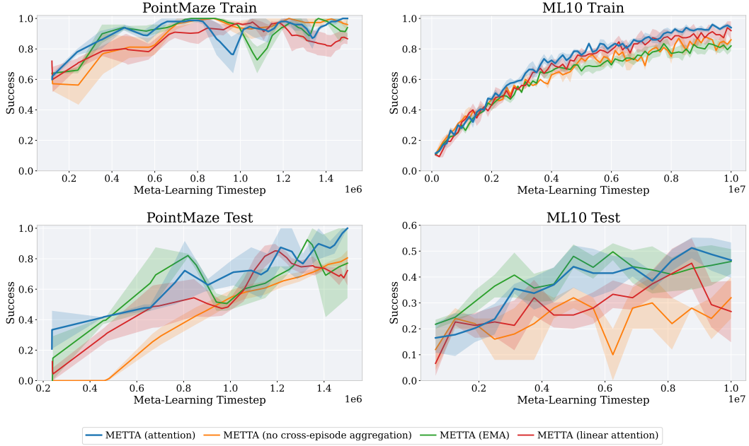
Figure 10: Comparison of cross-episode aggregation mechanisms in METTA on ML10 and PointMaze. All variants use the same within-episode neural memory.
