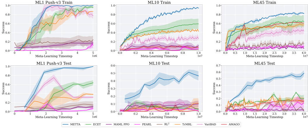
Figure 4: Meta-World success rate on ML1, ML10, and ML45. Top: evaluation on unseen task instances from task families used during meta-training. Bottom: evaluation on the Meta-World test benchmark, which contains unseen held-out task families for ML10 and ML45.
