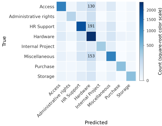
Fig. 5. TF-IDF + LR confusion matrix without abstention on the full test set ( n = 9,567 ). Color uses a square-root count scale; the three largest off-diagonal cells are labeled.
