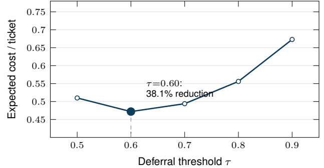
Fig. 3. TF-IDF + LR test cost over the predeclared threshold grid under (0, 1, 5). The calibration-selected \tau = 0.60 yields a 38.1 % reduction (95 % CI [35.7 %, 40.4 %]).
