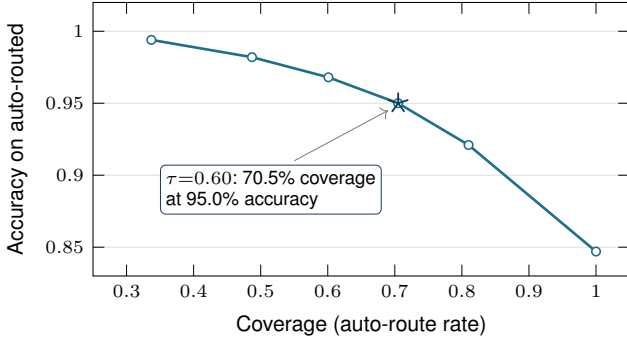
Fig. 4. TF-IDF + LR coverage–accuracy curve. The marked calibration-selected point routes 70.5 % of test tickets at 95.0 % accuracy.
