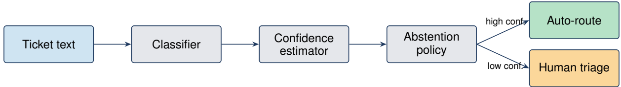
Fig. 1. Evaluation pipeline from ticket text to auto-routing or human triage, with prediction, confidence estimation, and abstention separated.
