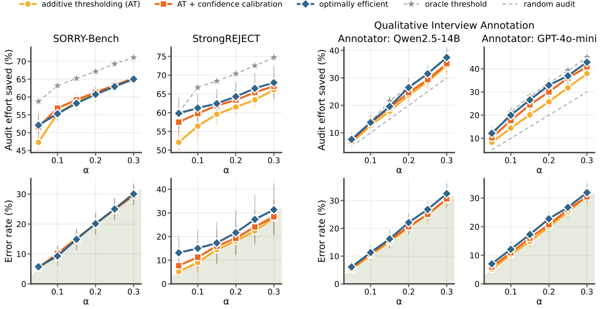
Figure 1: Error rate and audit effort saved on safety verification tasks.
