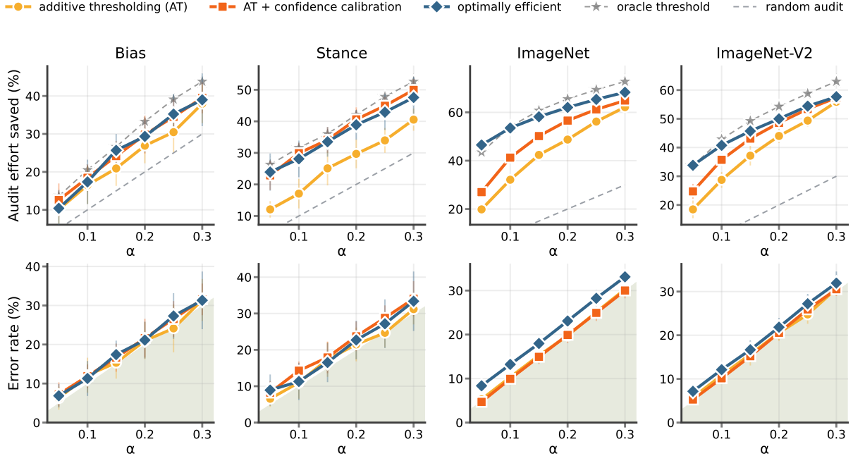
Figure 3: Error rate and audit effort saved on data labeling tasks.
