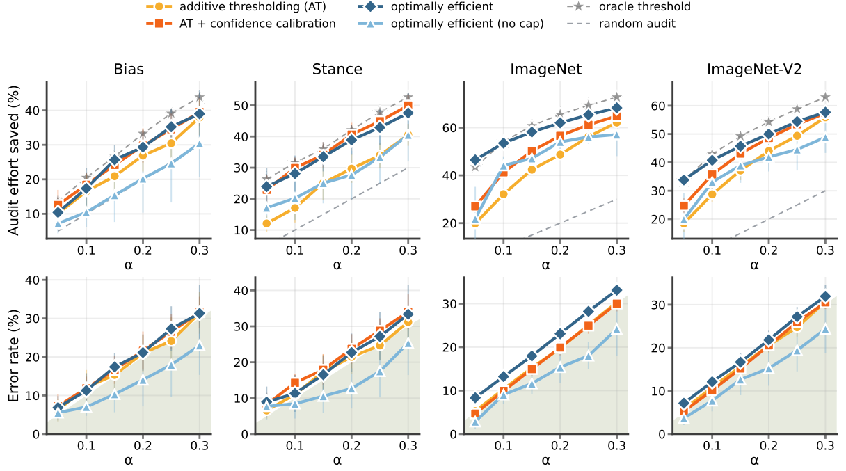
Figure 6: Error rate and audit effort saved on data labeling tasks, including both the capped and uncapped versions of optimally efficient auditing.
