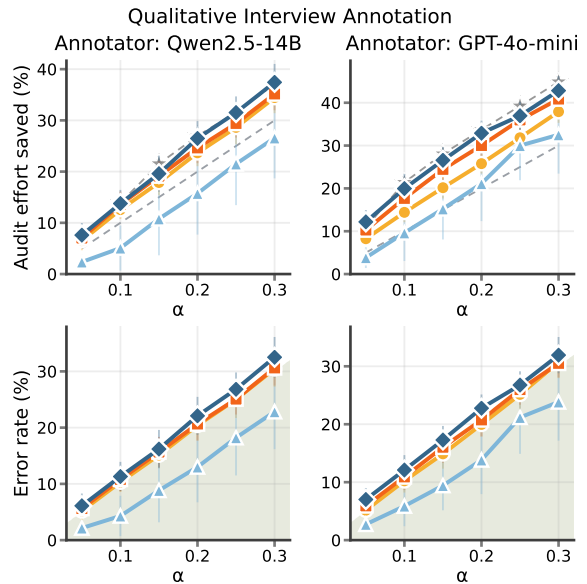
Figure 5: Error rate and audit effort saved on qualitative annotation of interview transcripts, including both the capped and uncapped versions of optimally efficient auditing.
