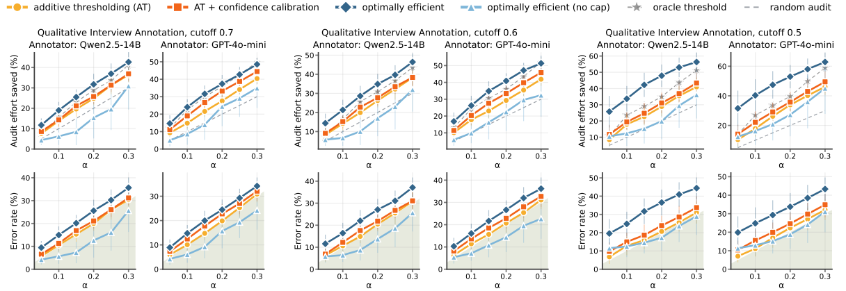
Figure 7: Error rate and audit effort saved on qualitative annotation of interview transcripts, with progressively sparser errors (cutoff = 0.7, 0.6, 0.5 going left to right), including both the capped and uncapped versions of optimally efficient auditing.
