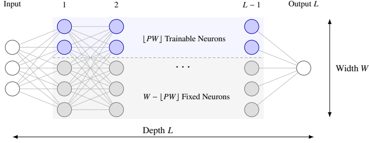
Figure 3. A P -trainable network with hidden layers of equal width W . Each hidden layer contains \lfloor PW \rfloor trainable neurons and W - \lfloor PW \rfloor fixed neurons. Thus, the network has O(PW^2L + W) trainable parameters out of O(W^2L) total parameters.
