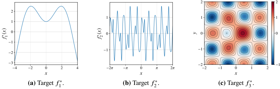
Figure 9. Target functions in the numerical experiments. Targets f_1^* and f_2^* are shown as curves, while f_3^* is shown as a heatmap, with color indicating the function value.
