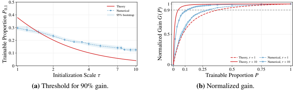
Figure 1. Phase transitions for two-layer spherical biased-ReLU P -trainable networks with d = 5 . Red curves are derived from the approximation bound, while blue curves show training results for a fixed RKHS target. Increasing the fixed initialization scale \tau \geq 1 raises the mismatch constant from its minimum at \tau = 1 . Both theory and training show qualitatively similar transition shapes and sharper transitions at larger \tau . Quantitative differences are expected because training also depends on finite sampling, the optimizer, and the training budget. Threshold P_{0.1} marks 90% normalized gain. Shaded bands indicate 95% bootstrap intervals. See experimental details in Appendix E.1.
