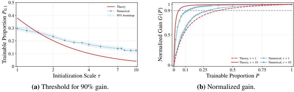
Figure 1 (reproduced). Theoretical and numerical phase transitions for two-layer spherical biased-ReLU P -trainable networks with d = 5 . Red curves are derived from the approximation bound, while blue curves show illustrative training results for a fixed RKHS target. Threshold P_{0.1} marks 90% normalized gain. Shaded bands indicate 95% bootstrap intervals.
