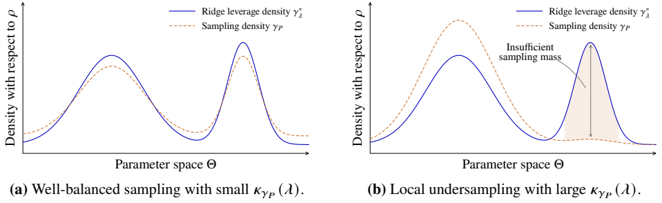
Figure 4. Schematic illustration of the mismatch factor \kappa_{\gamma_P}(\lambda) . The sampling density closely follows the ridge leverage density in (a), but assigns insufficient mass near the right peak in (b).
