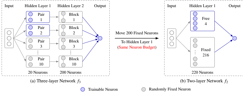
Figure 8. Architectural comparison with 220 hidden neurons and four trainable neurons. In (a), 20 first-layer neurons form 10 pairs, each feeding a block of 20 fixed neurons with tied incoming weights. In (b), the second-layer budget is reallocated to the single hidden layer. Only representative fixed neurons are shown.
