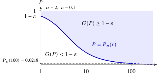
Figure 5. Minimum trainable proportion for 90% normalized gain, with \alpha = 2 and \varepsilon = 0.1 . Shaded region above P_\varepsilon(r) satisfies G(P) \geq 1 - \varepsilon . The endpoint at r = 1 represents the limit 1 - \varepsilon as r \rightarrow 1_+ .
