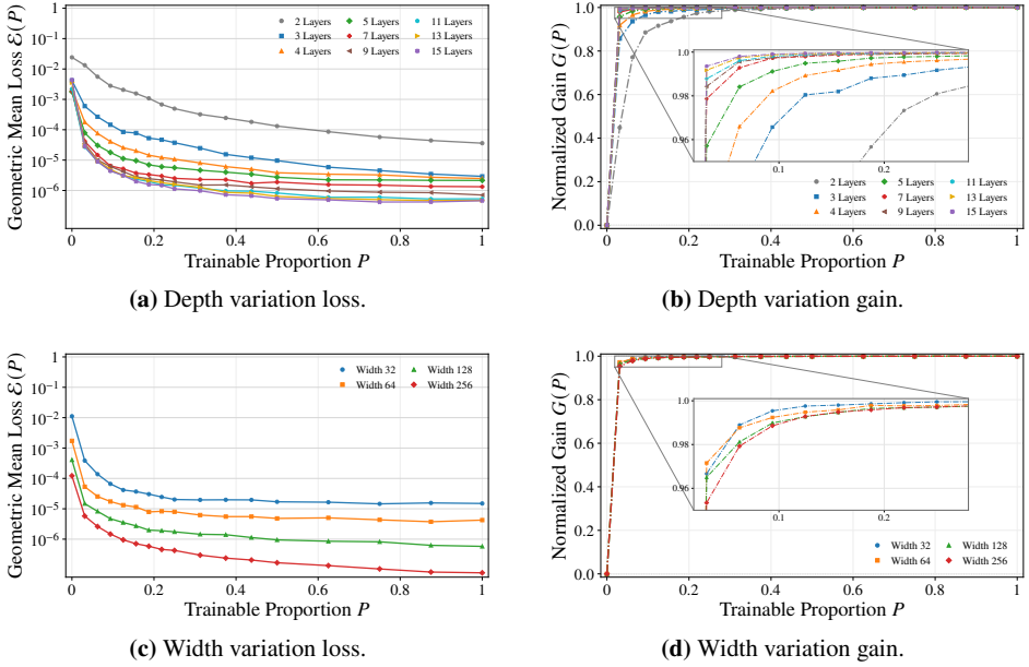
Figure 10. Training results for f_1^* with ReLU activation. The top and bottom rows show depth and width variation, respectively. The left column reports the geometric mean of the best training loss across 21 repetitions, and the right column shows the normalized gain.
