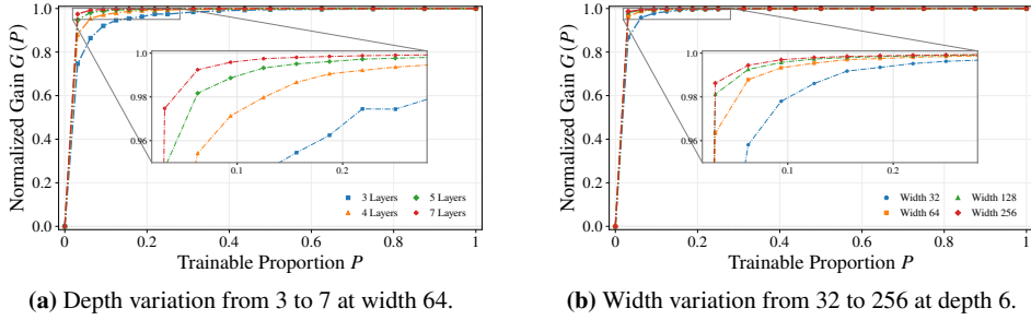
Figure 2. Representative numerical normalized gains for P -trainable ReLU networks on a surface target function. Gains are normalized by the observed loss reduction between P = 0 and P = 1 . Both depth and width comparisons show rapid gains at small P , followed by diminishing gains.
