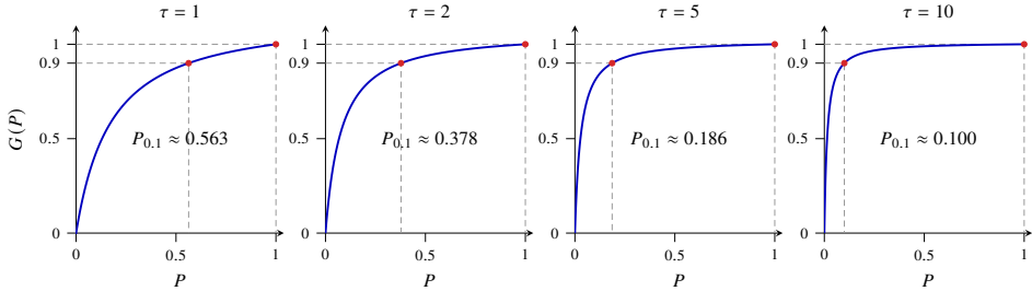
Figure 7. Normalized gain predicted by the spherical biased-ReLU bound in dimension d = 20 ( \alpha = 22/19 ) for increasing \tau . Gray dashed guides mark 90% gain and the endpoint G(1) = 1 .
