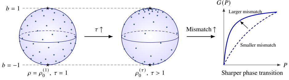
Figure 6. Scaled spherical initialization. Increasing \tau shifts fixed-neuron parameters toward the poles b = \pm 1 . The right panel schematically shows how greater mismatch can sharpen the gain at small P .
