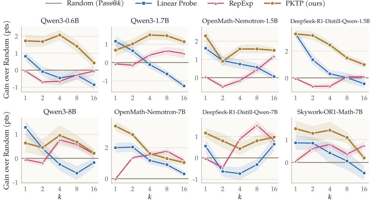
Figure 9: Gain in pass@ k over random pruning with N = 48 . As in Fig. 3, with a pool of N = 48 rollouts drawn from the 128 generated for each problem and T = 4000 .
