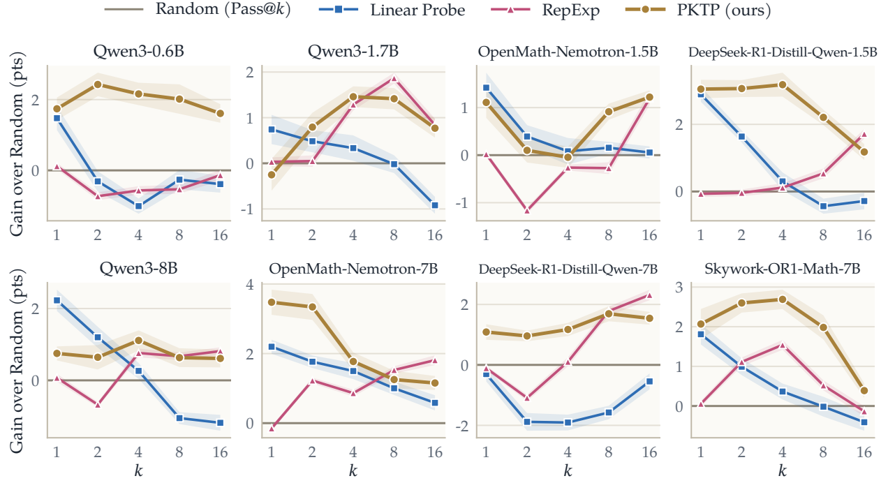
Figure 13: Gain in pass@k over random pruning with N = 112 . As in Fig. 3, with a pool of N = 112 rollouts drawn from the 128 generated for each problem and T = 4000 .
