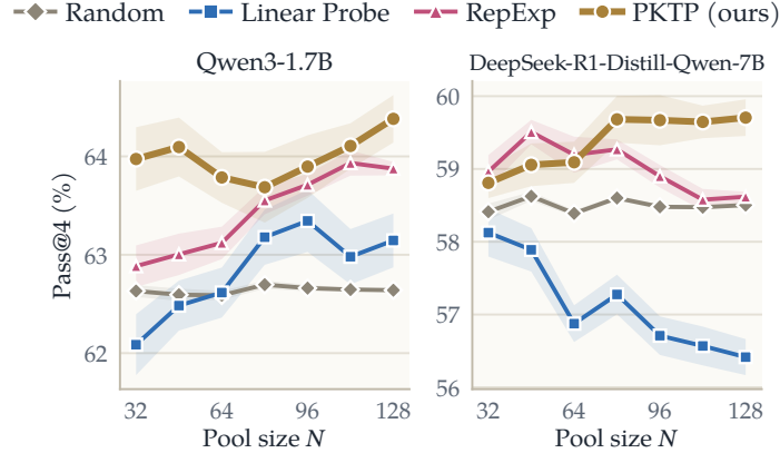
Figure 7: PKTP leads once the pool is large enough. Pass@4 on Qwen3-1.7B and DeepSeek-R1-Distill-Qwen-7B as the pool size N grows from 32 to 128, with T = 4000 . PKTP is the best method for every N on Qwen3-1.7B and from N = 80 on DeepSeek-R1-Distill-Qwen-7B, where the Linear Probe falls as the pool grows and stays below Random. Bands are one standard error.
