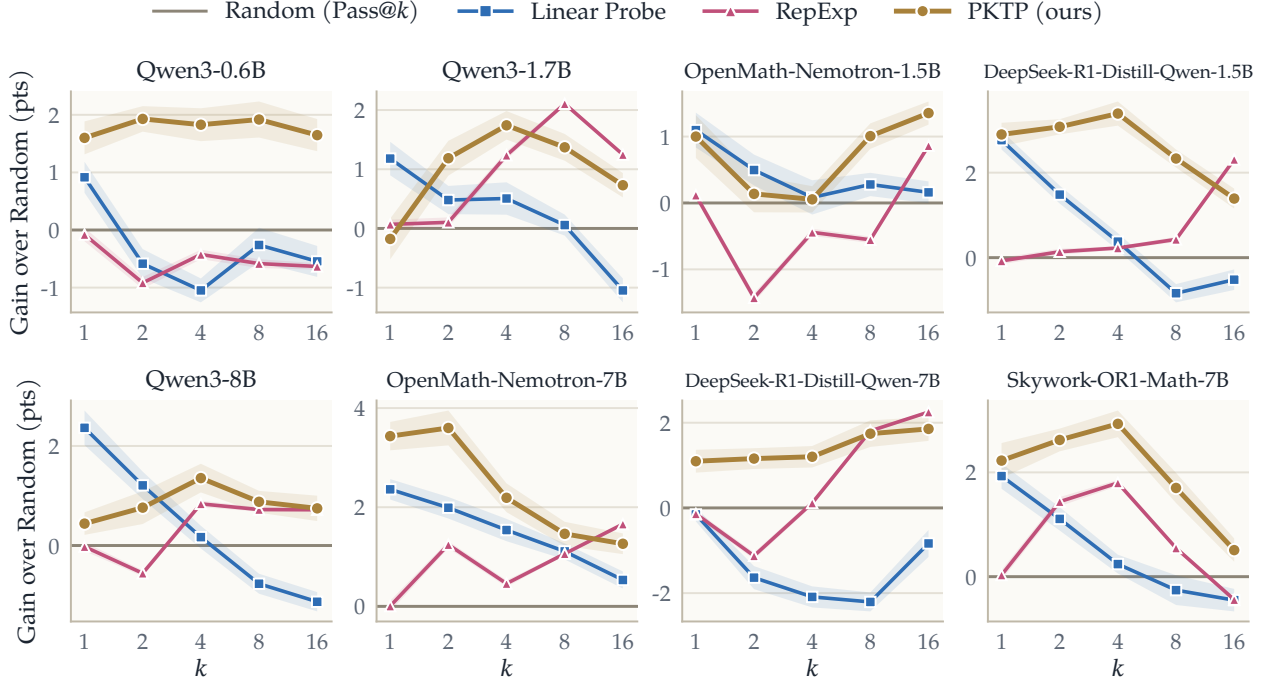
Figure 3: Gain in pass@k over random pruning. For every model, the pooled pass@ k of each pruning policy minus that of Random (Pass@ k ), in percentage points, as a function of the number k of rollouts kept, with a band of one standard error of the repetition-by-repetition difference. The absolute numbers are in Table 1 and the per-benchmark breakdown in Appendix D.
