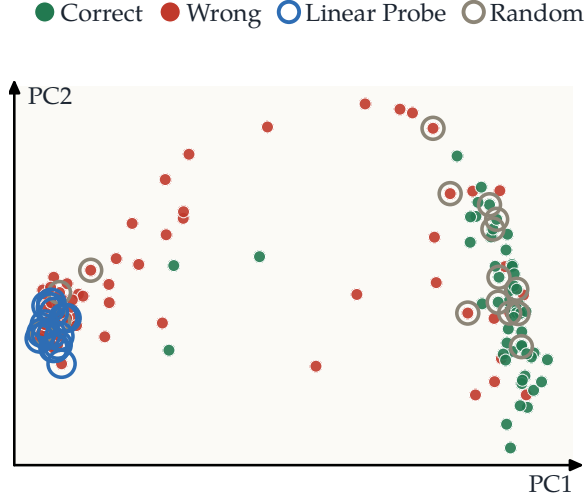
Figure 4: Linear Probe keeps a cluster of rollouts that fail together. The 128 rollouts of one problem (Qwen3-8B, AMO-Bench), projected on the first two principal components of their representations, with correct rollouts in green and wrong rollouts in red. The 16 rollouts ranked highest by the Linear Probe (blue rings) lie close together and are all wrong, while 16 random picks (gray rings) include 7 correct rollouts.
