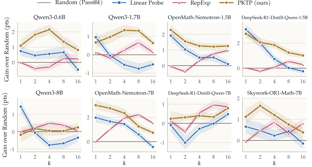
Figure 8: Gain in pass@k over random pruning with N = 32 . As in Fig. 3, with a pool of N = 32 rollouts drawn from the 128 generated for each problem and T = 4000 .
