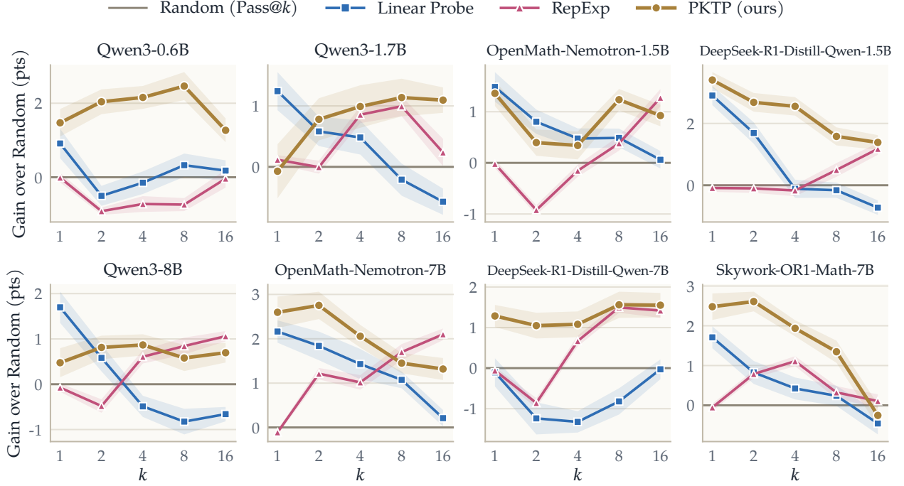
Figure 11: Gain in pass@ k over random pruning with N = 80 . As in Fig. 3, with a pool of N = 80 rollouts drawn from the 128 generated for each problem and T = 4000 .
