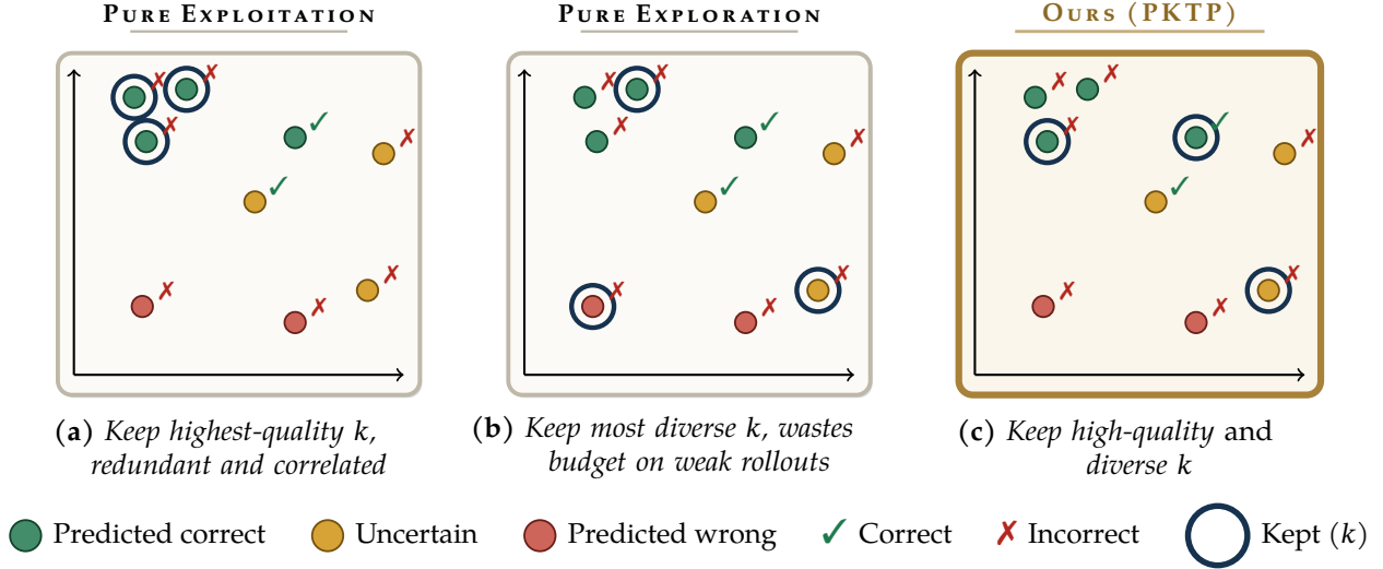
Figure 2: Conceptual illustration. The same pool of candidate rollouts, positioned by their partial rollout representations in embedding space, under three pruning strategies. Each rollout is colored by its predicted correctness and marked ✓/✗ by its actual outcome; the k = 3 kept rollouts are ringed. (a) Pure exploitation keeps the highest-scoring rollouts, but they are correlated and cluster together, so they miss the correct rollout. (b) Pure exploration keeps a maximally diverse subset yet spends its budget on low-quality rollouts, also missing it. (c) Our method optimizes \text{pass}@k directly over the kept subset, balancing quality and diversity, and retains the correct rollout.
