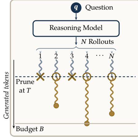
Figure 1: Test-time pruning. Only k of the N rollouts (ringed) continue past the cutoff T , up to the budget B .
