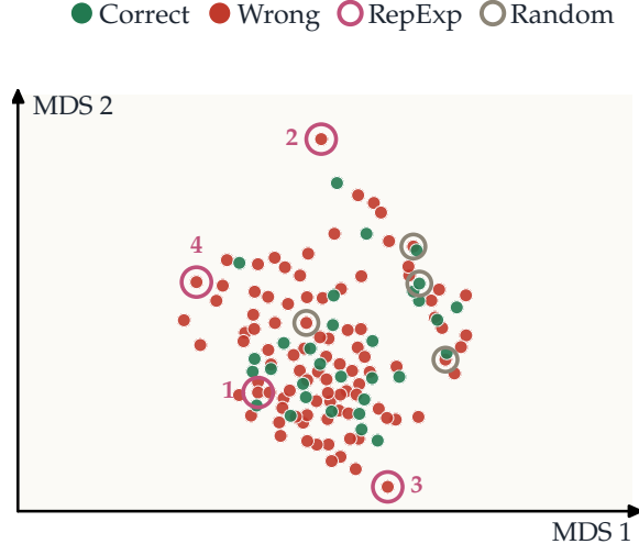
Figure 5: RepExp keeps outliers that are unlikely to be correct. The 128 rollouts of one problem (Qwen3-8B, Omni-MATH), embedded in two dimensions by multidimensional scaling of their representations, with correct rollouts in green and wrong rollouts in red. After a random first pick, RepExp (pink rings, numbered in pick order) selects rollouts far from the rest, and all 4 of its picks are wrong, while 4 random picks (gray rings) include 1 correct rollout.
