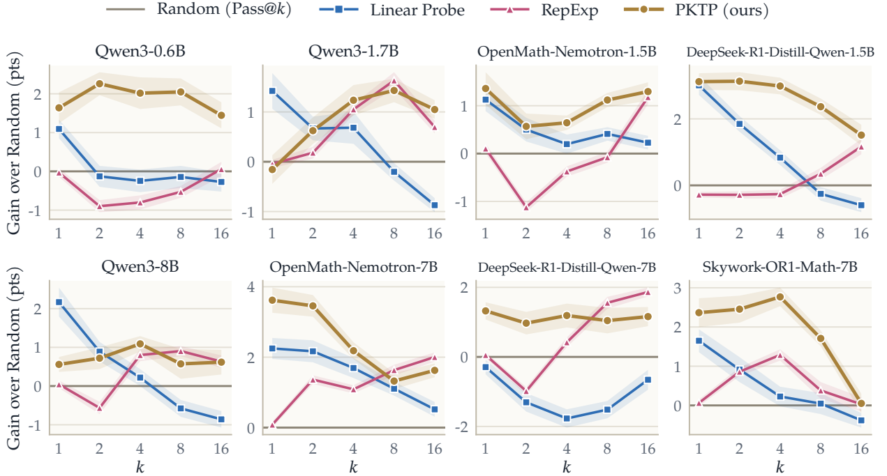
Figure 12: Gain in pass@ k over random pruning with N = 96 . As in Fig. 3, with a pool of N = 96 rollouts drawn from the 128 generated for each problem and T = 4000 .
