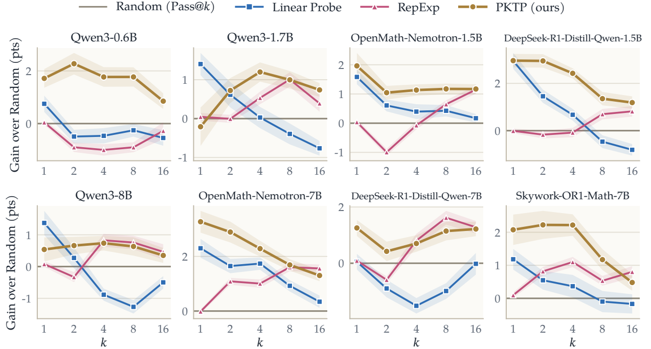
Figure 10: Gain in pass@ k over random pruning with N = 64 . As in Fig. 3, with a pool of N = 64 rollouts drawn from the 128 generated for each problem and T = 4000 .
