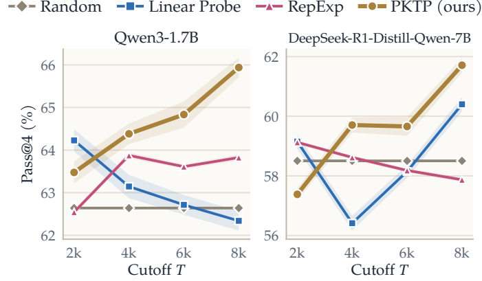
Figure 6: A later cutoff improves PKTP. Pass@4 on Qwen3-1.7B and DeepSeek-R1-Distill-Qwen-7B as the cutoff T grows from 2000 to 8000 tokens, with N = 128 . PKTP is the best method for every T \geq 4000 and keeps improving with longer prefixes, while the Linear Probe and RepExp gain much less, and the Linear Probe on Qwen3-1.7B even drifts below Random. Bands are one standard error.
