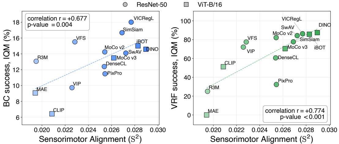
Figure 11 | Sensorimotor Alignment ( S^2 ) of frozen vision encoders correlates with downstream policy success rate. Points represent the 14 frozen backbones of Hu et al. [19], scored by S^2 on DROID without policy training. The vertical axis shows the interquartile mean (IQM) of task success rates over 21 tasks, using low-data behavior cloning (left) or reinforcement learning with visual reward functions (right).
