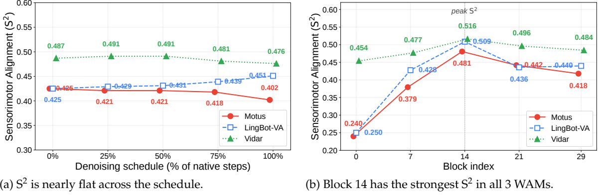
Figure 10 | Sensorimotor Alignment ( S^2 ) is already high at early denoising steps and peaks at mid-depth blocks. For 3 world action models (WAMs), (a) S^2 remains nearly flat across denoising, suggesting early-step features already align with robot trajectories; (b) schedule-averaged S^2 peaks at Block 14, showing peak alignment at mid-depth.
