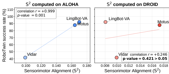
Figure 12 | Sensorimotor Alignment ( S^2 ) is sensitive to a mismatch in arm configuration. For 3 world action models (WAMs) evaluated on bimanual RoboTwin, the matched bimanual ALOHA reference (left) recovers the success-rate ordering, while the single-arm DROID reference (right) weakens the correlation. S^2 thus reflects whether reference data matches the target arm configuration.
