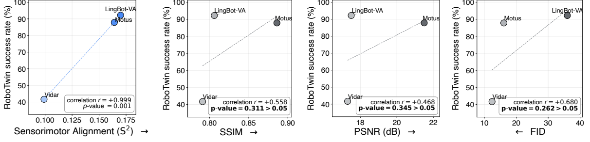
Figure 5 | Sensorimotor Alignment ( S^2 ) correlates with WAM success rate more closely than video-quality metrics. For 3 world action models (WAMs) evaluated on RoboTwin, video-quality metrics (SSIM, PSNR, FID) show no significant correlations with task success. In contrast, only S^2 correctly recovers the success-rate ordering. Only 3 of the 6 WAMs are compared because the others do not generate future video during closed-loop task evaluation.
