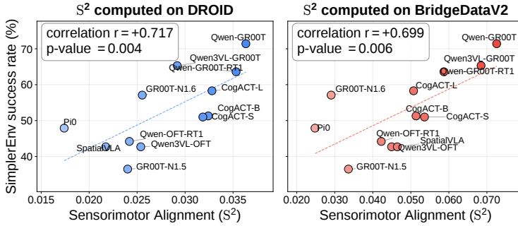
Figure 6 | The correlation transfers across reference datasets. For 12 vision-language-action models, Sensorimotor Alignment ( S^2 ) on DROID (left) and BridgeDataV2 (right) correlates strongly with the same SimplerEnv-WidowX task success rates, so the correlation does not depend on the reference dataset.
