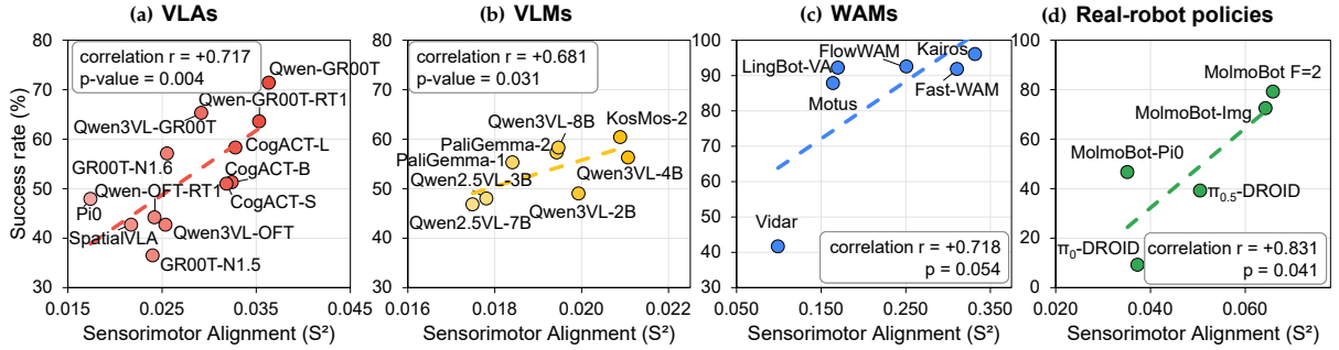
Figure 3 | Sensorimotor Alignment ( S^2 ) correlates with task success across model families and in simulated and real-world evaluations. Each panel plots offline S^2 (x-axis) against downstream task success rate (y-axis) for (a) fine-tuned vision-language-action models (VLAs), (b) raw vision-language models (VLMs), (c) world action models (WAMs), and (d) real-robot policies. For raw VLMs, task success is measured after VLA fine-tuning. These correlations (Pearson’s r ; unadjusted one-tailed p -values) support S^2 as an offline proxy across model families.
