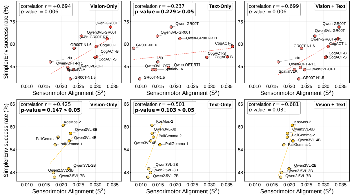
Figure 8 | Fine-tuned VLAs rely mainly on visual rather than language representations. We correlate Sensorimotor Alignment ( S^2 ) from vision, text, and joint vision-text features (left to right) with SimplerEnv task success rate. Top: For fine-tuned vision-language-action models (VLAs), vision and joint features correlate similarly strongly, while text features correlate weakly. Bottom: For raw vision-language models (VLMs), joint-feature S^2 correlates with task success after VLA fine-tuning, while neither modality alone reaches significance.
