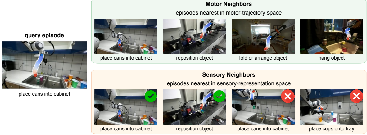
Figure 2 | Measuring Sensorimotor Alignment ( S^2 ) by nearest-neighbor overlap. For the query episode (left), sensory neighbors (bottom right) have similar vision-text features, and motor neighbors (top right) have similar trajectories. Green checks mark shared neighbors; red crosses mark neighbors found only in the sensory set. A larger overlap means that episodes with similar sensory representations also follow similar motor trajectories.
