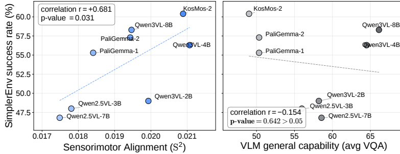
Figure 4 | Sensorimotor Alignment ( S^2 ) correlates with VLA success rate where VQA scores do not. Across 8 raw vision-language models (VLMs) [57], S^2 (left) correlates strongly with SimplerEnv task success after fine-tuning into vision-language-action models (VLAs), whereas visual question answering (VQA) scores (right) show virtually no correlation.
