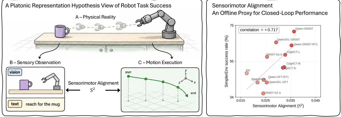
Figure 1 | Left: We test the Platonic Representation Hypothesis (PRH) in robotics, using image-text features as the sensory representation and end-effector trajectories as the motor representation: a more capable embodied model should have sensory representations that align more closely with this motor representation. To validate this, we define Sensorimotor Alignment ( S^2 ). Right: We measure S^2 across 12 vision-language-action models (VLAs) and find that S^2 correlates positively with SimplerEnv task success rate (Pearson r = +0.717 ), providing empirical support for this PRH-inspired view of embodiment.
