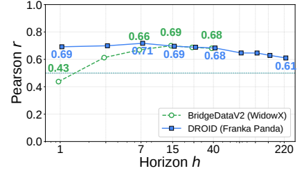
Figure 7 | Stable correlations across horizons. For 12 vision-language-action models, Sensorimotor Alignment ( S^2 ) and SimplerEnv-WidowX success rate have Pearson r > 0.5 at nearly all tested horizons h (future steps) on DROID and BridgeDataV2.
