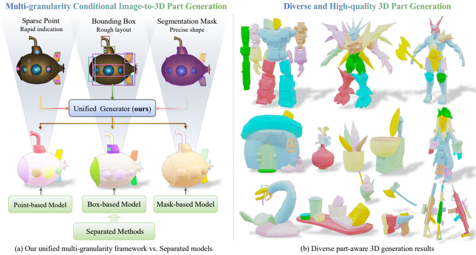
Figure 1: (a) Our unified framework integrates variable-granularity geometric prompts from sparse points to dense masks into one model for flexible part control. (b) The proposed method produces high-fidelity, semantically coherent 3D parts across diverse object categories.
