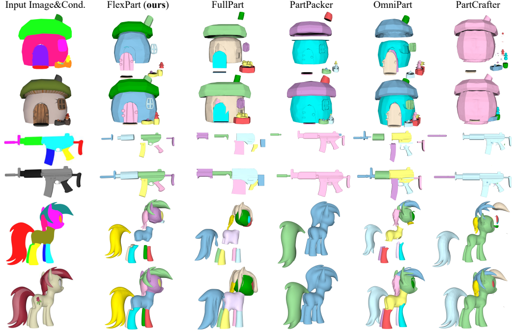
Figure 3: Qualitative results of different methods. The upper row shows exploded views for inspecting individual parts, and the lower row shows the assembled meshes. Our method uses masks as input, while other methods are evaluated with their respective input conditions.
