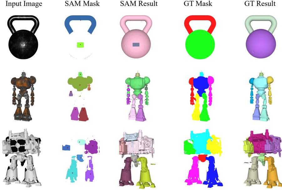
Figure 7: Qualitative evaluation of the SAM-based interface. We compare generation results under two input conditions across diverse examples. SAM : masks generated by SAM from a single point prompt sampled near the visual center. GT : ground-truth segmentation masks.
