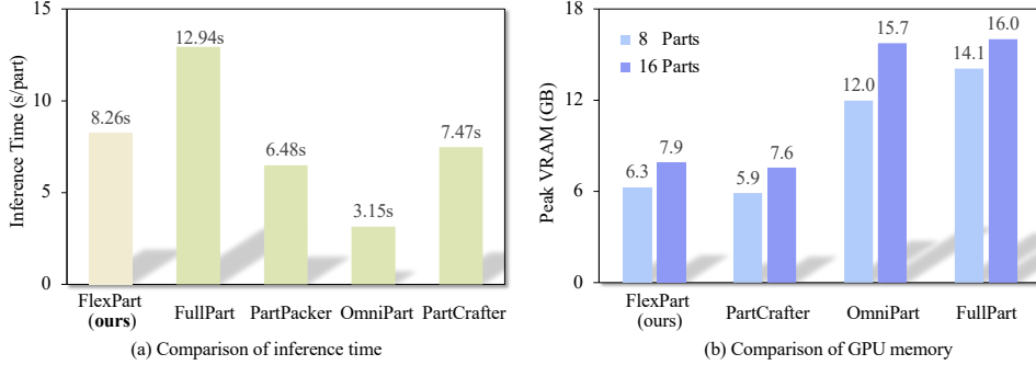
Figure 5: Efficiency comparison between FlexPart and other methods.
