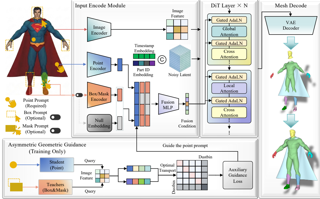
Figure 2: Overview of the FlexPart framework. FlexPart supports point, box, and mask prompts, with points as the minimal input. The noisy latent, part ID, and timestep are jointly conditioned on encoded prompts, where learnable null embeddings replace missing inputs. The fused condition modulates each DiT layer for part generation via gated adaptive layer normalization. During training, a multi-granularity geometric guidance branch aligns weak and strong priors via optimal transport.
