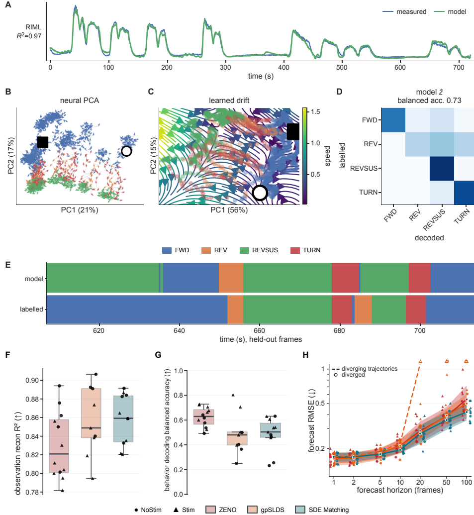
Figure 4: Whole-brain calcium dynamics in C. elegans A) Example ZENO reconstruction of RIML neuron. B-C) ZENO recovers limit cycles. D-E) Inferred latents are consistent with known behavioral labels. Model performance compared to baselines on F) reconstruction R^2 , G) behavior decoding accuracy, and H) forecasting RMSE. Points represent individual worms, separated into NoStim and Stim conditions. Error bars are 1SD.
