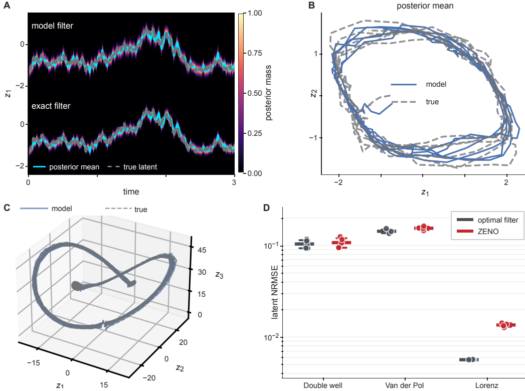
Figure 2: Latent Inference of Simulated Dynamical Systems. A) Exact filtering distribution for the double well system vs filtering posterior distribution estimated by ZENO. B) Latent Posterior Mean Estimate for the Van Der Pol System. C) Latent Trajectory Inference for the Lorenz Attractor. D) Comparison of ZENO’s normalized root mean squared error with the exact optimal filter for each system.
