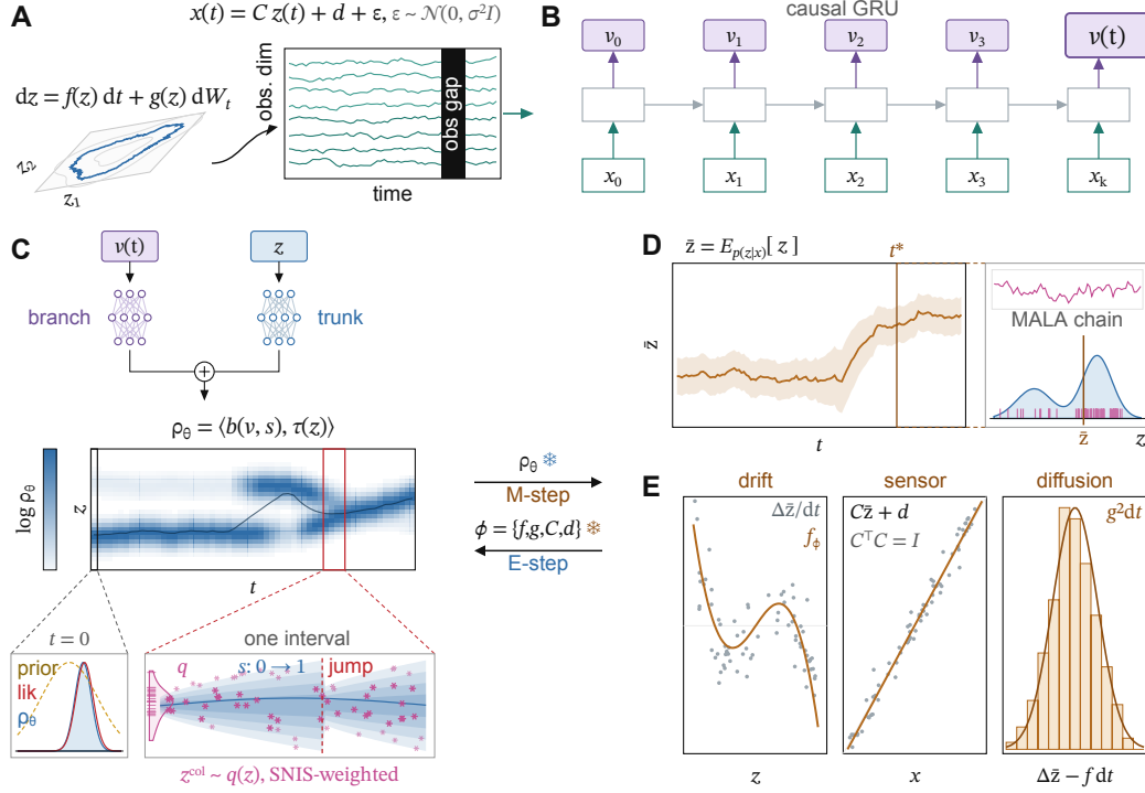
Figure 1: Architecture Diagram. A) Generative Model. B) Causal GRU encodes observations into context trajectory. C) Context trajectory is fed into the branch of a Deep Operator Network along with substeps to produce basis functions. Trunk network can be queried at any z and outputs \log \rho_\theta , the unnormalized log density. IC loss between the learned posterior and an IC prior \mathcal{N}(0, I) combined with Fokker Planck Residual Loss between observations and Jump Loss at observations D) Posterior Expectation \bar{z} = \mathbb{E}_{p(z|x)}[z] computed through MCMC sampling. E) Dynamics and Observation Parameters fit by regressing against \bar{z}
