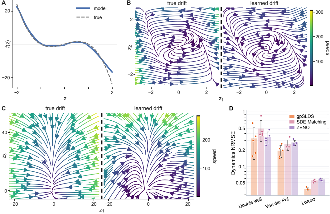
Figure 3: ZENO Drift Estimation Performance. A) True cubic drift of double well (dashed line) overlaid with model estimate. B) True Van Der Pol Vector field (Left) vs Model’s inferred Vector Field. C) Lorenz Attractor Dynamics plotted in the xz plane. D) Model’s NRMSE performance compared to baselines. Dots represent seeds and error bars are 1 SD.
