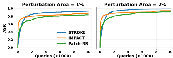
Figure 2: ASR comparison at nominal area settings on ResNet-50. Attack success rate (ASR) versus query budget on ImageNet for STROKE, IMPACT, and Patch-RS at nominal 1% and 2% area settings.
