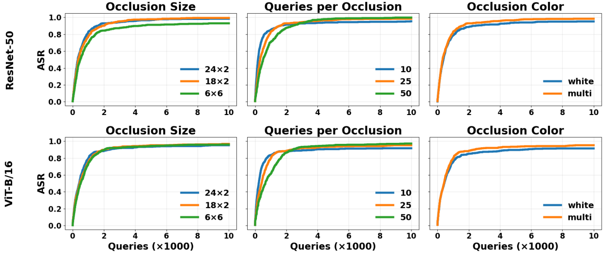
Figure 4: STROKE ablations at a nominal 2% coverage threshold and 10k-query limit (untargeted). ASR versus queries on ImageNet for ResNet-50 (top row) and ViT-B/16 (bottom row). We ablate (left) occlusion size ( \ell \times w ) for POQB = 25, color = multi, (middle) queries per occlusion (POQB) for size = 24x2, color = multi, and (right) occlusion color mode for POQB = 25, size = 24x2.
