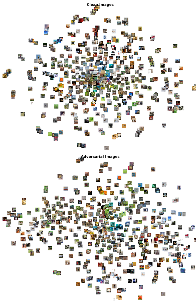
Figure 6: t-SNE visualization of ResNet50 feature embeddings for clean images (top) and adversarial images generated by STROKE (bottom). Each point is rendered as a thumbnail of the corresponding image. Adversarial perturbations lead to a noticeable redistribution of samples in the embedding space compared to the clean inputs.
