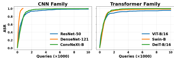
Figure 3: Attack success rate (ASR) vs. Queries for STROKE. Results at a nominal 2% pixel-coverage threshold for CNNs (ResNet-50, DenseNet-121, ConvNeXt-B) and Transformers (ViT-B/16, Swin-B, DeiT-B/16). STROKE achieves high success rates within a few thousand queries.
