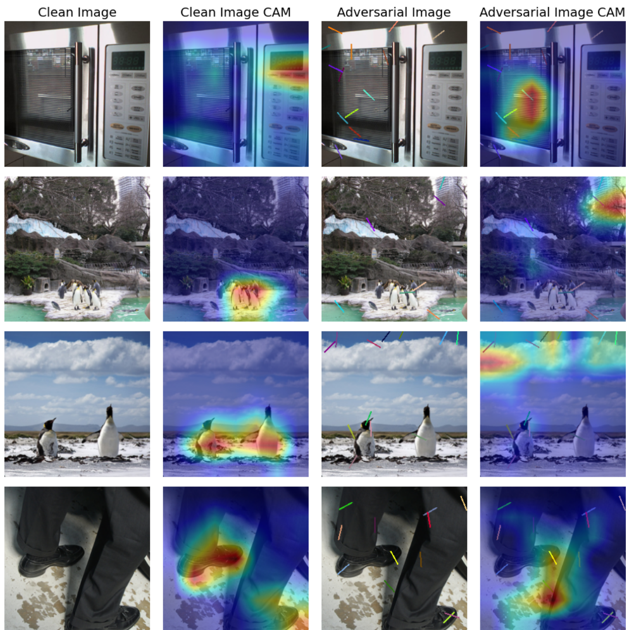
Figure 5: Grad-CAM visualizations for representative examples at the nominal 2% pixel-coverage threshold and 10k-query limit on ResNet50. Columns show the clean image, the corresponding Grad-CAM map, the adversarial image produced by STROKE, and the Grad-CAM map of the adversarial prediction. The attention regions often shift away from the original object regions after the attack.
