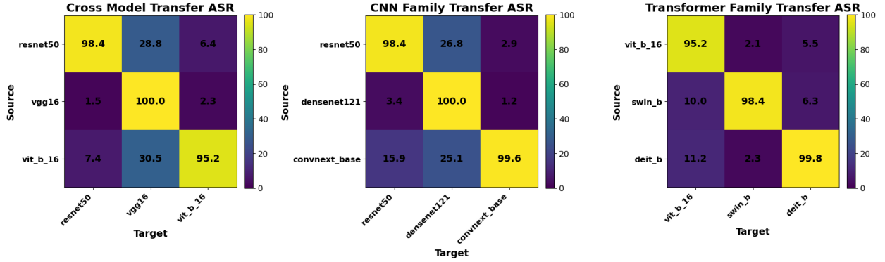
Figure 7: Transferability of adversarial examples generated by STROKE across different architectures. Rows correspond to the source model used to generate adversarial examples, and columns correspond to the target model used for evaluation. Each cell reports the attack success rate (ASR, %). Results are shown for (left) cross-model transfer among commonly used architectures, (middle) transfer within CNN-based models, and (right) transfer within transformer-based models at a nominal 2% coverage threshold and 10k-query limit.
