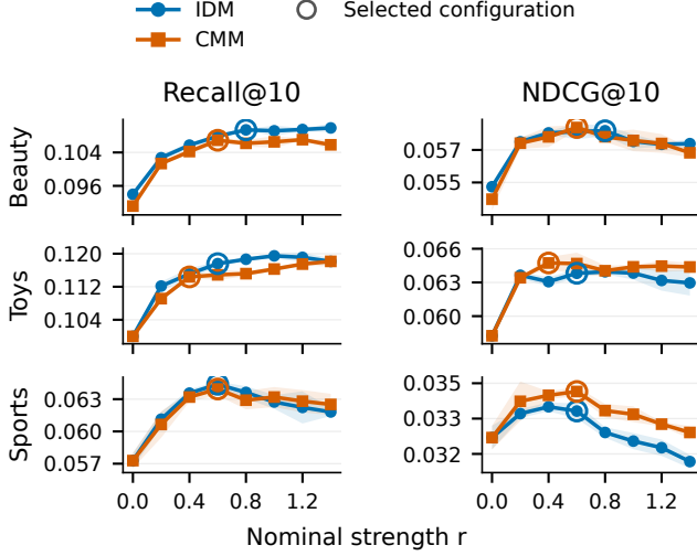
Figure 2: Distillation-strength sensitivity. Bands denote \pm one sample standard deviation over three runs, and rings indicate the validation-selected configurations. The r = 0 controls match the learning rate of each curve and coincide on Toys and Sports.
