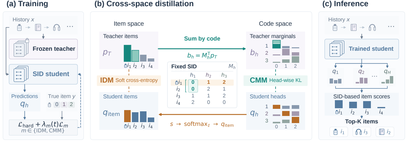
Figure 1: Overview of item- and code-space knowledge distillation for parallel semantic-ID recommendation. (a) A parallel SID student learns from hard labels and a frozen teacher using either IDM or CMM. (b) Fixed assignments M_h connect teacher item probabilities with student code predictions. IDM matches distributions over valid catalogue items; CMM matches teacher-derived code marginals with student head distributions. (c) At inference, the student predicts SID codes in parallel and ranks valid items without the teacher.
