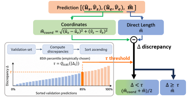
Fig. 3: Illustration of the coordinate-length consistency mechanism with a threshold selection based on validation-set discrepancies.
