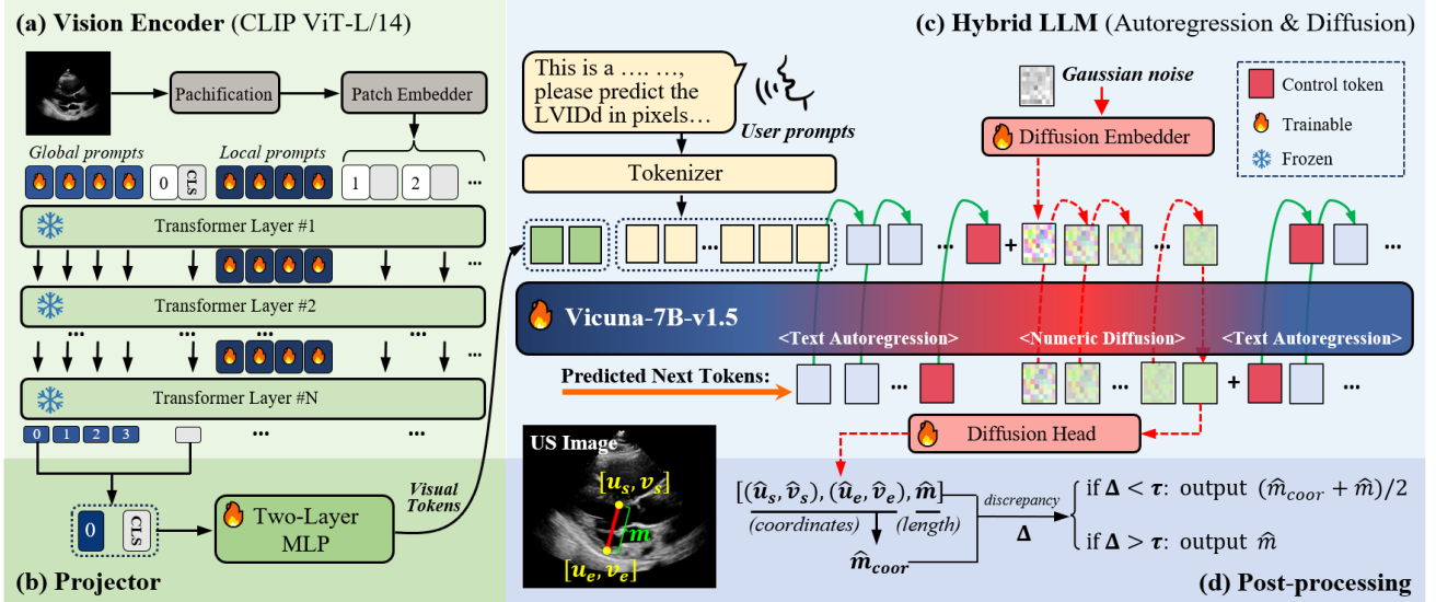
Fig. 2: Overview of HAD-VLM for prompt-conditioned quantitative ultrasound measurement. The framework comprises (a) an prompt-adapted vision encoder, (b) a projector, (c) a hybrid LLM, and (d) a post-processing module. It integrates autoregressive text generation with diffusion-based continuous measurement prediction via a 5-tuple measurement representation and a coordinate-length consistency mechanism.
