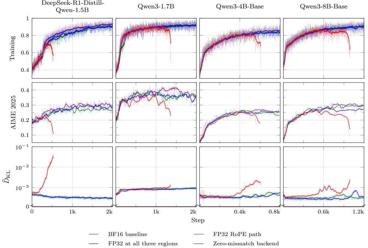
Figure 3 Training accuracy (top), AIME 2025 accuracy (middle), and inference-training discrepancy \hat{D}_{KL} (bottom; Eq. 3). Observations are smoothed using causal trailing means over 20 observations for training accuracy and \hat{D}_{KL} and five observations for AIME 2025 accuracy. The BF16 baseline collapses for every model; the FP32 RoPE path, FP32 at all three regions, and Zero-mismatch backend remain stable.
