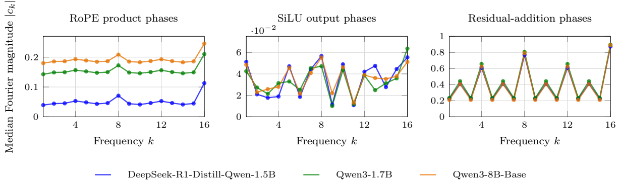
Figure 5 Fourier magnitudes for RoPE products, SiLU outputs, and residual sums. Each point summarizes |\hat{c}_{\ell,s,k}| by its median across layers. For residual addition, the magnitudes of the attention and MLP residual sums are averaged within each layer before taking the median. The panels use different vertical scales.
