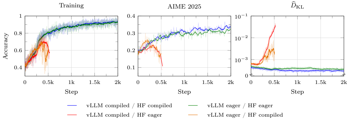
Figure 1 Training accuracy, AIME 2025 accuracy, and the inference–training discrepancy \hat{D}_{\text{KL}} (Eq. 3) for the four execution-mode conditions. Observations are smoothed using causal trailing means over 20 observations for training accuracy and \hat{D}_{\text{KL}} and five observations for AIME 2025 accuracy. Both aligned conditions maintain high accuracy; both crossed conditions initially improve and then lose accuracy.
