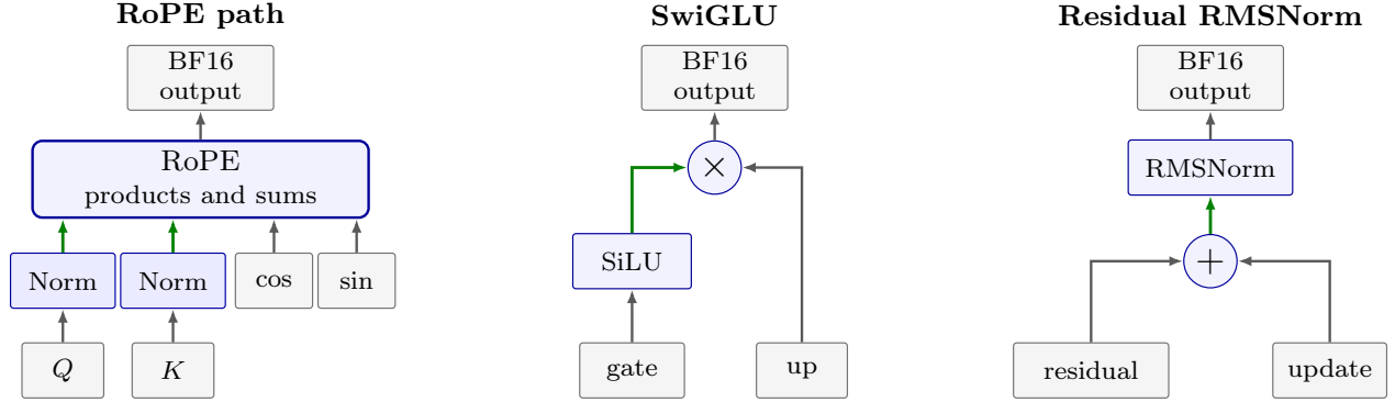
Figure 2 The three Qwen regions in which fusion changes rounding locations. Green arrows carry intermediates retained in FP32 under fusion and rounded to BF16 between separate operations. RoPE products and sums are also retained in FP32 under fusion. Region outputs are BF16 in both cases. Q/K normalization, when present, is part of the RoPE path.
