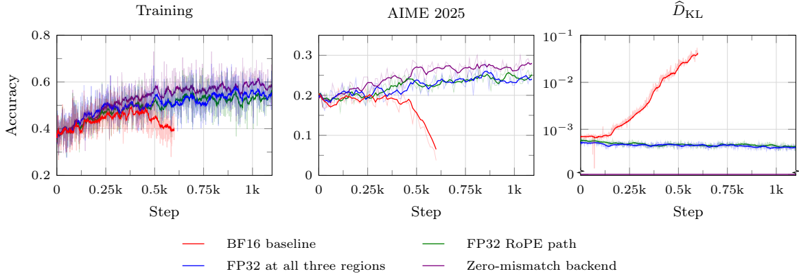
Figure 6 Training accuracy, AIME 2025 accuracy, and \hat{D}_{KL} (Eq. 3) for DeepSeek-R1-Distill-Qwen-1.5B trained on DAPO-Math-17k. Observations are smoothed using causal trailing means over 20 observations for training accuracy and \hat{D}_{KL} and five observations for AIME 2025 accuracy. The BF16 baseline loses accuracy after initial improvement; both rounding-location alignments and the Zero-mismatch backend sustain training progress.
