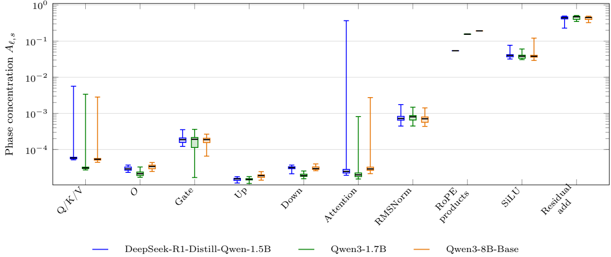
Figure 4 Layer distributions of the 16-frequency phase concentration. The center line is the layer median, boxes span the first and third quartiles, and whiskers show the full range. The three intermediates at changed rounding locations are markedly more nonuniform than the other signals.
