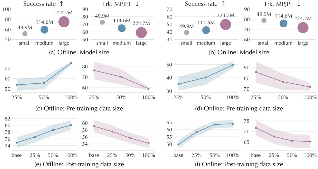
Figure 4: Scaling behavior of ViT-H on the video-only test set. Panels (a,b) vary the model size, with marker size indicating the number of parameters, panels (c,d) the percentage of pre-training data, and panels (e,f) the percentage of post-training data, where base denotes the pre-trained generator. Panels (a) to (d) use generators without post-training. Shaded regions denote 95% confidence intervals.
