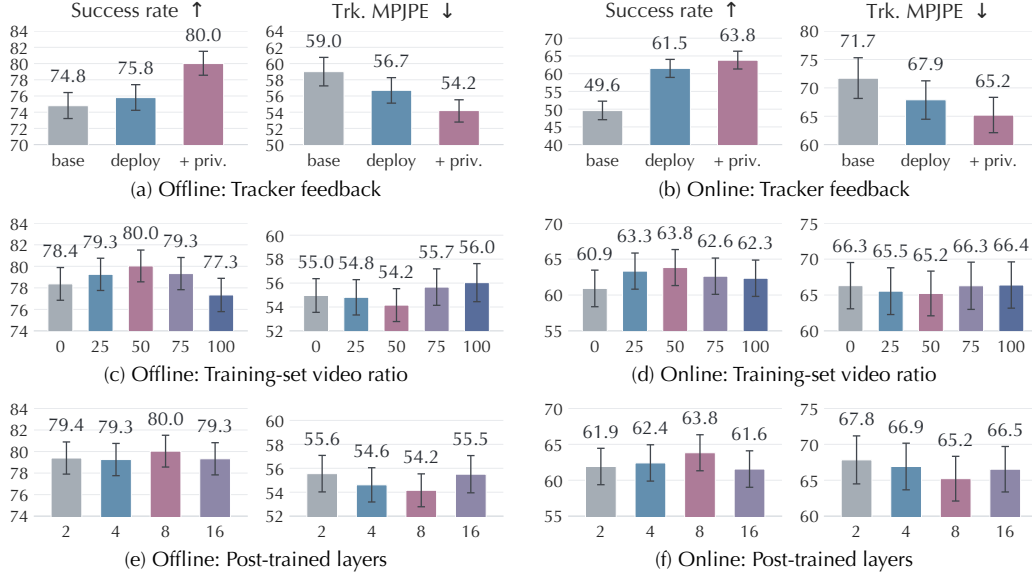
Figure 3: Analysis of DPO post-training on the video-only test set. Panels (a,b) vary the tracker feedback, from the pre-trained generator (base) to post-training with rewards from the deployable tracker alone (deploy) and with the privileged tracker added (+ priv.). Panels (c,d) vary the amount of in-distribution pre-training set data relative to video-only data during post-training, and panels (e,f) the number of final Transformer layers updated during post-training. Error bars denote 95% confidence intervals.
