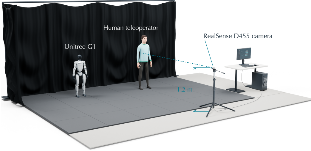
Figure A1: Video teleoperation setup. A RealSense D455 camera mounted 1.2 m above the ground, with its optical axis approximately parallel to the ground, records RGB video of the teleoperator, and the Unitree G1 stands beside the teleoperator.
