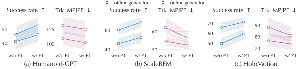
Figure 5: Post-training gains transfer to trackers not used in post-training. Motions generated by the offline (circles) and autoregressive (squares) generators on the video-only test set are executed by (a) Humanoid-GPT, (b) ScaleBFM, and (c) HoloMotion, before (w/o PT) and after (w/ PT) post-training. Shaded regions denote 95% confidence intervals.
