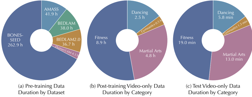
Figure A2: Dataset statistics. The charts show the duration of (a) each pre-training dataset, 383.8 hours in total, (b) each motion category in the video-only post-training data, 16.7 hours in total, and (c) each motion category in the held-out video-only test set, 39.1 minutes in total.
