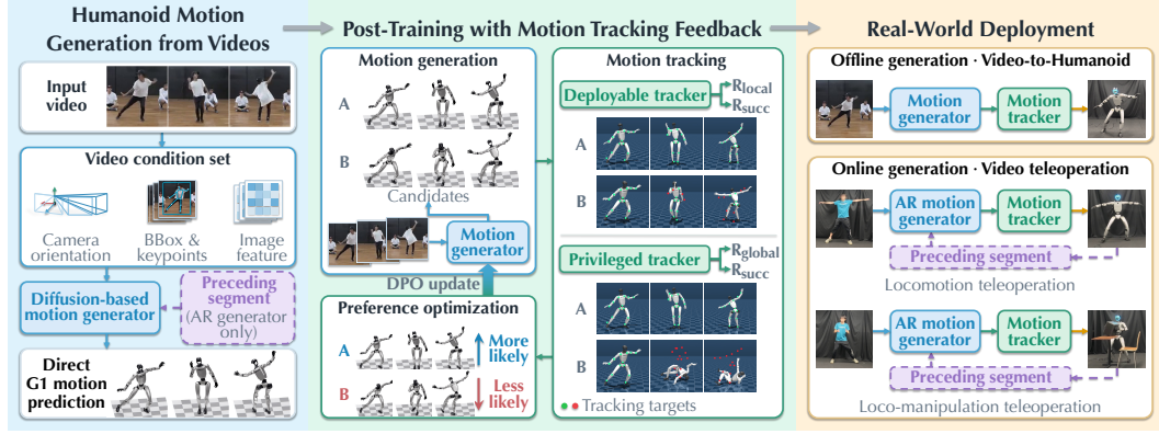
Figure 2: Overview of ViT-H. The diffusion-based generator (left) maps the camera orientations, bounding boxes, keypoints, and image features of a video directly to G1 reference motions, and its autoregressive variant also conditions on the preceding segment. For post-training (middle), candidates sampled for the same video are executed by a deployable tracker, which scores local pose accuracy and success, and by a privileged tracker, which scores global motion accuracy and success. At deployment (right), the offline generator drives video-to-humanoid control and the autoregressive generator drives real-time teleoperation.
