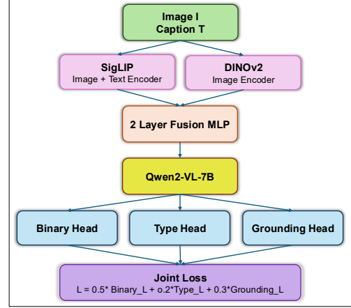
Figure 2. The three stage architecture of the MiD-VLM system.
