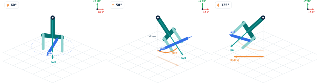
Figure 7: Slot yaw, tilt and tilt direction. The gripper orientation parameterization used by move_to (§3.1). Left: slot yaw \psi turns the jaw slot (blue), the axis a held object lies along, about the vertical. Middle: tilt \tau leans the tool axis (teal) away from straight down; 0^\circ is top-down and 90^\circ horizontal. Right: tilt direction \phi sets the compass direction the fingertips tip toward. Each angle changes exactly one thing about the gripper that can be seen. All angles are measured counterclockwise from world +x .
