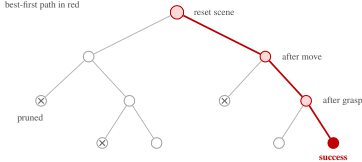
Figure 8: Prefix-tree search (§3.3). A node is created after each physical action (a move, grasp or release) settles. The search keeps returning to the most promising partial episode and branching from there, instead of starting every attempt from scratch; branches that keep failing are pruned. We allow up to about 1,000 leaves per task.
