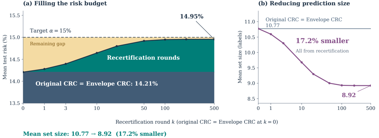
Figure 1: Risk-budget use and mean prediction-set size on CIFAR-100 with confidence-adaptive prediction rules ( n = 50 , \alpha = 0.15 ). Round 0 is CRC, and later rounds apply recertification. Results are averaged over 300 paired splits, each with 16 test images.
