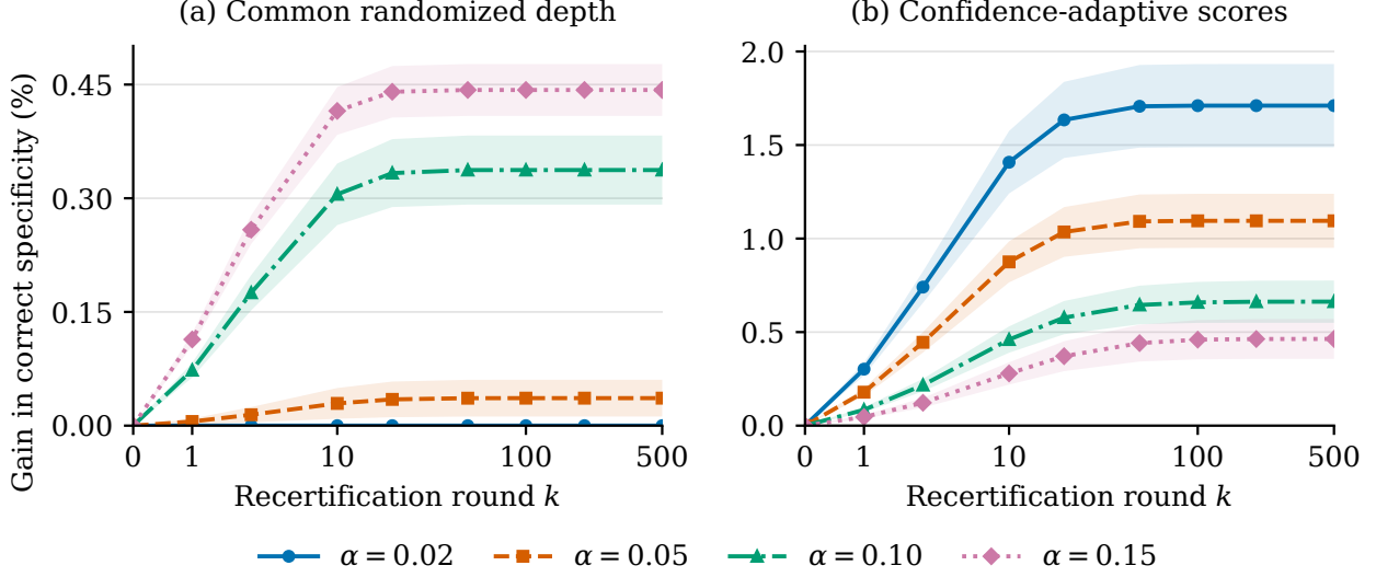
Figure 2: Gains in correct specificity of recertification beyond envelope CRC at n = 50 . Each panel shows mean paired gains over 300 splits, with shaded pointwise 95% Student- t intervals. The horizontal axis is logarithmic in k + 1 , where k is the number of rounds.
