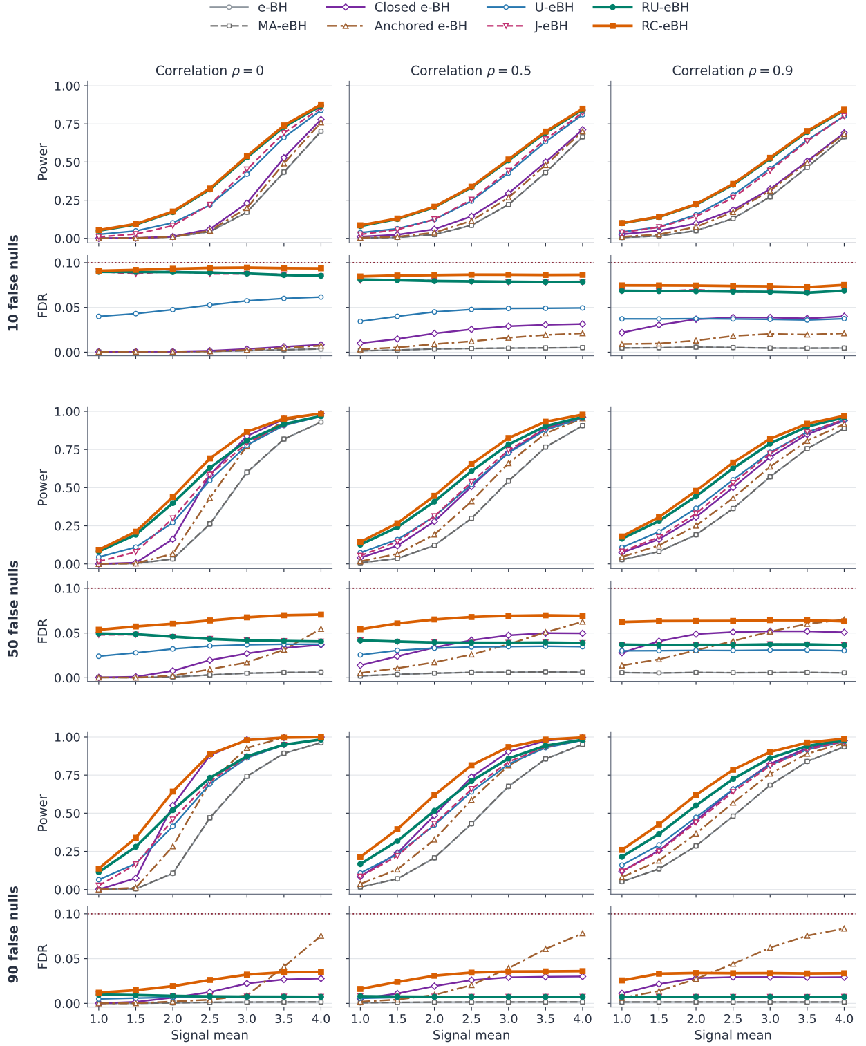
Figure 3: Power and FDR of RU-eBH, RC-eBH and six other procedures that are valid under arbitrary dependence, with 10, 50 and 90 false nulls among K = 100 hypotheses at \alpha = 0.1 and three levels of correlation (columns). Each point averages 50,000 data sets. The dotted lines mark \alpha .
