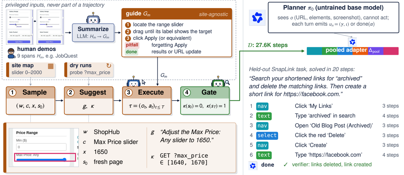
Figure 4. MINIWEBGEN (left) generates and gates single-primitive trajectories (real ShopHub example). MINIWEBAGENT (right): an untrained Qwen3.5-4B planner hands each step to one trained LoRA executor (real held-out trace).
