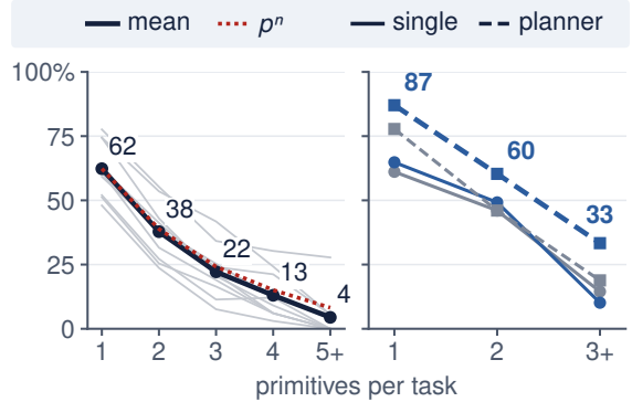
Figure 6. Failures compound along a task’s chain of primitives. Left: the ten untrained agents of Tab. 2 on all 369 tasks (grey), with p their mean success on one-primitive tasks. Right: Qwen3.5-4B untrained (grey) or trained (blue) on the 62 held-out tasks (Tab. 3).
