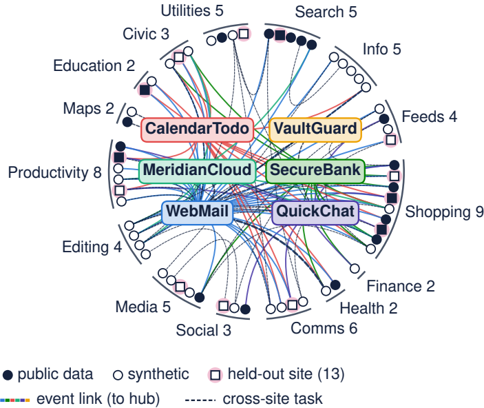
Figure 2. The 65 websites. Left: sites by domain (squares: held-out), linked to hubs at the center (colored edges) and by cross-site tasks (dashed). Right: the 65 MINIWEB sites, divided by data source.
