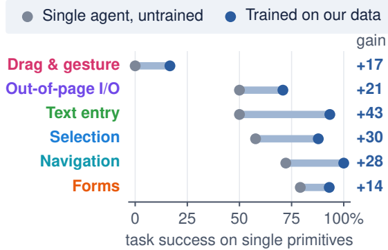
Figure 7. Practice lifts every skill family. Success per skill family on the 103 generated single-primitive tasks of the held-out sites, for a single Qwen3.5-4B agent untrained (grey) and trained on our data (blue), with the gain at the right; reasoning , which is not trained, is left out.
