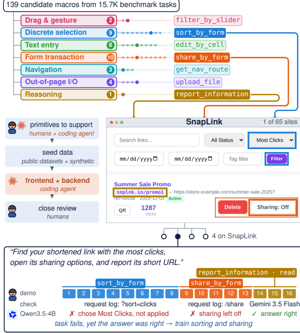
Figure 3. Building MINIWEB bottom up. (1) Tasks of existing benchmarks are mined into 37 primitives in 7 families. (2) Sites are built around their primitives. (3) Tasks chain primitives, with a verdict per primitive. Takeaway: every step of a task maps to one skill that can be graded.
