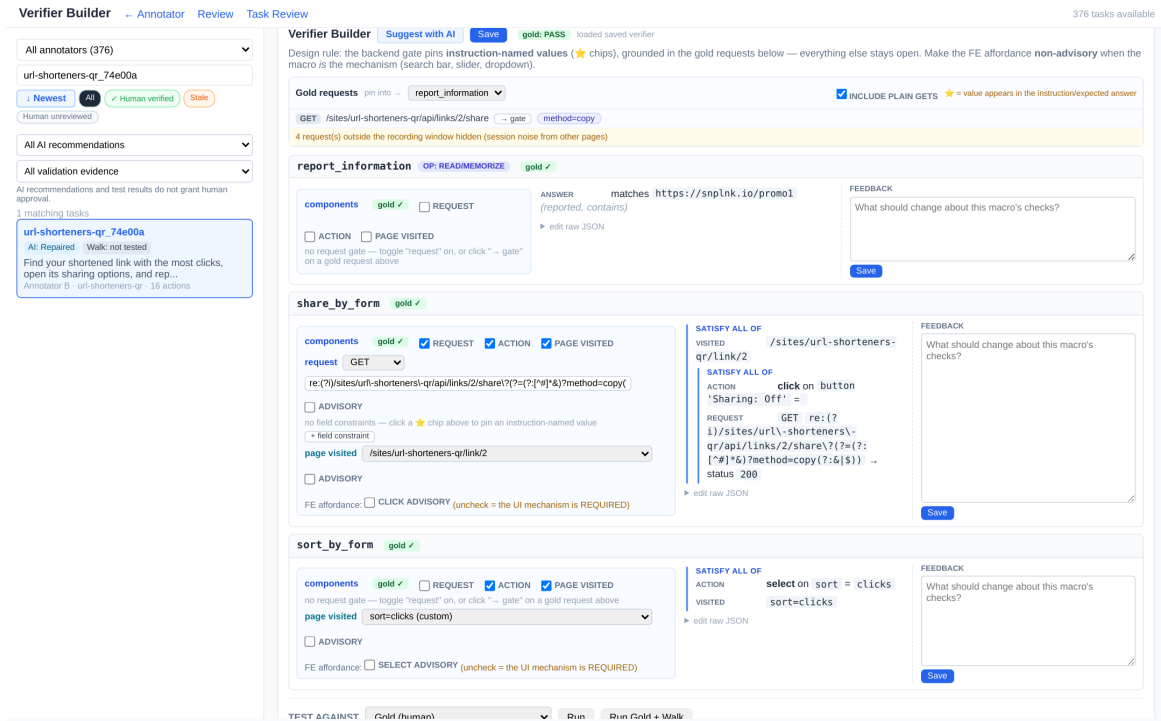
Figure 10. Verifier builder. Each primitive instance of the task gets its own check (request, action, page visited, answer), grounded in the gold requests of the recording; the sandbox below tests the verifier against the gold recording and negative controls.
