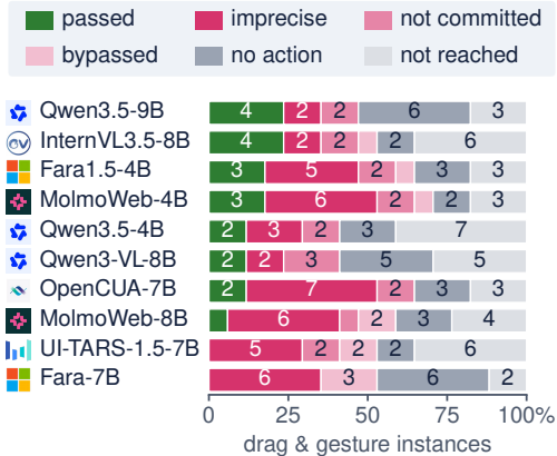
Figure 5. Most drag failures happen at the gesture itself. Outcomes of the ten untrained agents on every drag & gesture instance (11 slider and 6 signature tasks), from the VLM judge’s explanations; bypassed means, e.g., typing a name instead of drawing it.
