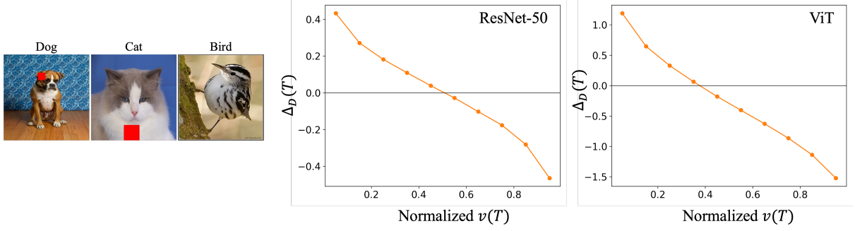
Figure 4: Controlled marker-bias experiment. Left: representative inputs. The marker is correlated with the dog class and can therefore mislead cat predictions. Middle and right: for both ResNet-50 and ViT-B/16, the marginal contribution \Delta_D(T) = v(T \cup D) - v(T) decreases with the strength of the non-marker context. The marker helps in weak contexts but suppresses the cat logit in strong contexts.
