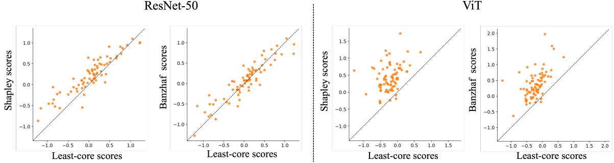
Figure 5: Per-image marker attribution for ResNet-50 (left) and ViT-B/16 (right). We compare the Shapley and Banzhaf ( p = 0.5 ) scores with the corresponding least-core scores. Each point represents one retained image, and the dashed line indicates equal attribution; points above the line receive more attribution from the semivalue than from the least-core.
