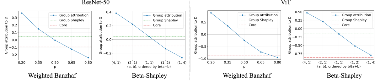
Figure 6: Effect of context-size weighting on the group attribution to the marker region D . The left two panels show ResNet-50 and the right two show ViT-B/16. Within each pair, the first panel varies p for the weighted-Banzhaf family, and the second shifts the Beta-Shapley parameters from small-context weighting (4, 1) to large-context weighting (1, 4) . The solid blue curves show the group semivalue obtained at each parameter setting. The dotted green and dashed red lines show the independently estimated group Shapley baseline and the least-core attribution, respectively.
