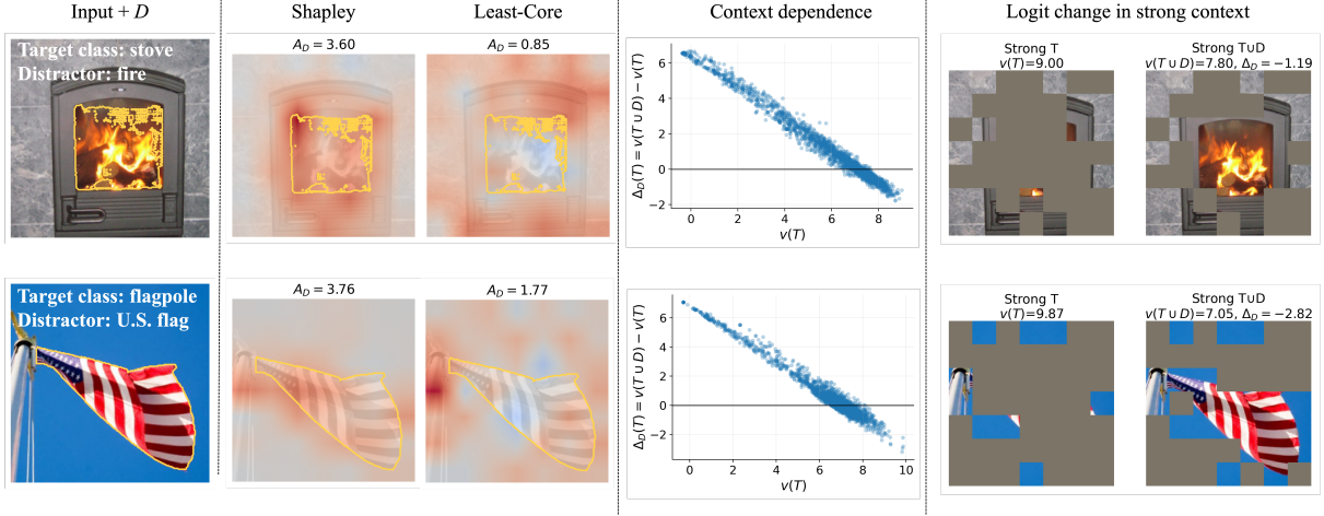
Figure 3: Representative examples of contextual distractors. Input + D : the original input, with the distractor region D outlined in yellow. Shapley and Least-Core : patch-attribution heatmaps, where red and blue indicate positive and negative attribution, respectively; A_D gives the total attribution assigned to the patches in D . Context dependence : the marginal contribution \Delta_D(T) = v(T \cup D) - v(T) plotted against the target-class logit v(T) obtained from the surrounding context T . Logit change in strong context : a sampled strong coalition T before and after adding D , reporting the resulting target-class logit v(T \cup D) and its change \Delta_D from v(T) .
