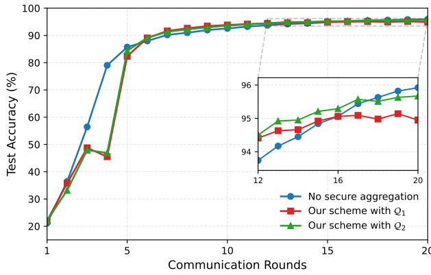
Fig. 1. Test accuracy versus communication rounds on MNIST dataset with our secure aggregation protocol, under distinct quantization settings Q_1 and Q_2 , against FedAvg.
