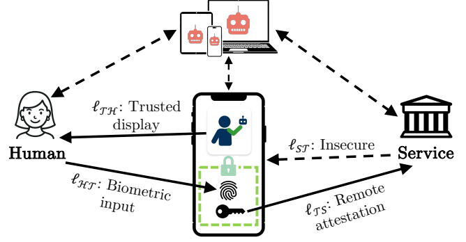
Figure 6: The Countersign topology. A user’s mobile phone serves as \mathcal{T} and establishes channels to \mathcal{H} and \mathcal{S} . Channels are labeled with the mechanism they use to establish authenticity. On the phone, the green lock represents that the enclosed functionalities are run by on-device secure hardware, the application itself is run by the OS.
