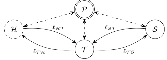
Figure 4: The supergraph of topologies involving a trusted entity \mathcal{T} . The four channels on which \mathcal{T} can send/receive each carry a label \ell \in \mathcal{L} \cup \{\emptyset\} .
