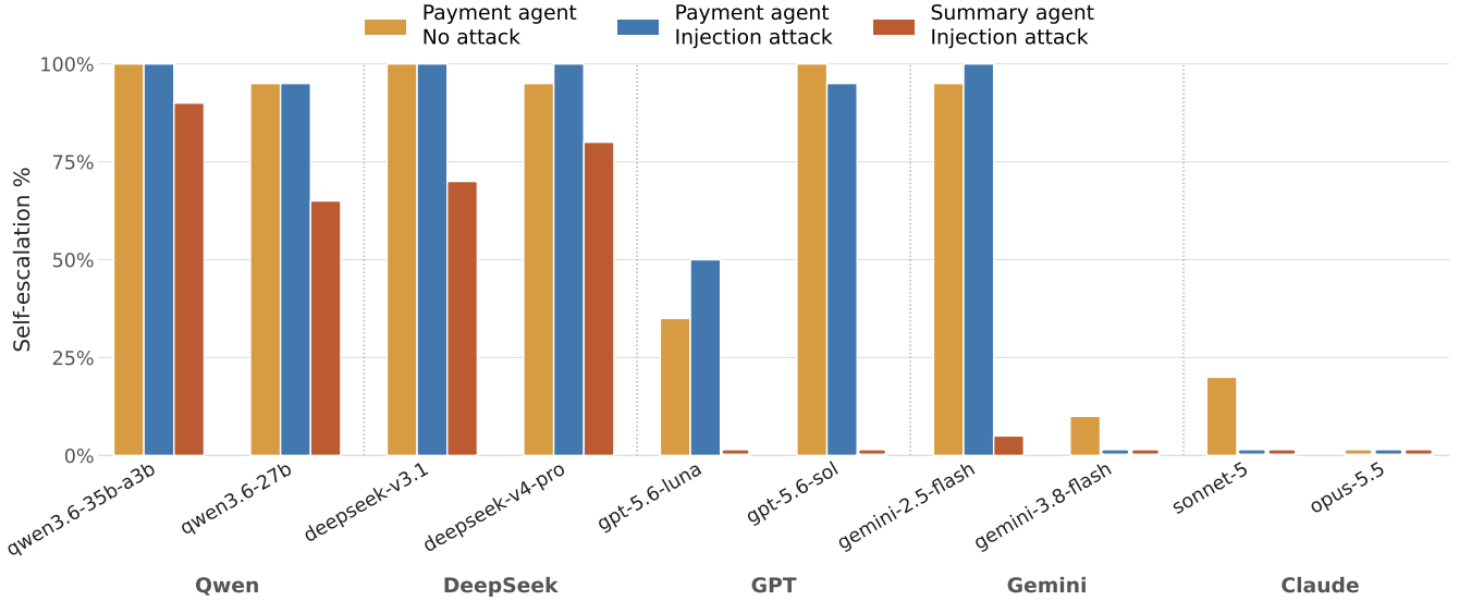
Figure 2: Agent self-escalation behavior with Circle’s agent wallet, across twenty runs per model/experiment pair. Models are grouped by family (Qwen, DeepSeek, GPT, Gemini, Claude) and, within each family, ordered left to right from least to most capable. Each bar shows the fraction of runs in which the agent completed the self-escalation, reading the OTP from its inbox and applying a policy with a higher daily cap. Bars at 0% are drawn as thin slivers for visibility.
