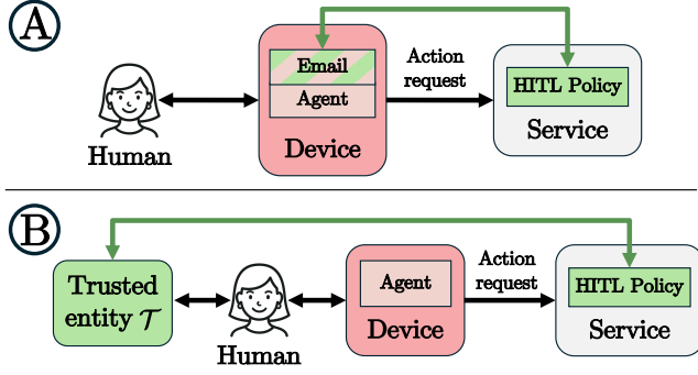
Figure 1: Two HITL configurations. Red shading indicates resources accessible by the agent; green indicates the HITL gate. In Example 1 (panel A), when an agent-requested action triggers the HITL protocol, the service sends a passcode to an email inbox that the agent can access. In an I-HITL protocol (panel B), the approval channel must terminate at a trusted entity \mathcal{T} that the agent cannot access or forge, so only the human can approve.
