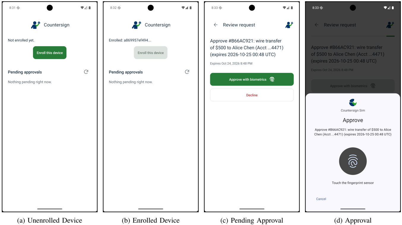
Figure 12: The Countersign Android application.
