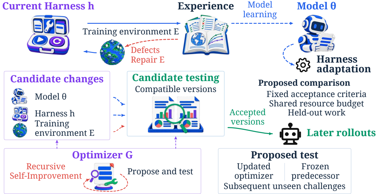
Figure 7 Model-harness coupling and improvement across training executions. The current harness shapes experience used to train the model; model updates can motivate harness adaptation. Evidence informs candidate changes to executor weights \theta , harness h , or training environment E . Optimizer G proposes and tests changes, and accepted versions supply subsequent rollouts. The paths illustrate possible component updates, without prescribing their order or requiring every target to change. A separate relation denotes recursive self-improvement of G ’s search and diagnostic/testing procedures. Fixed acceptance criteria, held-out work, and a shared resource budget are our proposed comparison conditions. We further propose comparing the updated optimizer with its frozen predecessor on subsequent unseen challenges.
