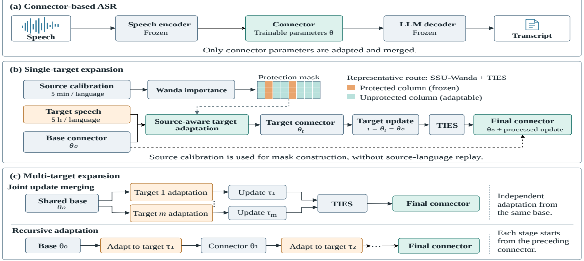
Figure 1: Overview of source-aware multilingual ASR expansion.
