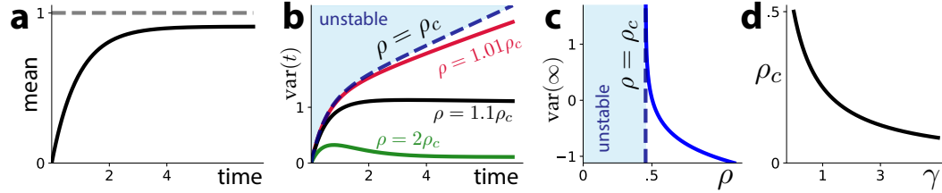
Figure 2: Instability in a linear model. (a) Average dynamics are unconditionally stable and do not depend on the arrival rate \rho . (b) Output variance converges more slowly as \rho decreases and diverges to infinity when \rho < \rho_c . (c) The steady state output variance diverges like 1/(\rho - \rho_c) . (d) \rho_c decreases as \gamma increases, so one way to improve stability is to increase the regularization strength.
