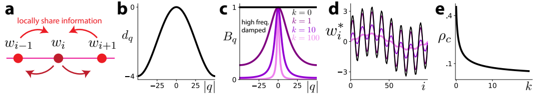
Figure 5: Pooling parameters can improve stability. (a) If nearby synapses store similar information, neurons may benefit from sharing information with their spatial neighbors. Pictured is a line of synaptic weights; arrows indicate bidirectional information sharing. (b) The eigenvalues d_q of \mathbf{D} are indexed by spatial frequencies |q| , and d_q decreases as |q| increases. (c) The q -dependence of d_q causes higher spatial frequencies of the fixed point to be damped, and the effect size increases as the amount of diffusion k increases (more purple \rightarrow higher k ). (d) One effect of this frequency-dependence is to smooth the fixed point of the average dynamics. In the pictured example, w_i^* is highly oscillatory (black), but dynamics converge to a smoothed version of it (shades of purple). (e) \rho_c decreases as k increases, so although parameter-pooling produces bias, it also improves stability.
