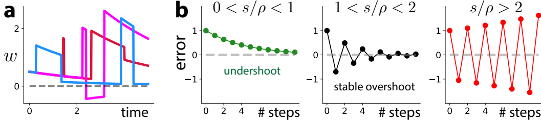
Figure 1: Sparse gradient arrivals: motivation and intuition. (a) A simple example of sparse gradient arrivals: a weight receives intermittent updates, in between which the regularization term produces relaxation toward zero. Three example stochastic simulations are shown. (b) Error as a function of number of arrivals in a toy model. If s/\rho < 1 , error always decreases (left); if 1 < s/\rho < 2 , error alternates in sign but decreases in magnitude (center); and if s/\rho > 2 , learning becomes unstable, and error both alternates in sign and increases in magnitude (right).
