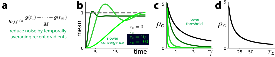
Figure 6: Averaging over gradient arrivals can improve stability. (a) Intuitively, one can reduce variance by performing a temporal average over recent gradient arrivals. (b) Mean dynamics are linear but not monotonic. As the gradient-averaging time scale \tau_z increases, they converge more slowly. (black: \tau_z = 0 ; lightest green: \tau_z = 100 ) (c, d) Increasing \tau_z improves stability since \rho_c decreases as long as \gamma > 0 . But if \gamma = 0 , there is no stability benefit.
