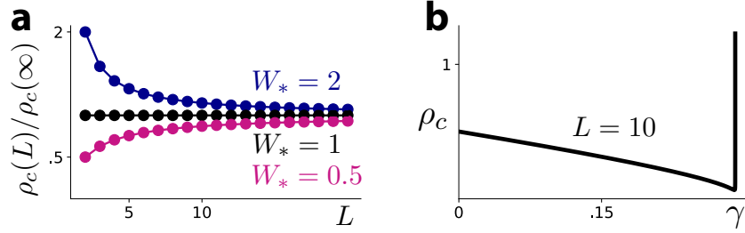
Figure 4: Depth benignly modulates stability in a deep linear network. (a) \rho_c can increase, decrease, or remain constant with L depending on the value of the target W_* . In all cases, the difference between \rho_c(L) and its asymptotic value \rho_c(\infty) is not substantial. (b) \rho_c is non-monotonic as a function of \gamma ( L = 10 shown), but this is mainly because sufficiently high regularization destabilizes the nontrivial fixed point.
